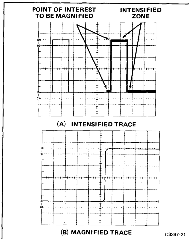
Figure 4-10. Delayed-sweep magnification.
