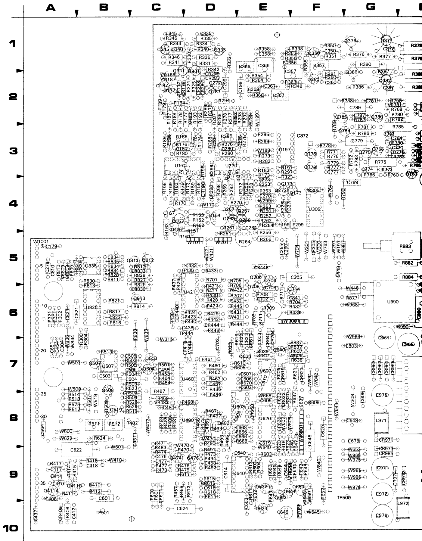
Fig. 9-9. A10—Main board (SN B020099 &amp; below)
