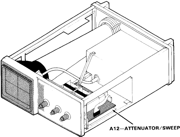
Figure 9-5. A12—Attenuator/Sweep board.
