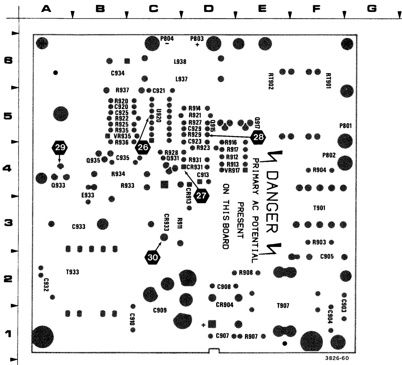
Figure 9-13. Circuit view of A18—Preregulator board.
