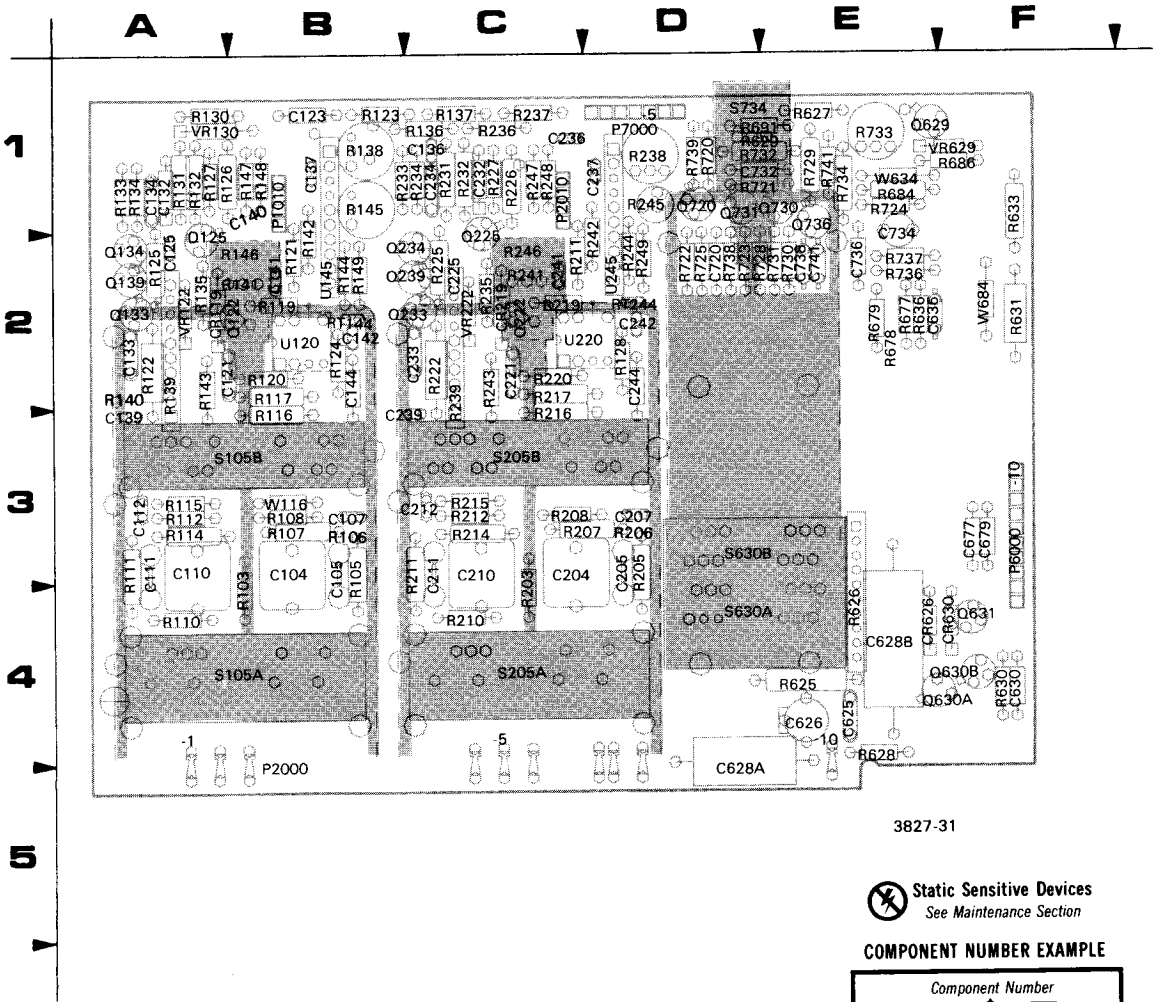
Figure 9-5. A12—Attenuator/Sweep board.
