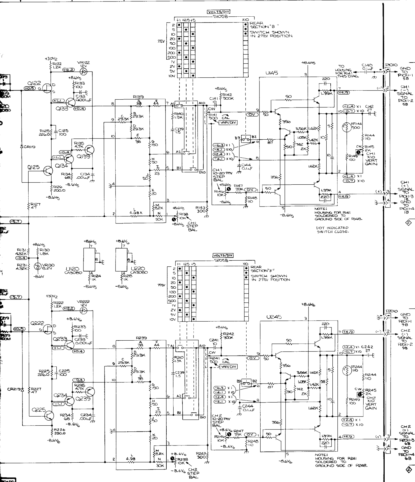
CH1 &amp; CH2 ATTENUATORS
