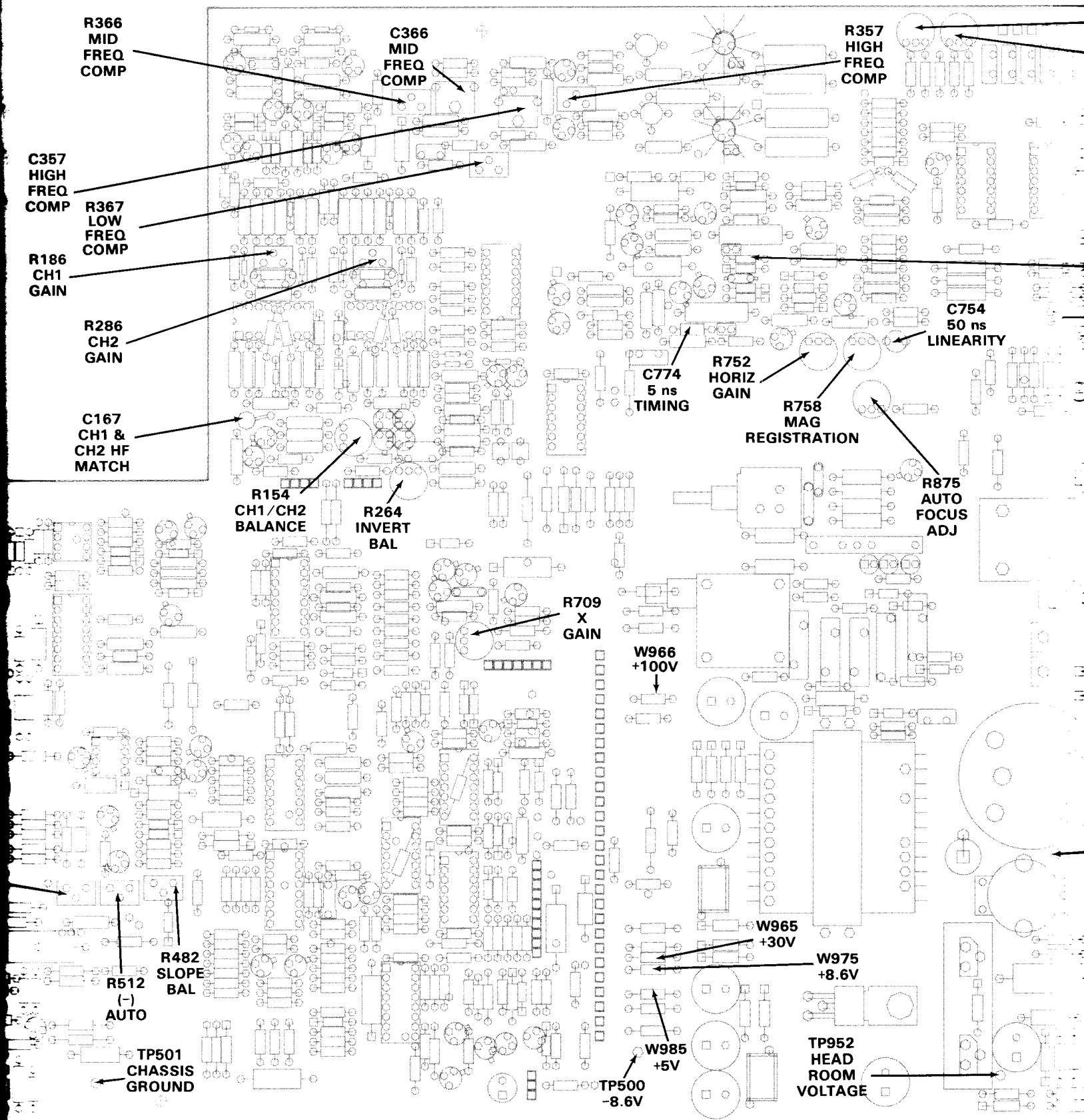
A10—MAIN BOARD ADJUSTMENT LOCATIONS
