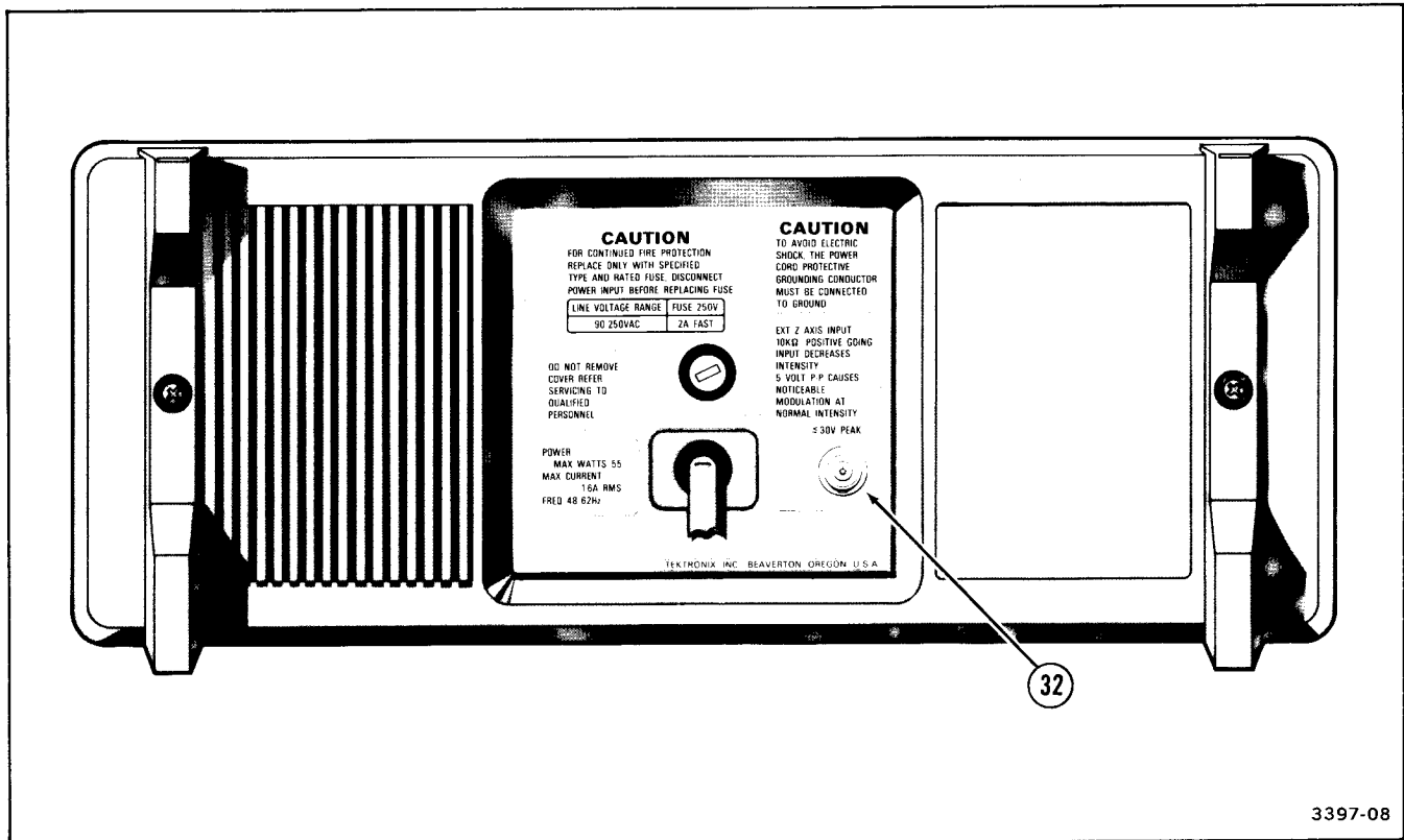
Figure 2-7. Rear-panel connector.
