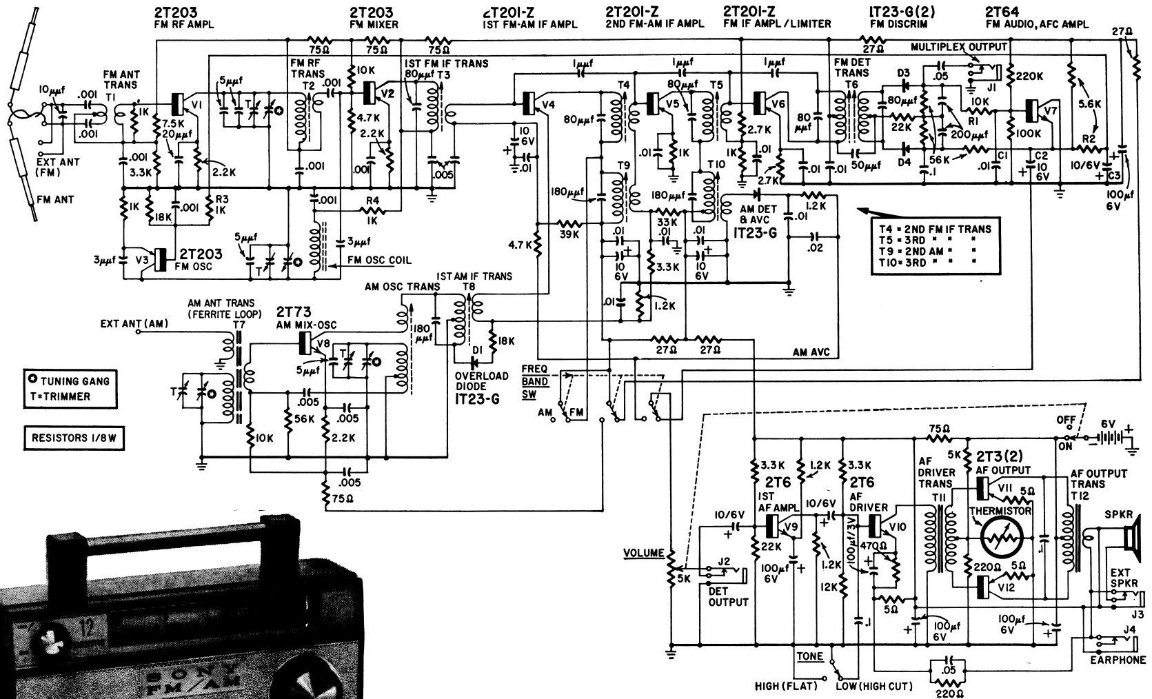
Circuit of the 12-transistor Sony TFM-121.
