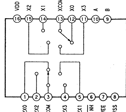
IC806, 807 MC14052BCP
