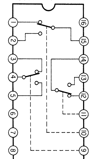
IC506 MC14053BCP
