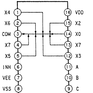
IC510 MC14051BCP
