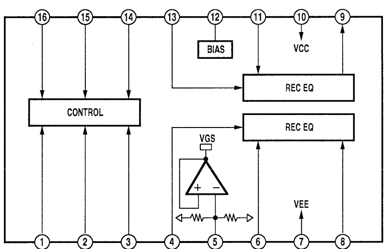
IC505 CXA1578P
