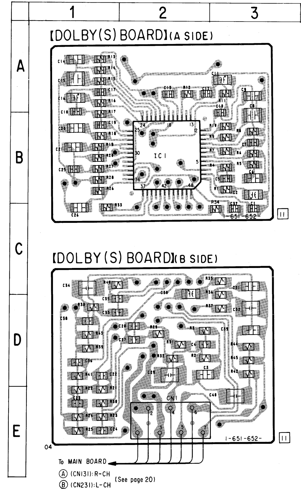
5-6. PRINTED WIRING BOARDS (DOLBY (S) SECTION) ● Refer to page 18 for Note. ● Refer to page 16 for Semiconductor Lead Layouts.
