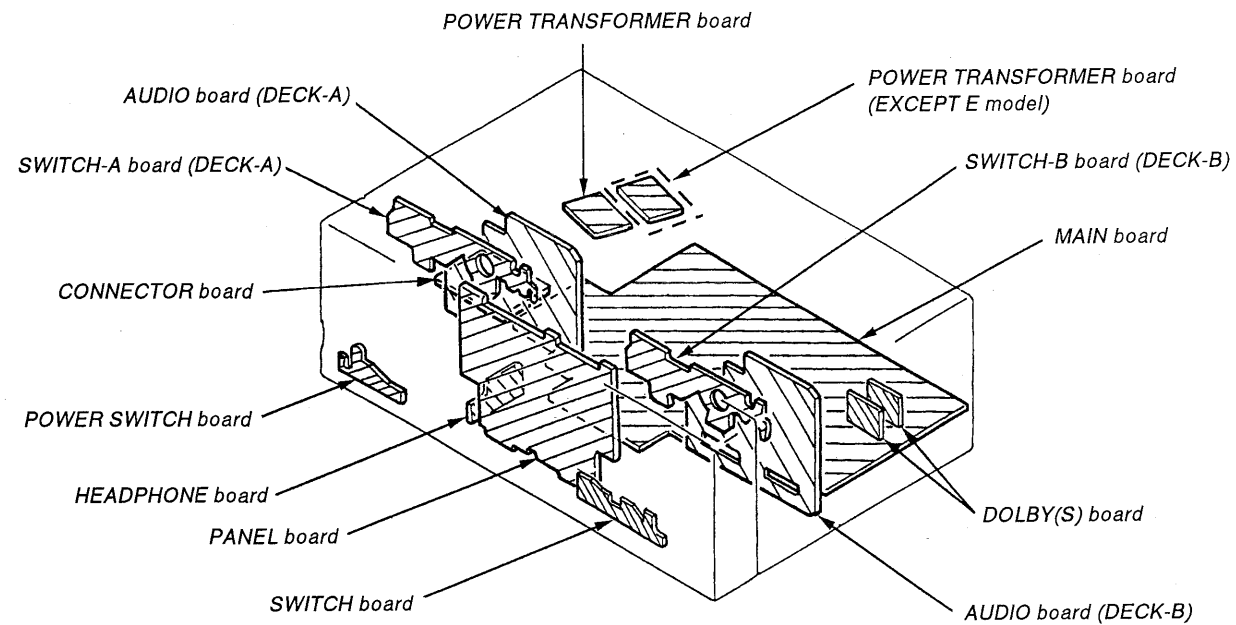
5-2. CIRCUIT BOARD LOCATION
