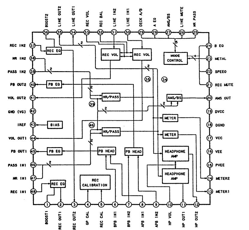
IC502 CXA1599Q
