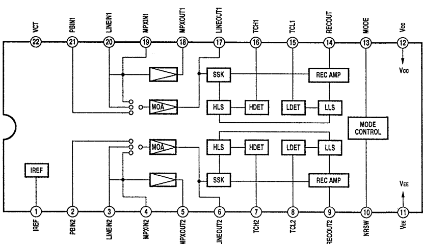
IC501 CXA1561S
