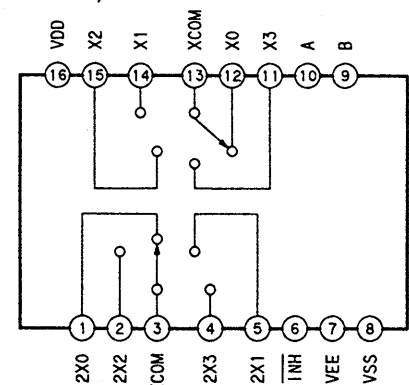
IC806, 807 MC14052BCP
