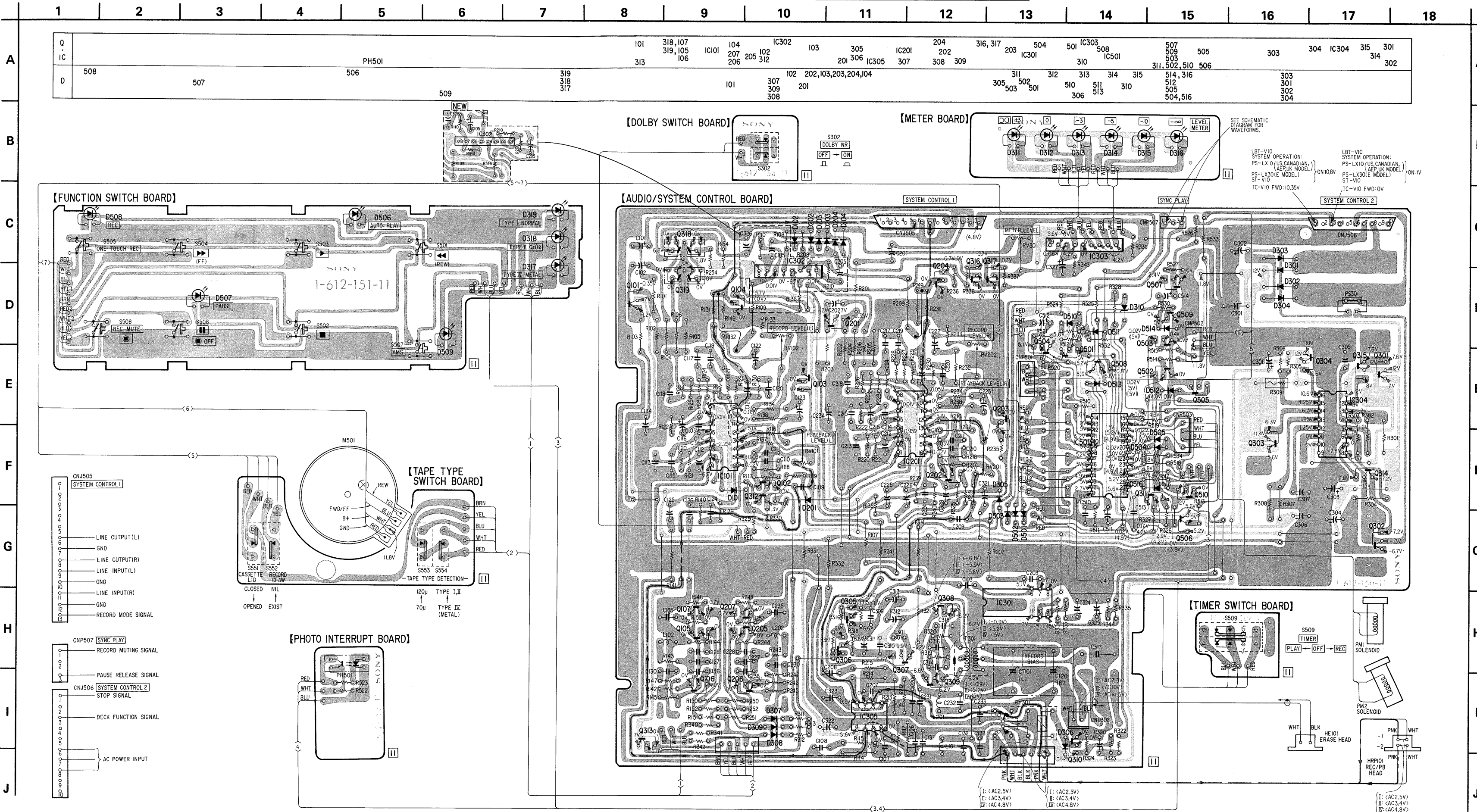
4-1. MOUNTING DIAGRAM
