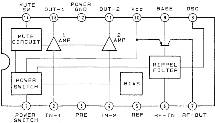
IC102 LA4538M
