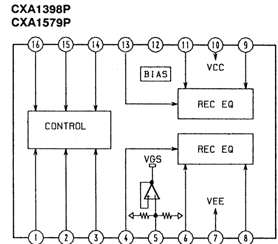
• IC BLOCK DIAGRAM
