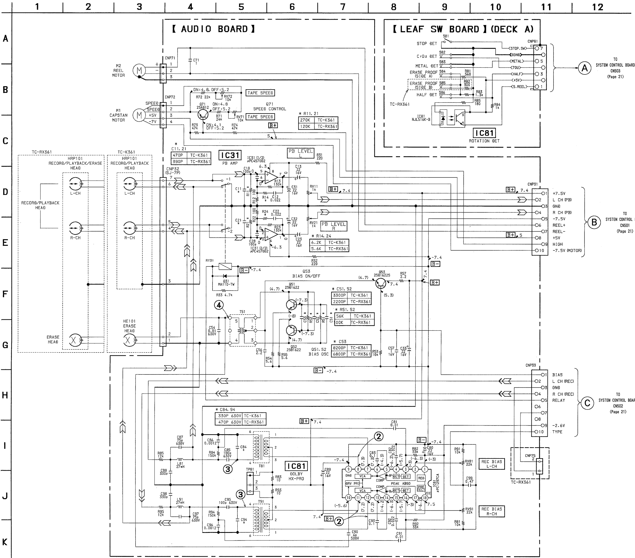
5-5. SCHEMATIC DIAGRAM (AUDIO SECTION)
