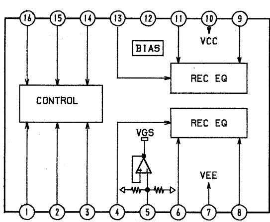
● IC Block Diagram IC502 CXA1579P
