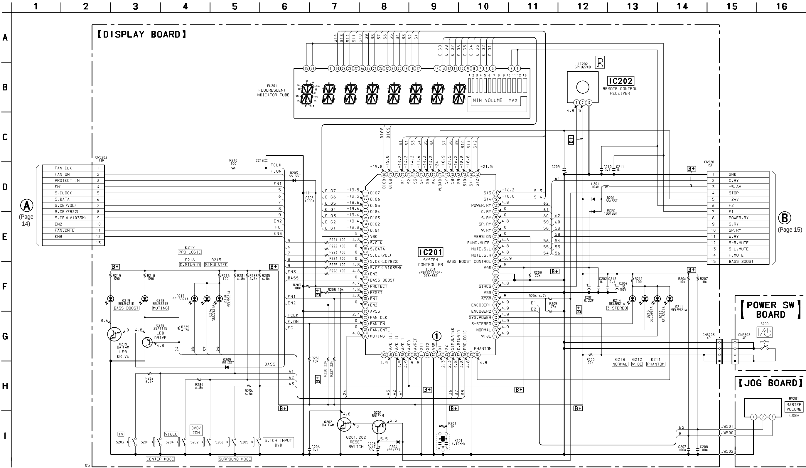
4-6. SCHEMATIC DIAGRAM – PANEL Section – • See page 8 for Waveform.
