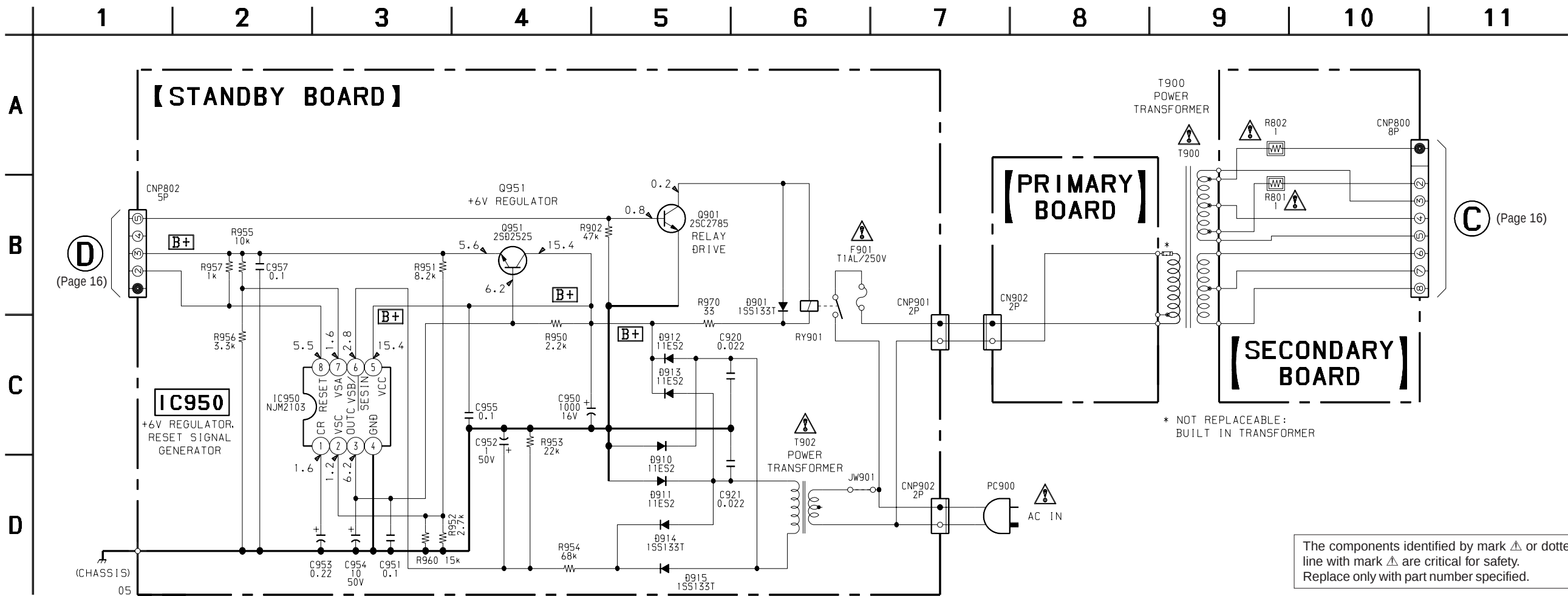
4-8. SCHEMATIC DIAGRAM – POWER Section – • See page 9 for IC Block Diagram.
