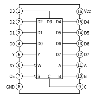
IC3313 TC74HC151AF-TP1 (DIGITAL BOARD)
