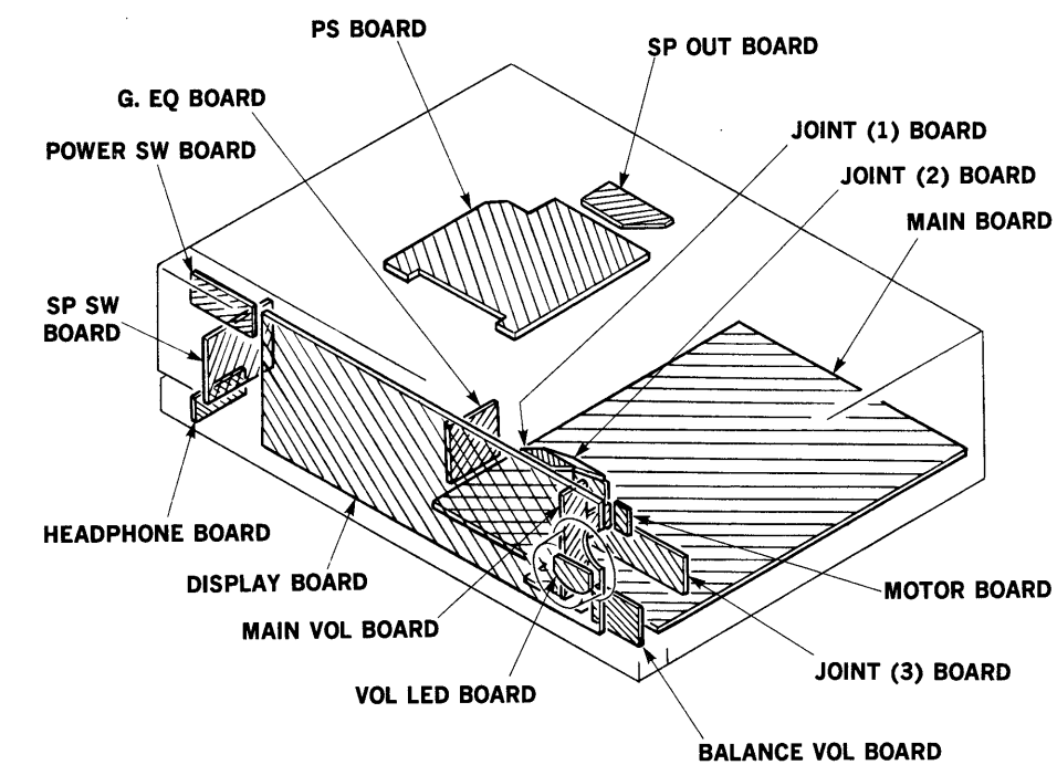
4-2. CIRCUIT BOARDS LOCATION
