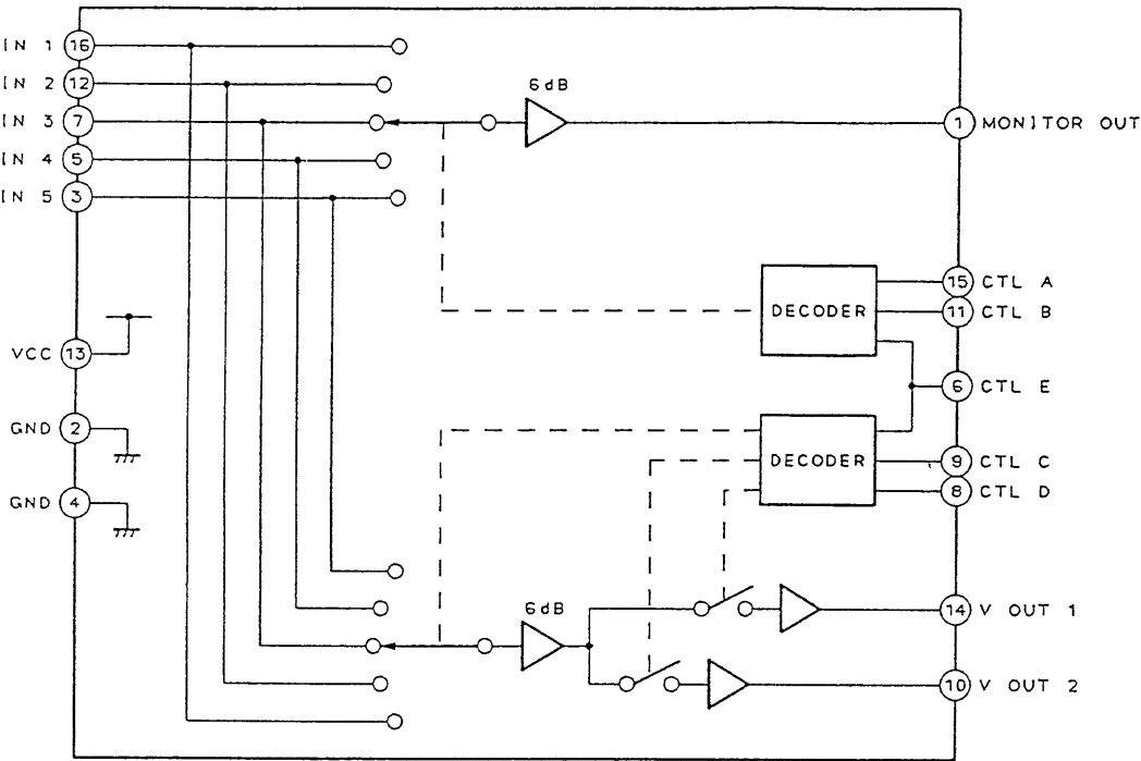
IC201, 251, 252 SN761200
