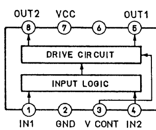
IC654 LB1639
