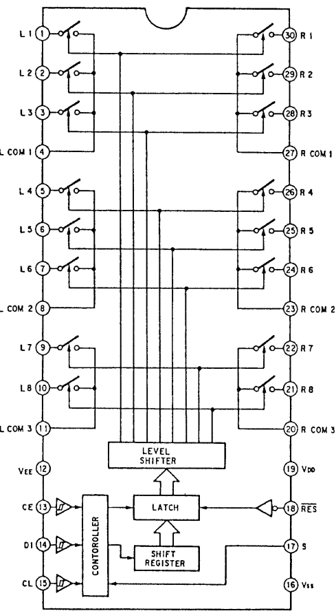
IC104, 105 LC7822
