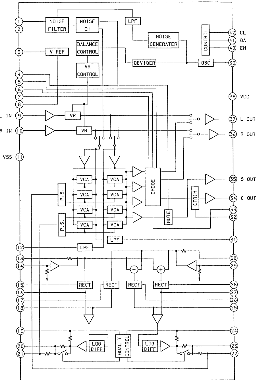
IC301 LA2785
