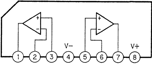
IC102 M5218AL
