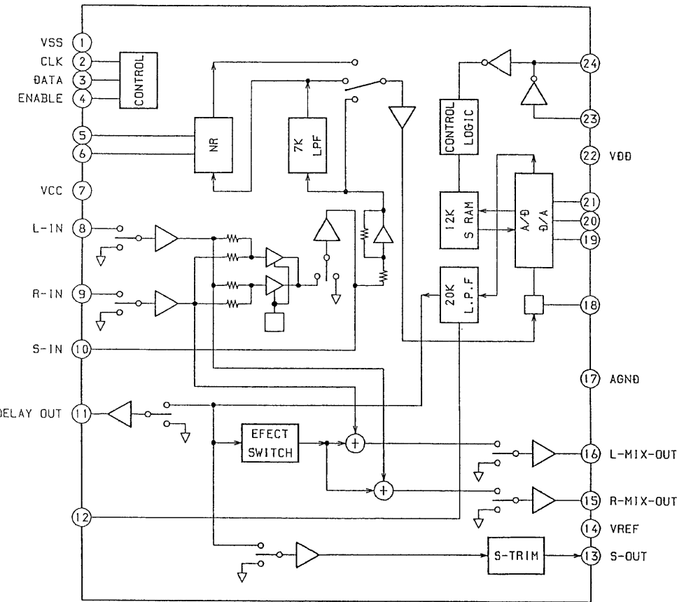
IC302 LV1011
