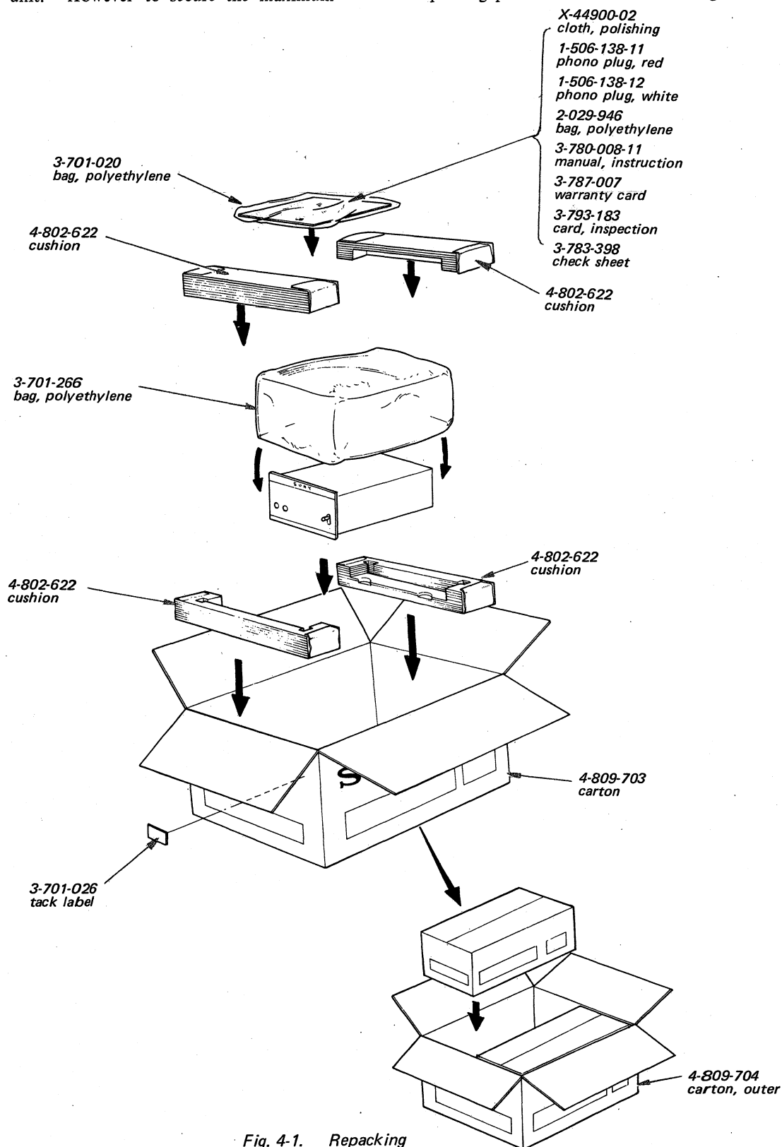
Fig. 4-1. Repacking
