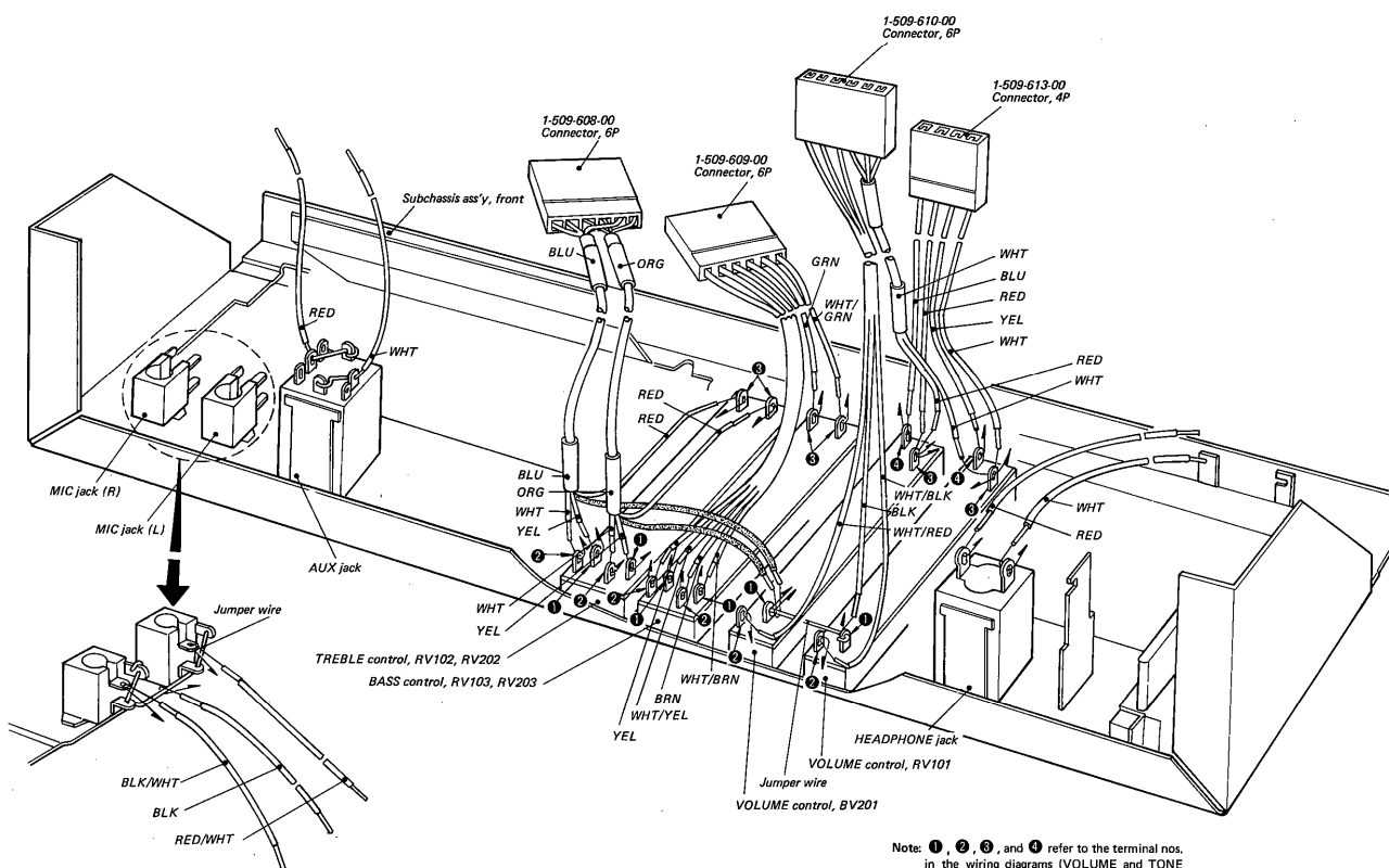
2-1. Front Subchassis Wiring Diagram
