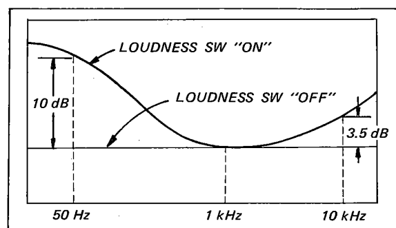
Fig. 1-3. Loudness circuit response
