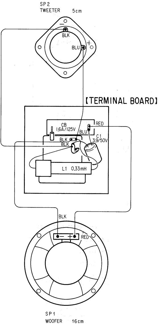
WIRING DIAGRAM
