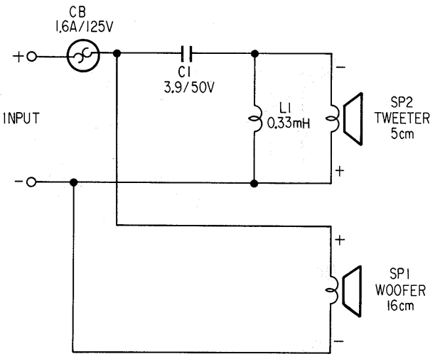
SCHEMATIC DIAGRAM
