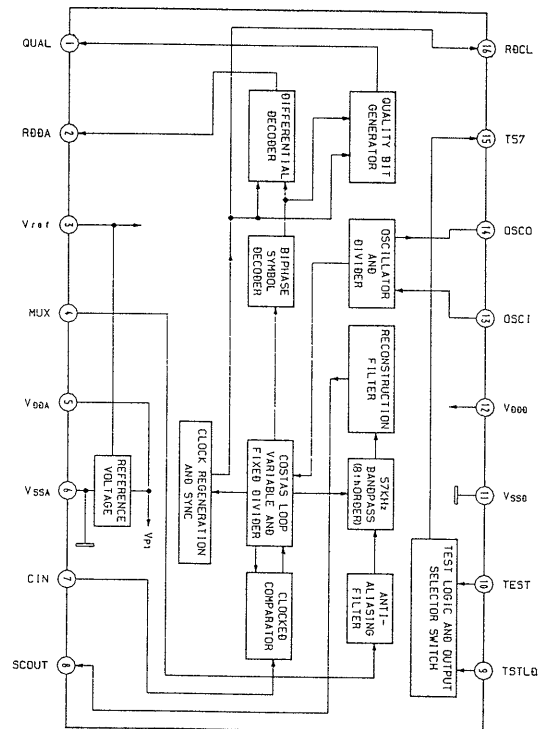
IC801 SAA6579T
