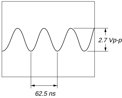
2 IC501 13 (XOUT)
