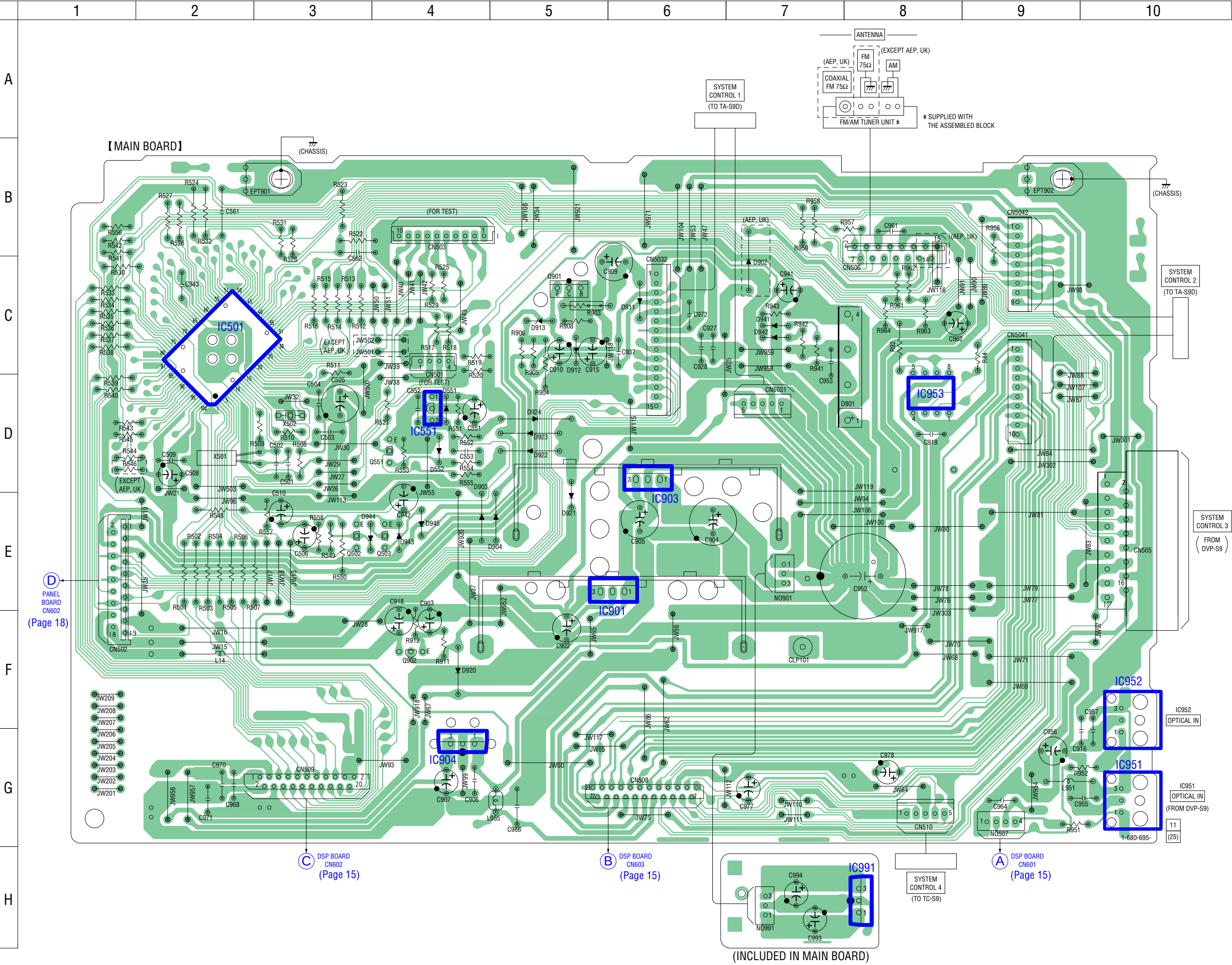
5-4. PRINTED WIRING BOARD – MAIN Board – • See page 10 for Circuit Boards Location.
