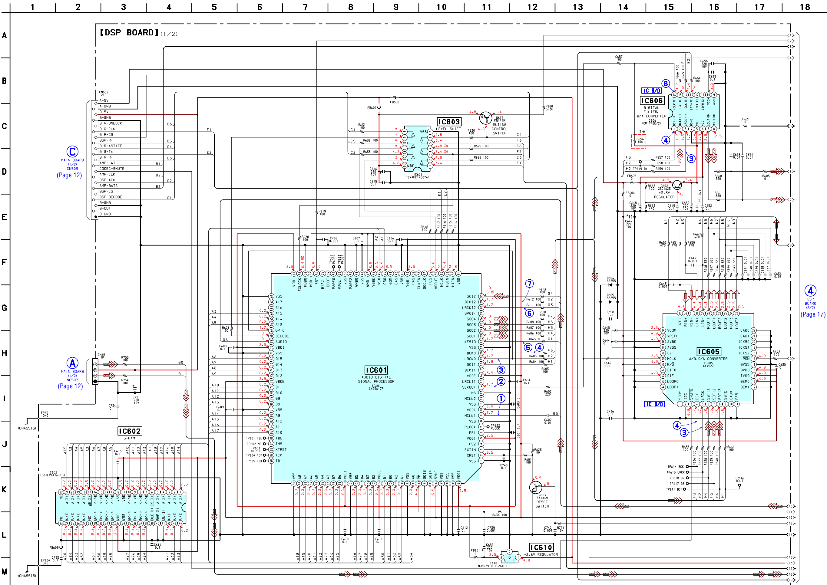
5-6. SCHEMATIC DIAGRAM – DSP Board (1/2) – • See page 11 for Waveforms. • See page 11 for IC Block Diagrams.
