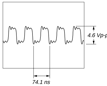
2 IC601 14 (SCKOUT)
