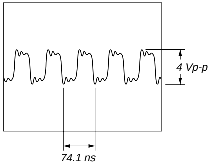
2 IC601 14 (SCKOUT)
