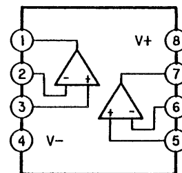
IC252, 302 M5218AP
