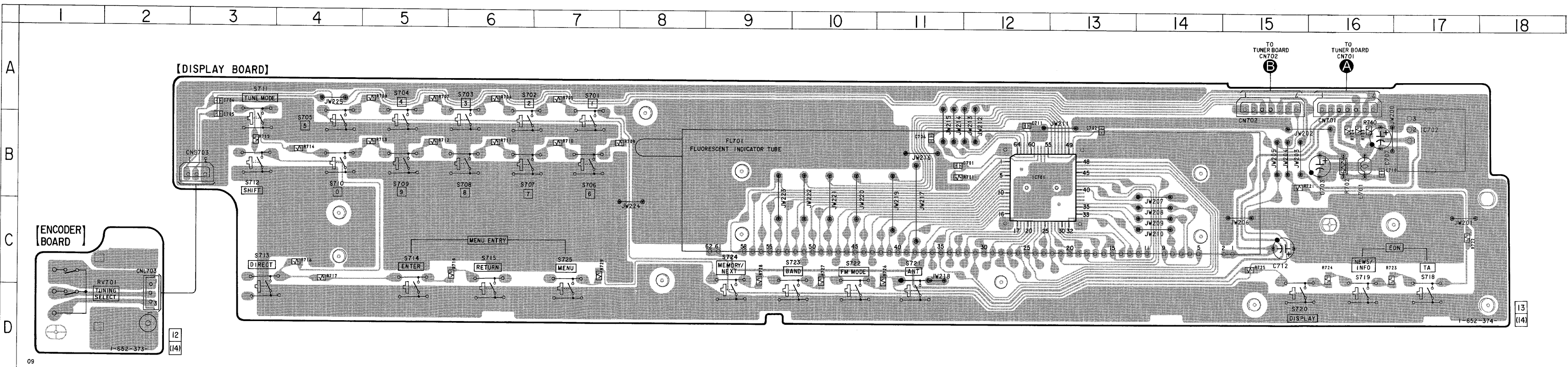
4-4. PRINTED WIRING BOARD — DISPLAY SECTION —
