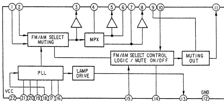
IC301 LA3401
