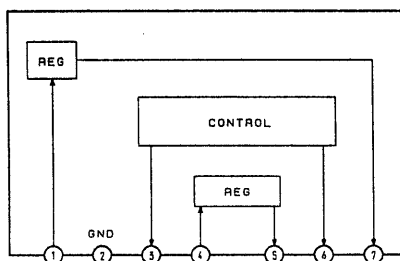
IC501 LA5667
