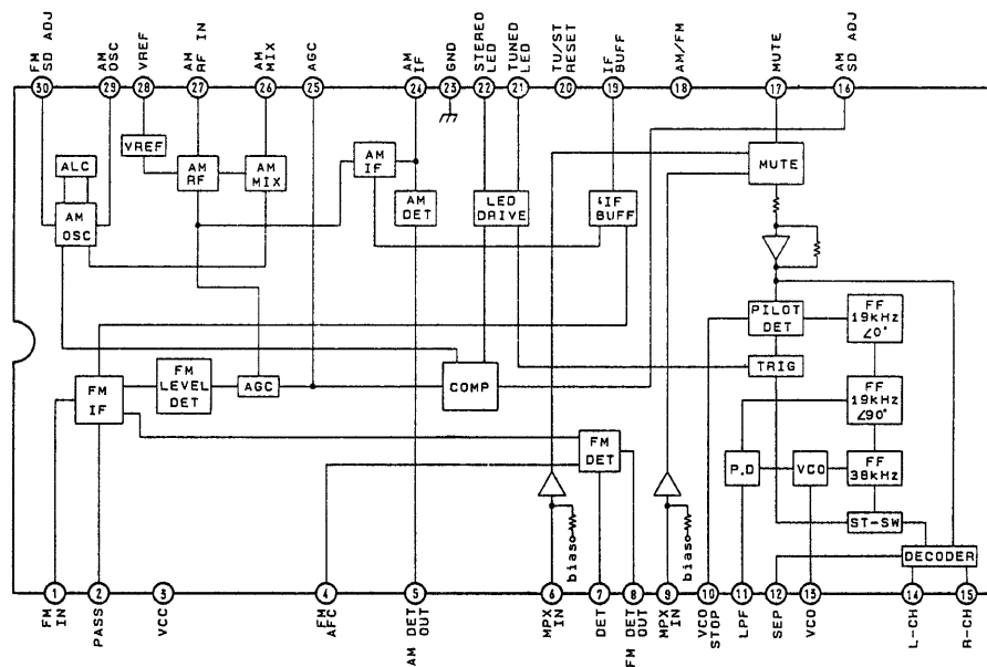
IC21 LA1851N
