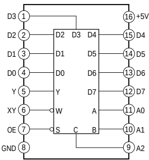
IC1313 TC74HC151AF (DIG-IN/OUT BOARD)
