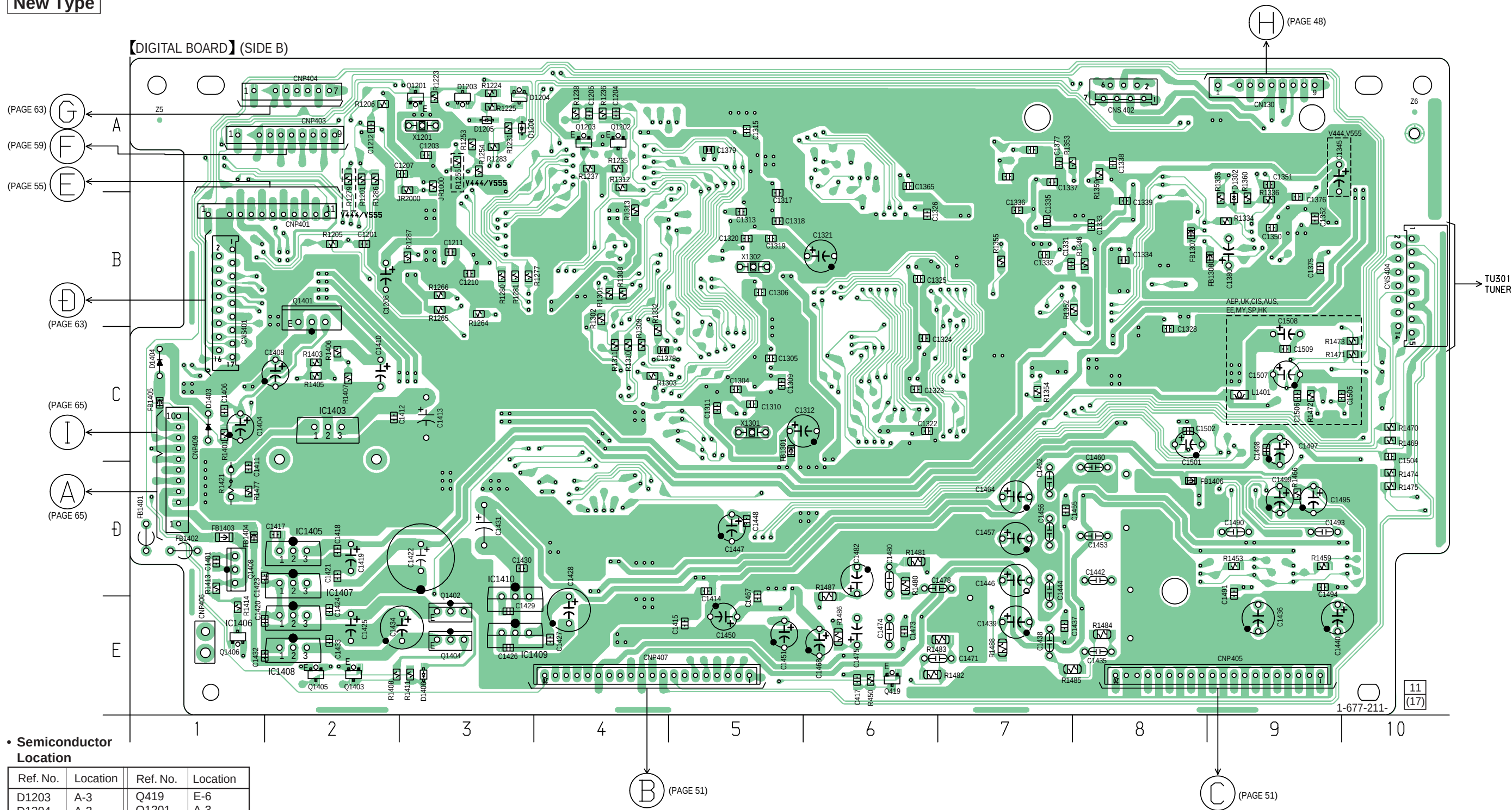
5-34. PRINTED WIRING BOARD — DIGITAL (SIDE B) SECTION — • See page 17 for Circuit Boards Location.
