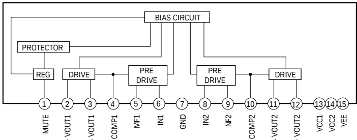
IC303, 306 TC9273F (INPUT BOARD)
