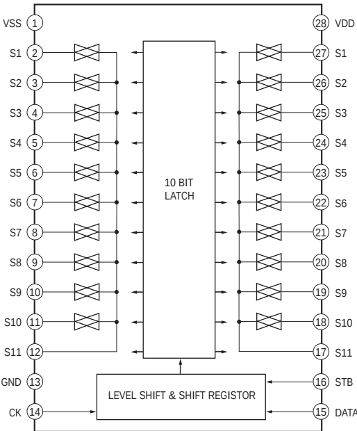
IC303, 306 TC9273F (INPUT BOARD)
