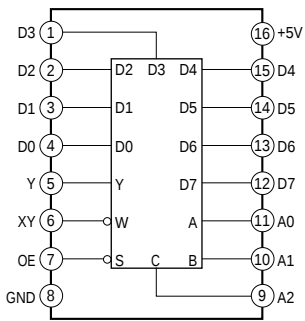
IC1313 TC74HC151AF (DIG-IN/OUT BOARD)
