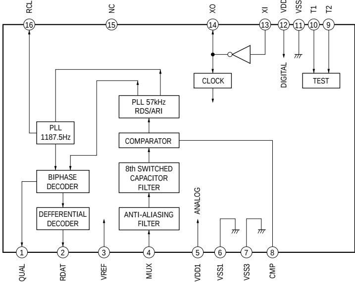
IC1420 BU1924F-E2 (DIGITAL BOARD)
