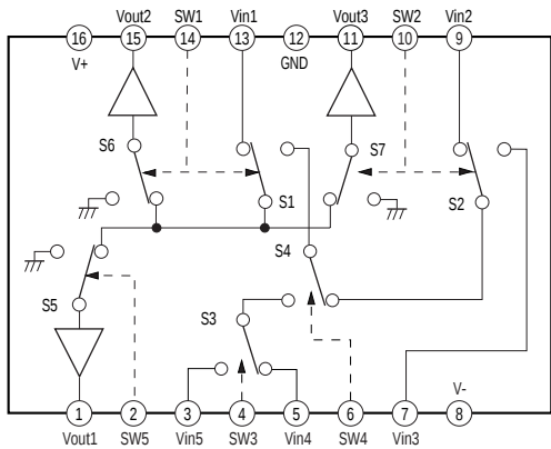
IC201, 211 NJM2296M-TE2 (C-VIDEO BOARD) IC202, 203 NJM2296M-TE2 (S-VIDEO BOARD)
