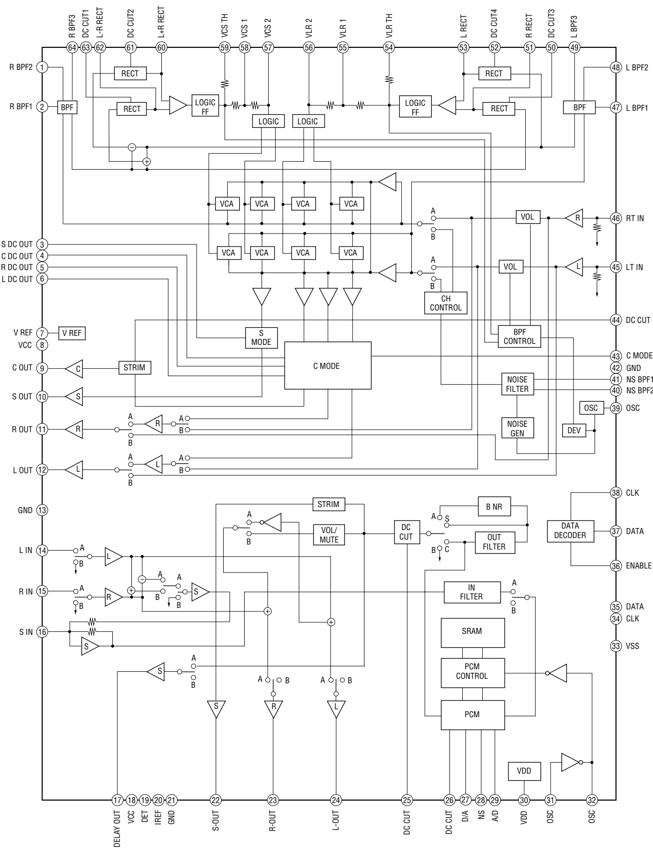
IC301 LV1035M
