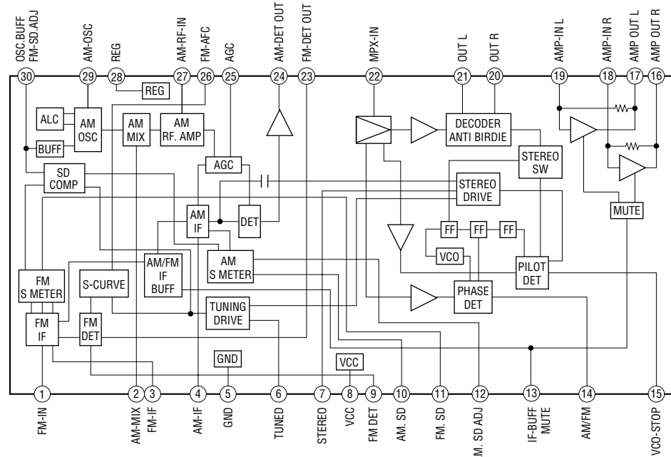
IC501 LA1838
