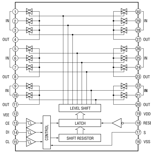
IC401 LC7822
