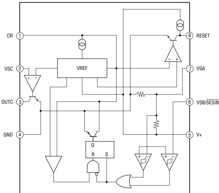
IC950 NJM2103D
