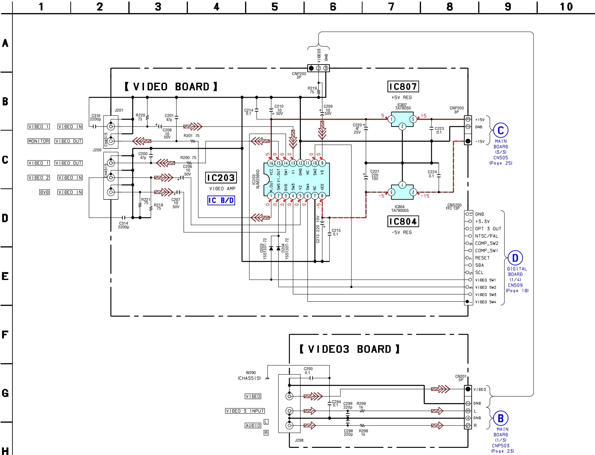
3-19. SCHEMATIC DIAGRAM – VIDEO IN/OUT SECTION – • See page 37 for IC Block Diagram.
