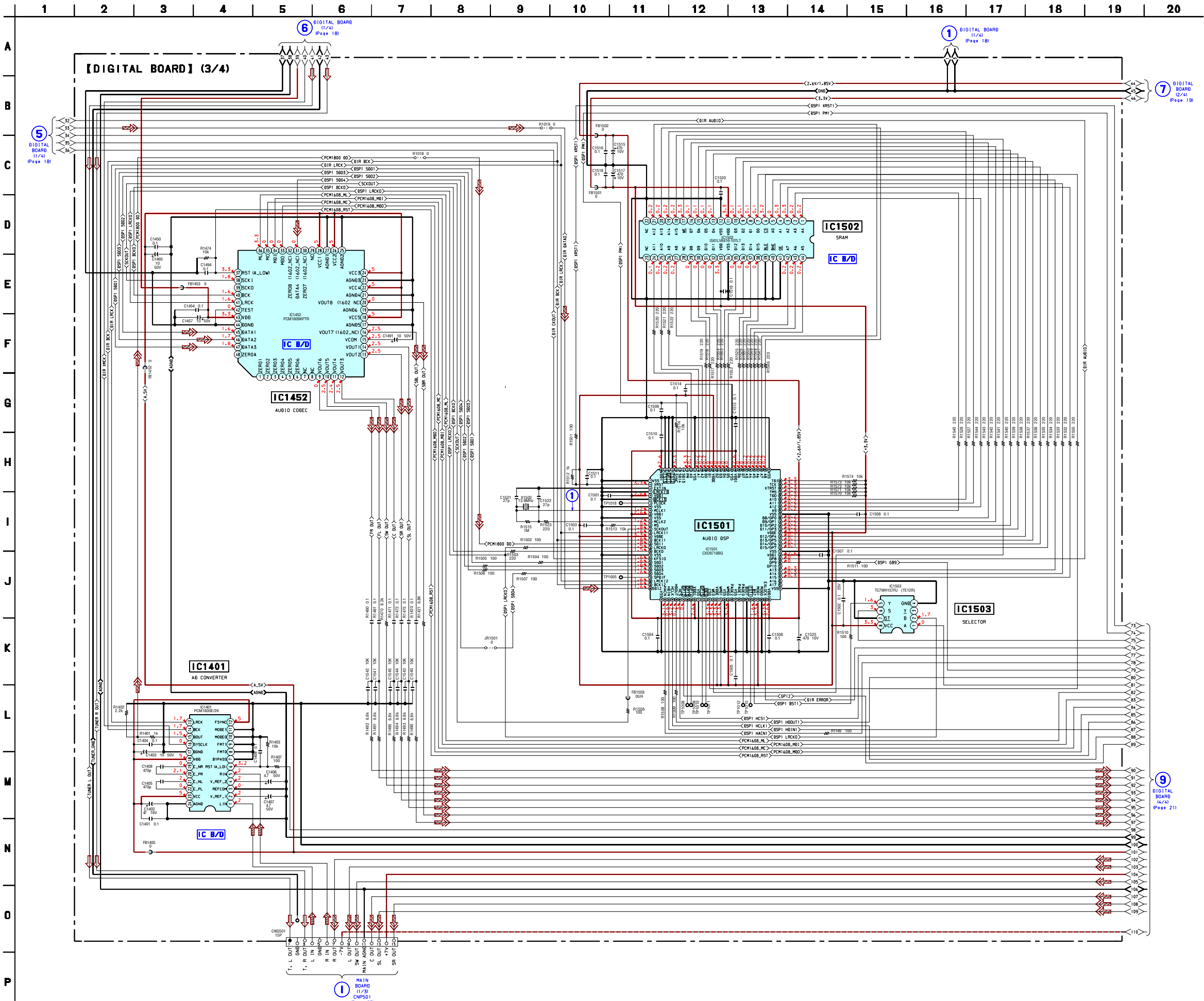
3-7. SCHEMATIC DIAGRAM – DIGITAL BOARD (3/4) – • See page 13 for Waveform. • See page 34, 35 for IC Block Diagram.
