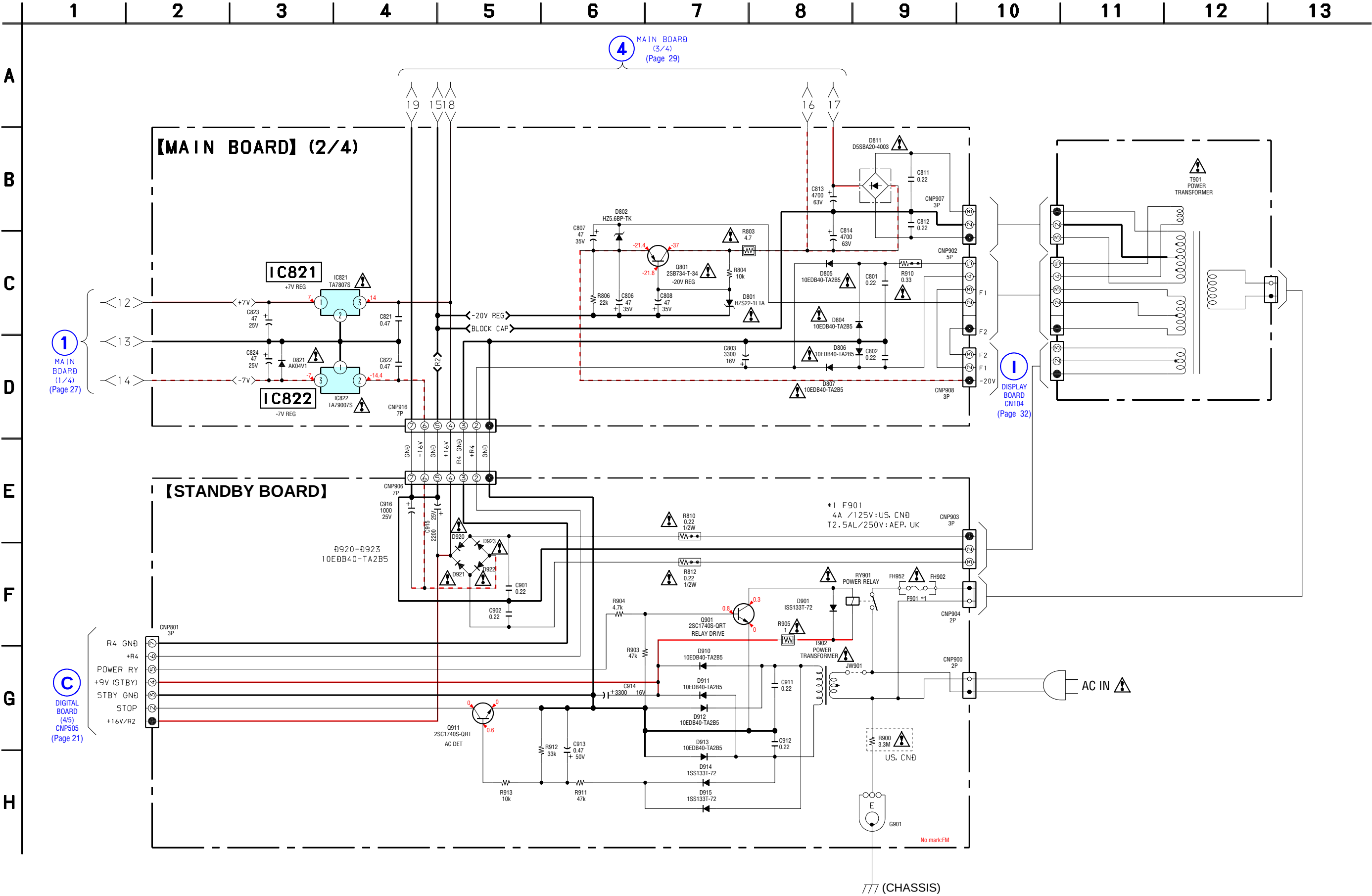
4-15. SCHEMATIC DIAGRAM – MAIN BOARD (2/4), STANDBY BOARD –
