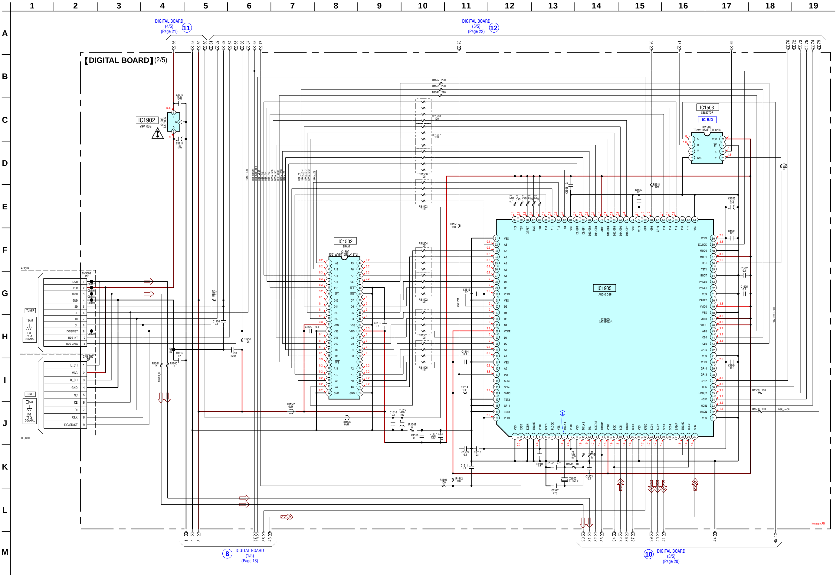
4-6. SCHEMATIC DIAGRAM – DIGITAL BOARD (2/5) – • See page 13 for Waveform. • See page 36 for IC Block Diagram.
