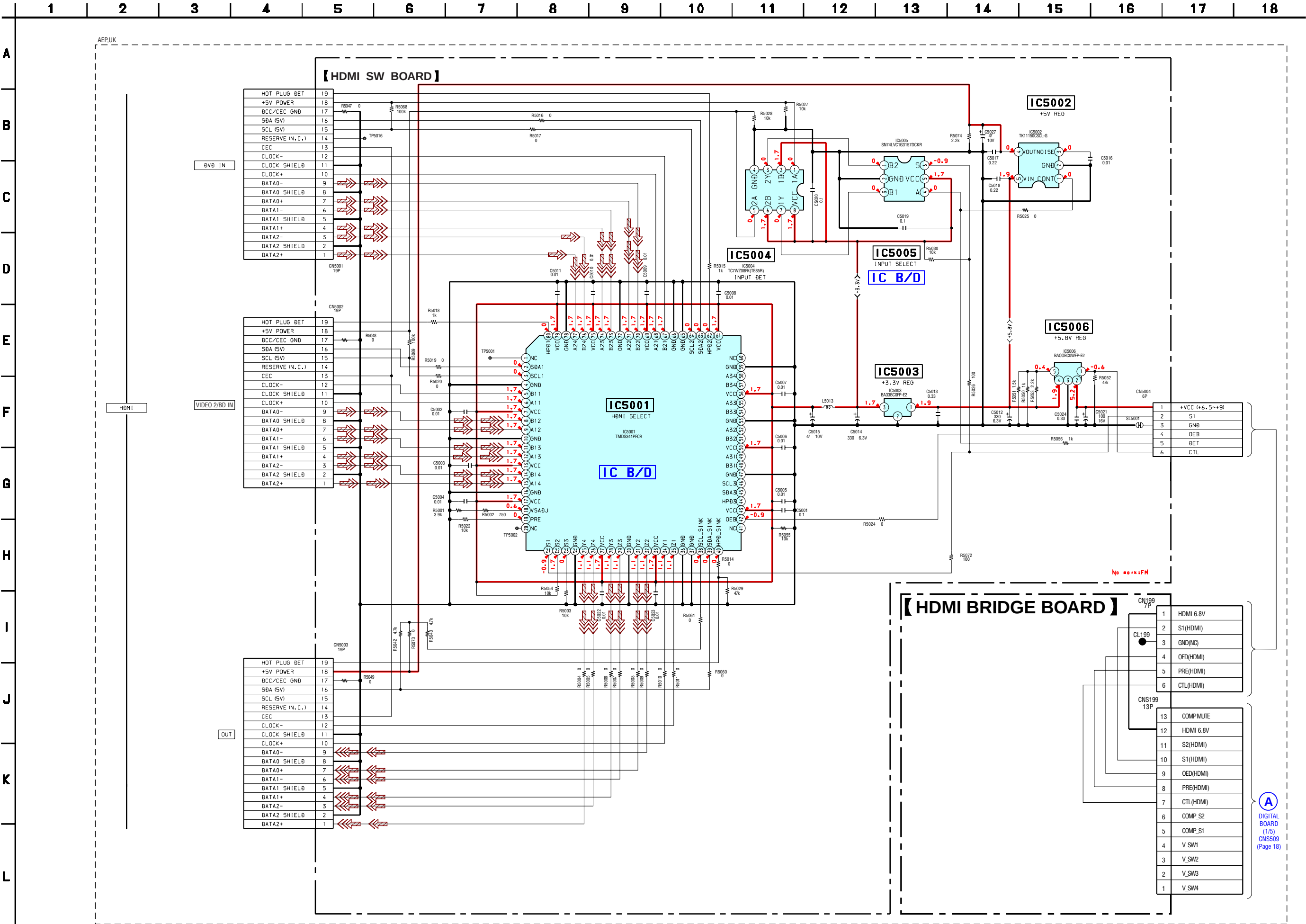
4-11. SCHEMATIC DIAGRAM – HDMI SW BOARD, HDMI BRIDGE BOARD (AEP, UK only) – • See page 37 for IC Block Diagrams.
