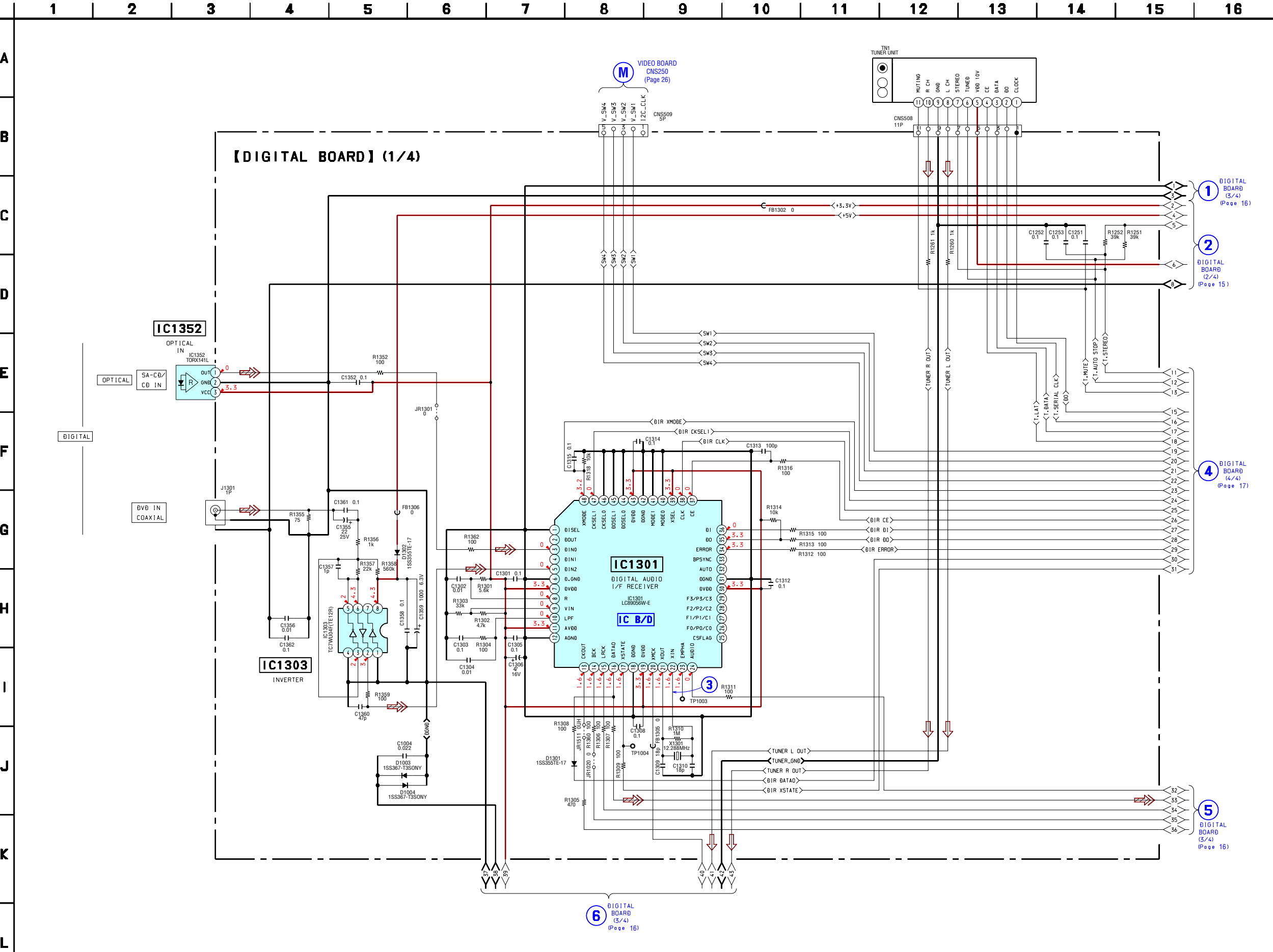
3-5. SCHEMATIC DIAGRAM — DIGITAL BOARD (1/4) — • See page 9 for Waveform. • See page 27 for IC Block Diagram.
