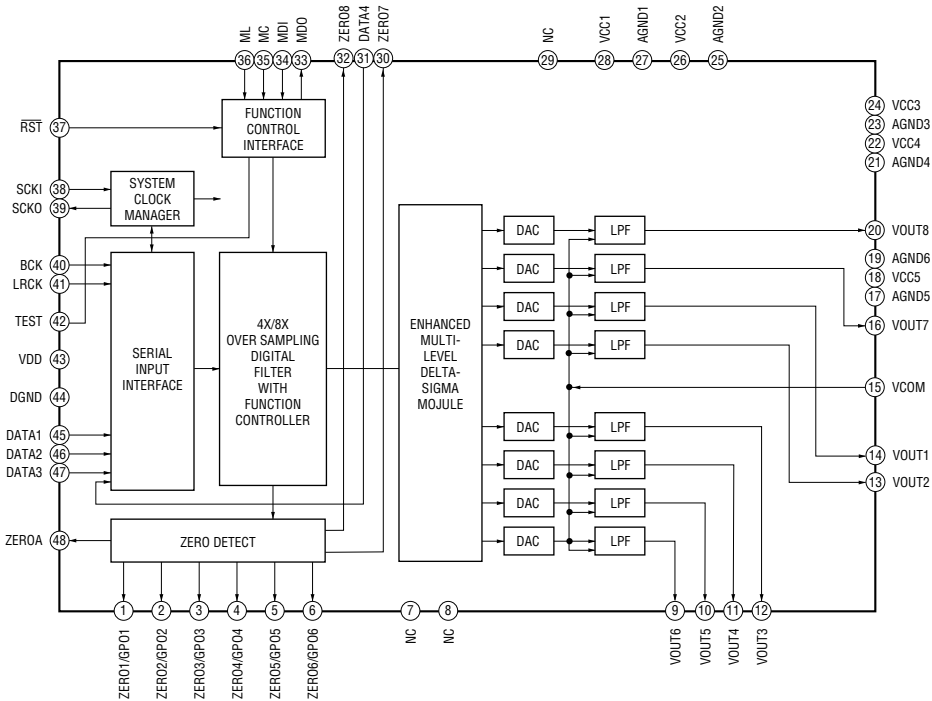
IC1452 PCM1602KYG/2K
