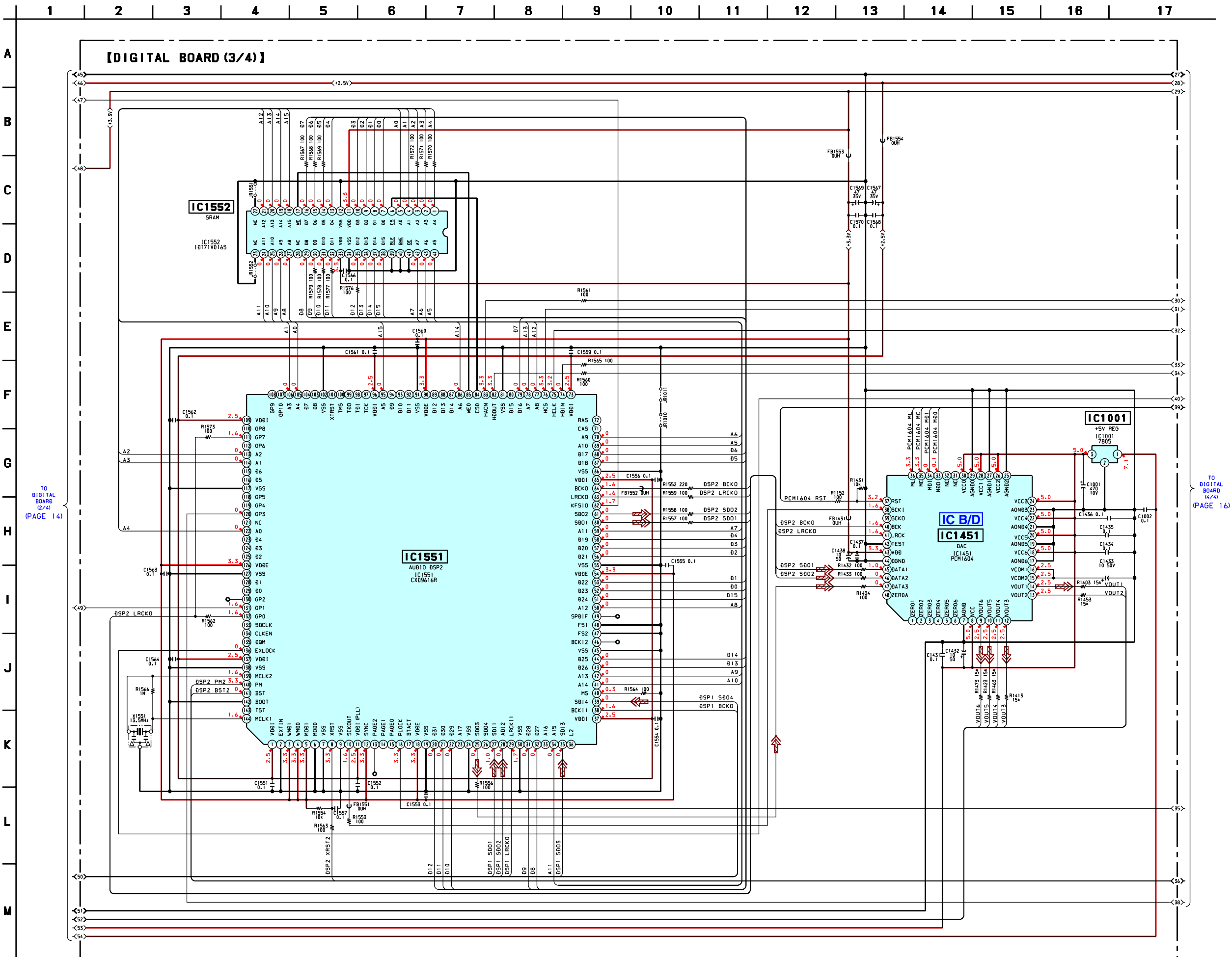
3-6. SCHEMATIC DIAGRAM – DIGITAL SECTION (3/4) – • See page 30 for IC Block Diagrams.
