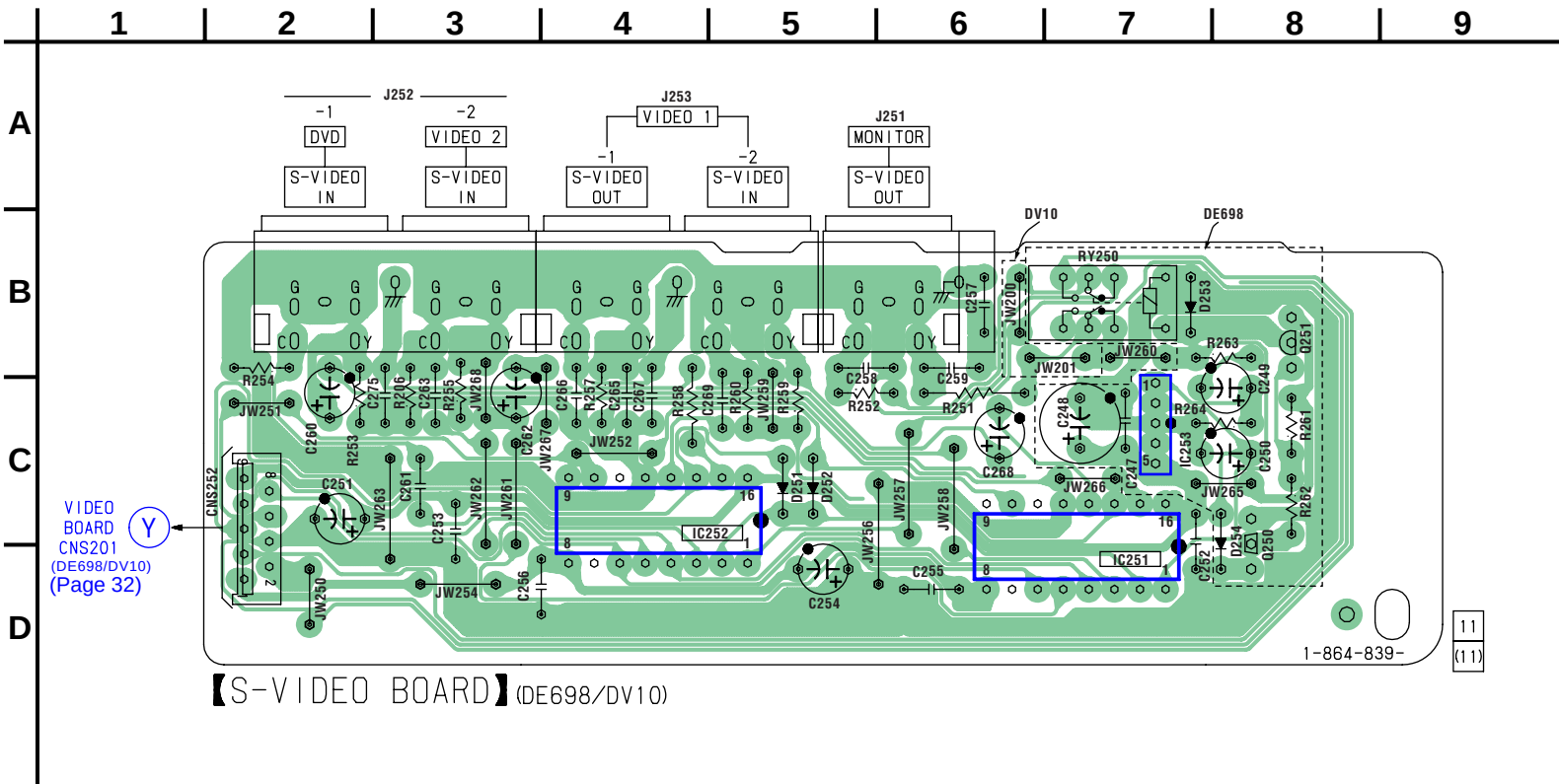
4-22. PRINTED WIRING BOARD — S-VIDEO SECTION (STR-DE698/DV10) — • Refer to page 14 for Circuit Boards Location.
