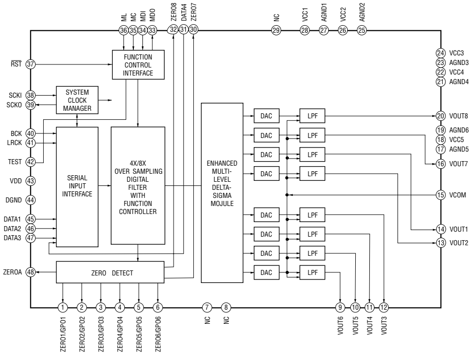
IC1452 PCM1609KPTR (DIGITAL BOARD (3/4))
