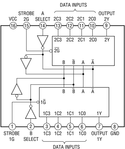
IC1302 TC74ACT153F(EL) (DIGITAL BOARD (1/4)) (STR-DE698/DV10)
