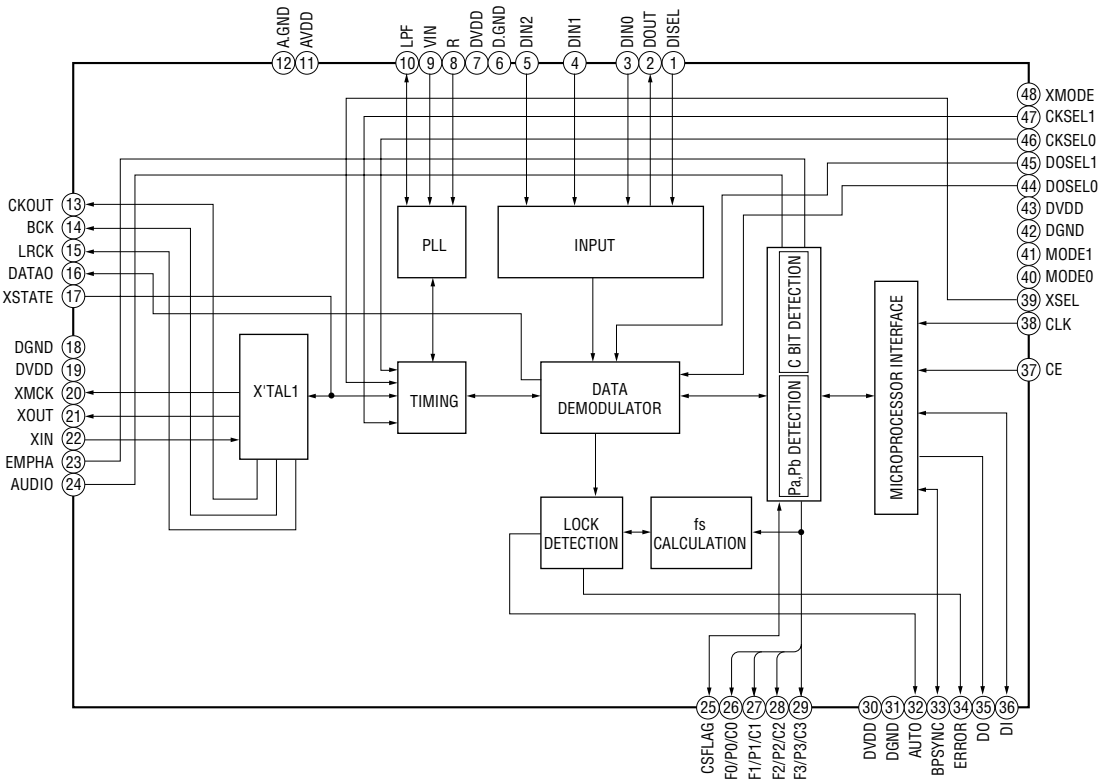
IC1301 LC89056W-E (DIGITAL BOARD (1/4))
