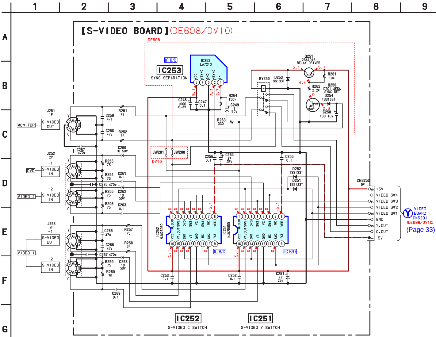
4-23. SCHEMATIC DIAGRAM — S-VIDEO SECTION (STR-DE698/DV10) — • Refer to page 41 for IC Block Diagrams.
