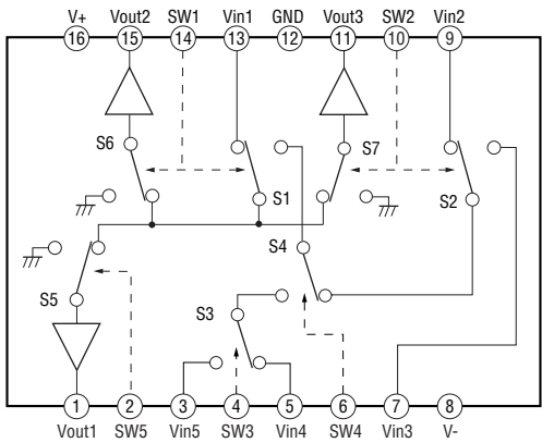
IC750, 752 NJM2296D (S-VIDEO Board)
