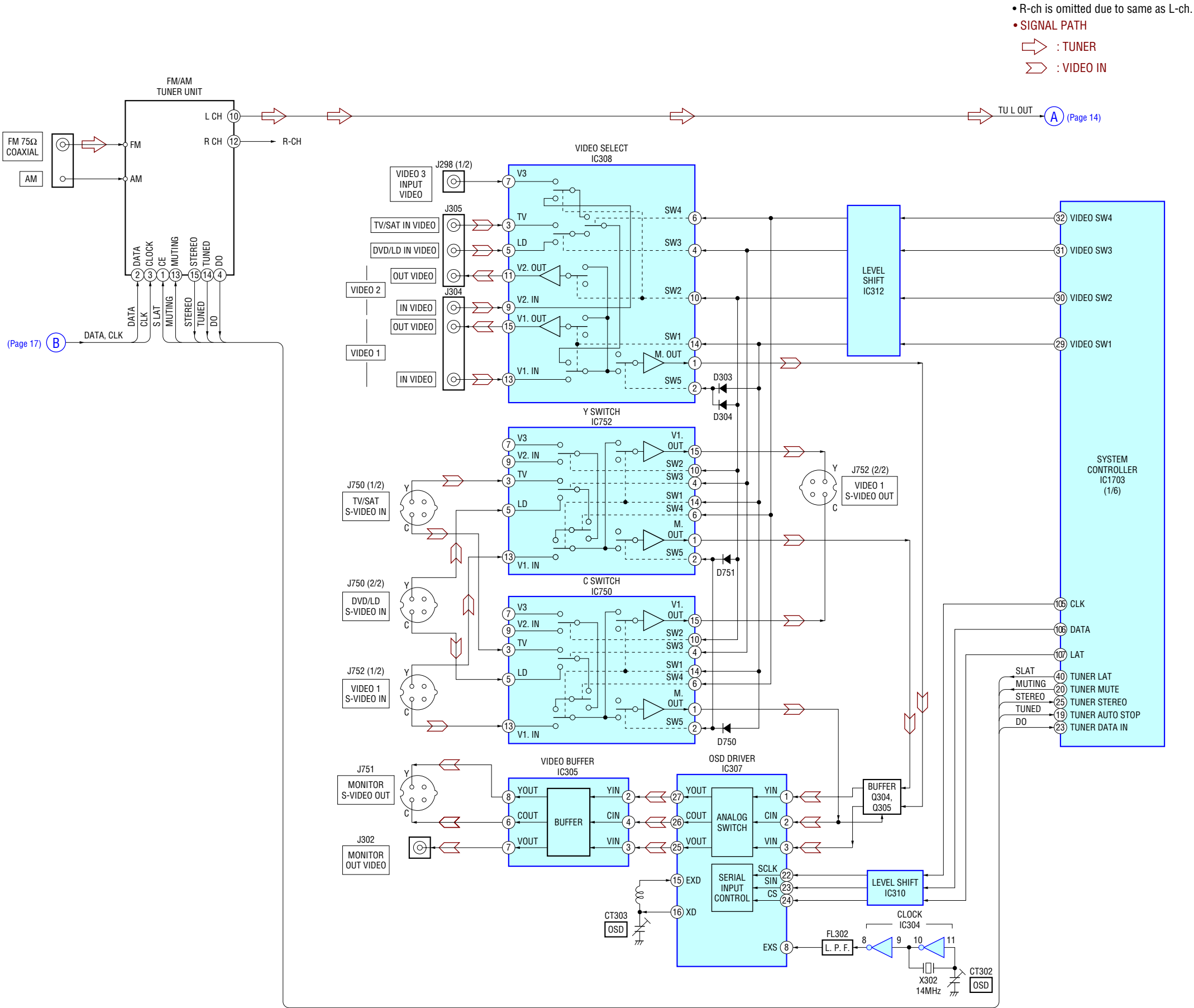
6-1. BLOCK DIAGRAM – TUNER/VIDEO INPUT Section –
