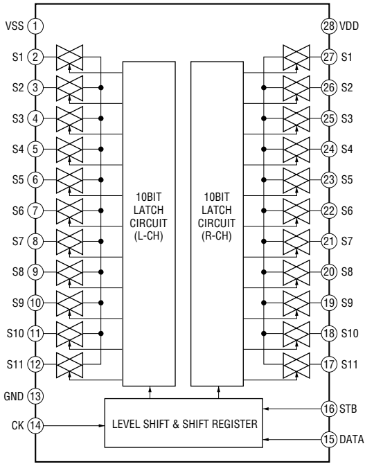
IC105 TC9273N-013 (MAIN Board)
