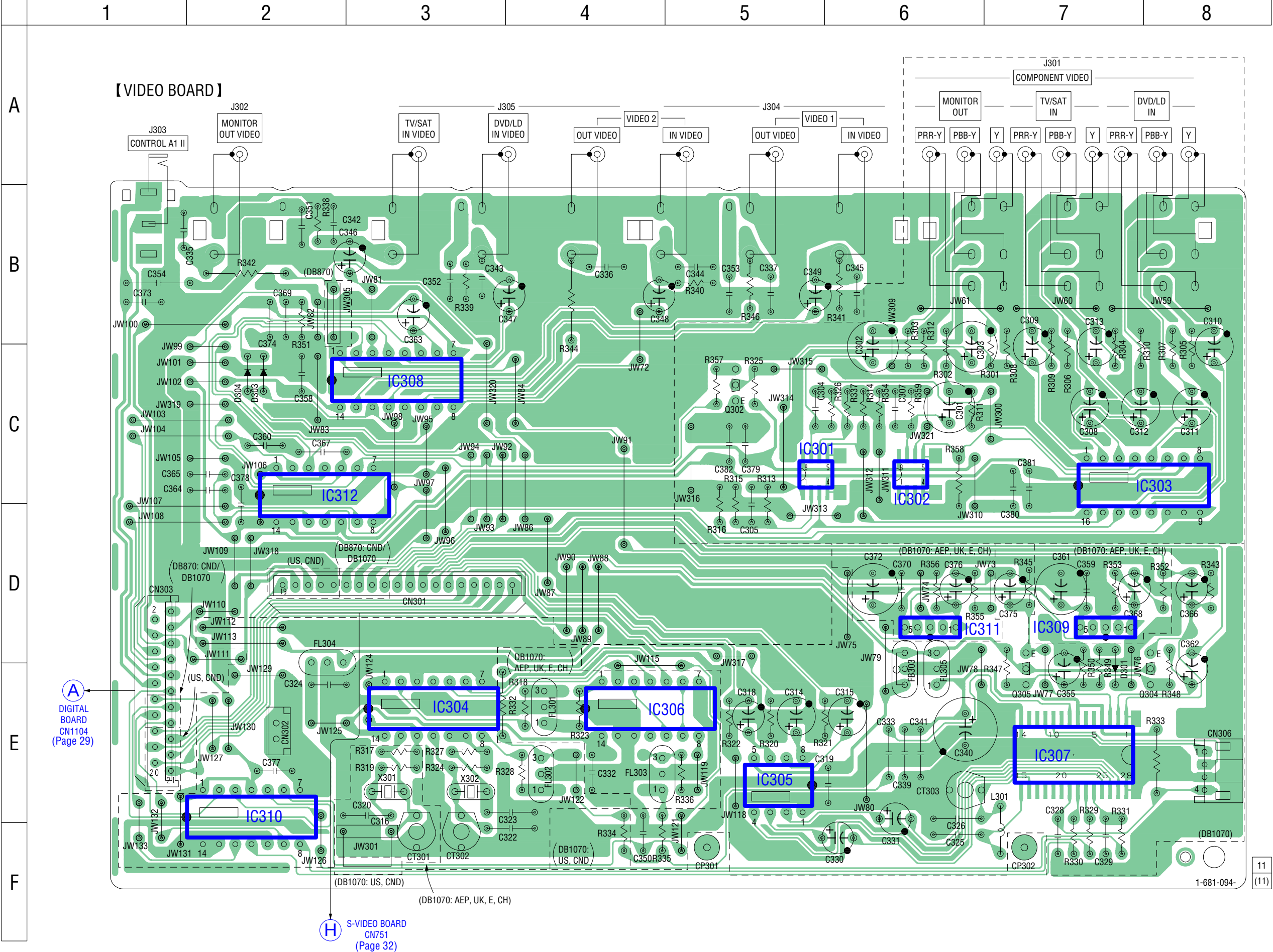
6-15. PRINTED WIRING BOARD – VIDEO Board – • See page 22 for Circuit Boards Location.
