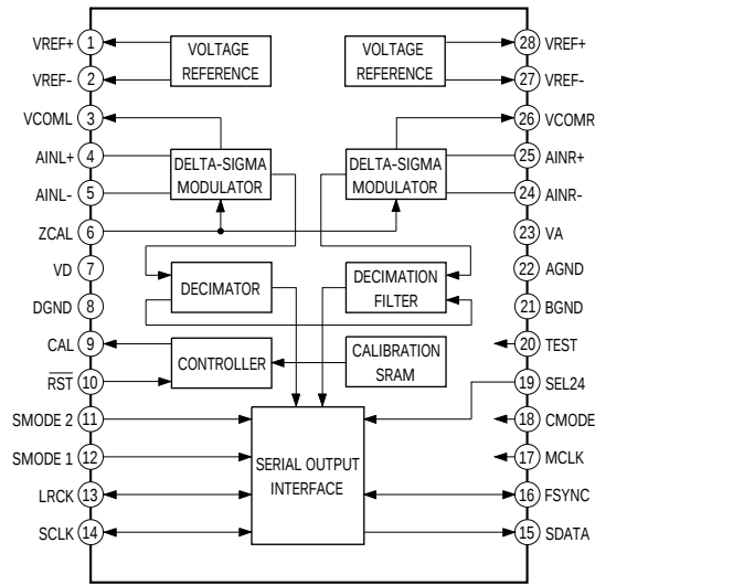
IC3104 CXD8681M-TP (DIGITAL BOARD)
