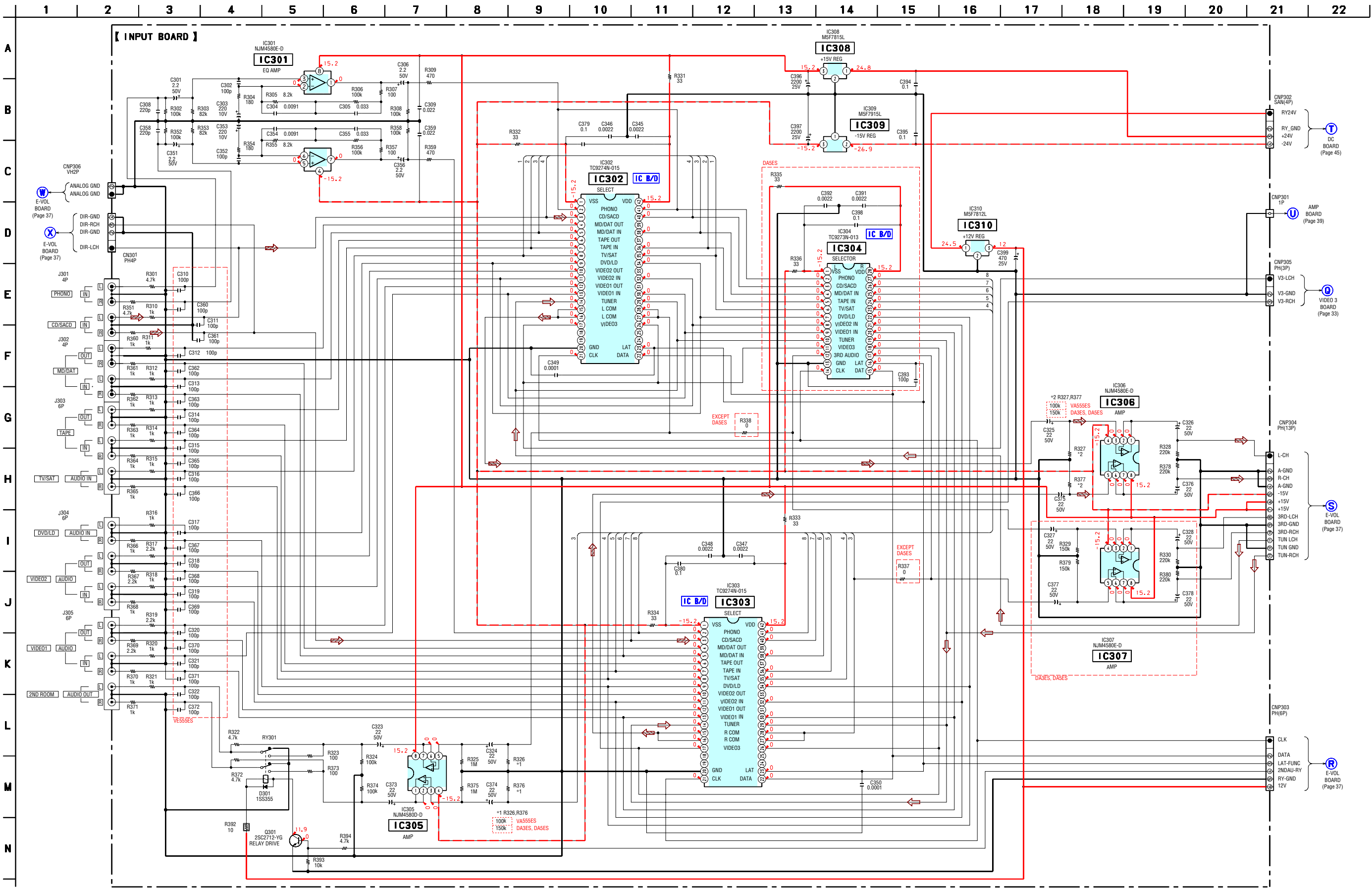
5-15. SCHEMATIC DIAGRAM — INPUT SECTION — • See page 53 for IC Block Diagram.
