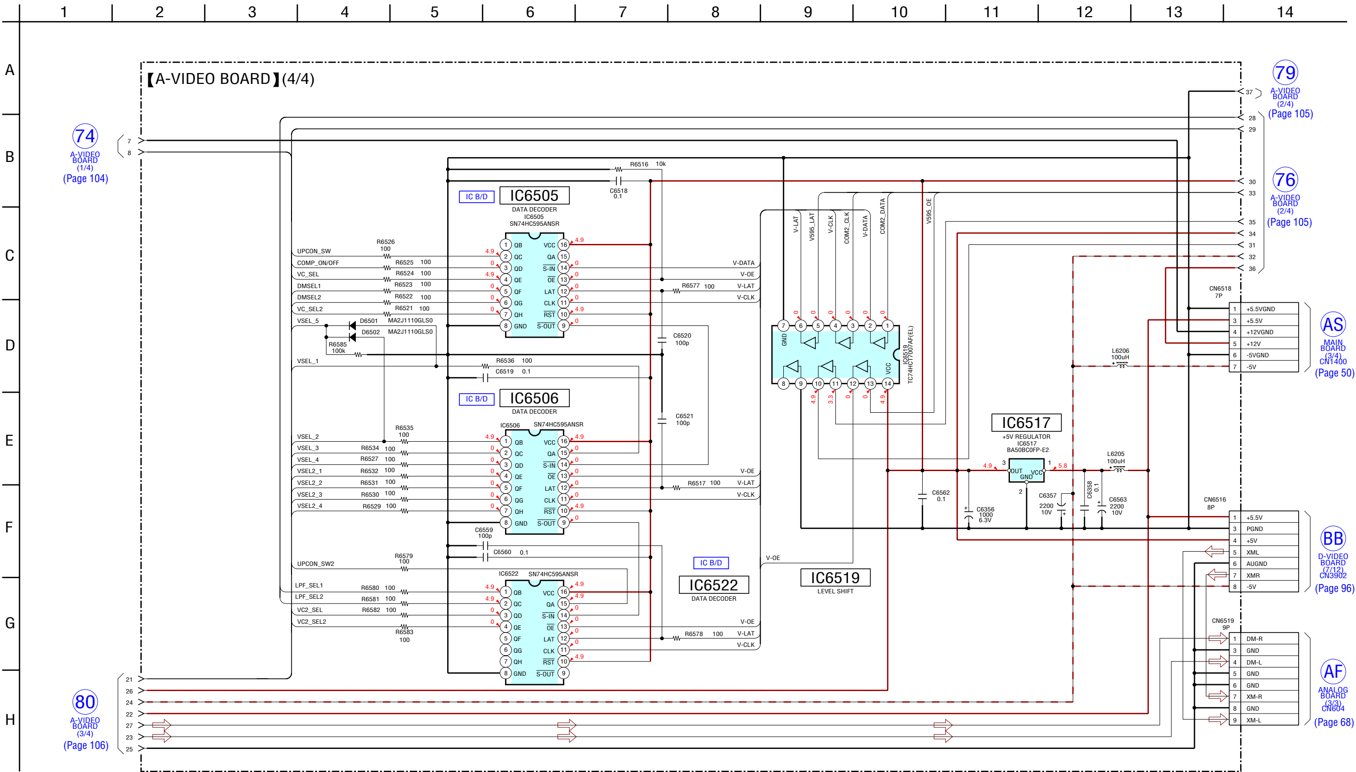
6-75. SCHEMATIC DIAGRAM – A-VIDEO Board (4/4) – • See page 127 for IC Block Diagrams.
