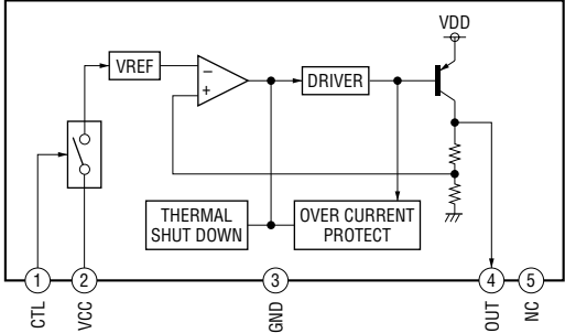
IC3905 BA00BC0WFP-E2
