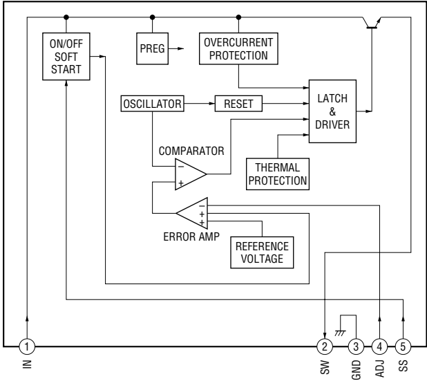
IC1402, 1403 SI-8008HFE
