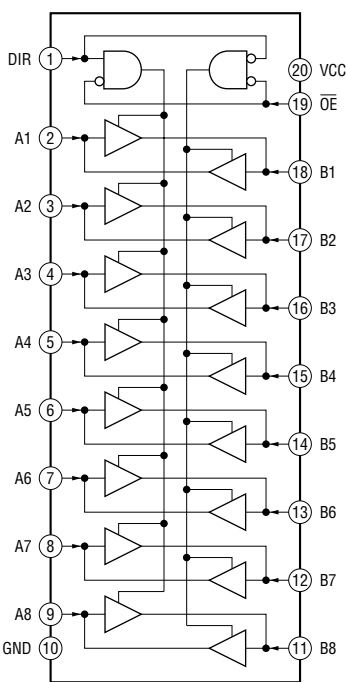
IC3619, 3620 TC74LCX245FK (EL)
