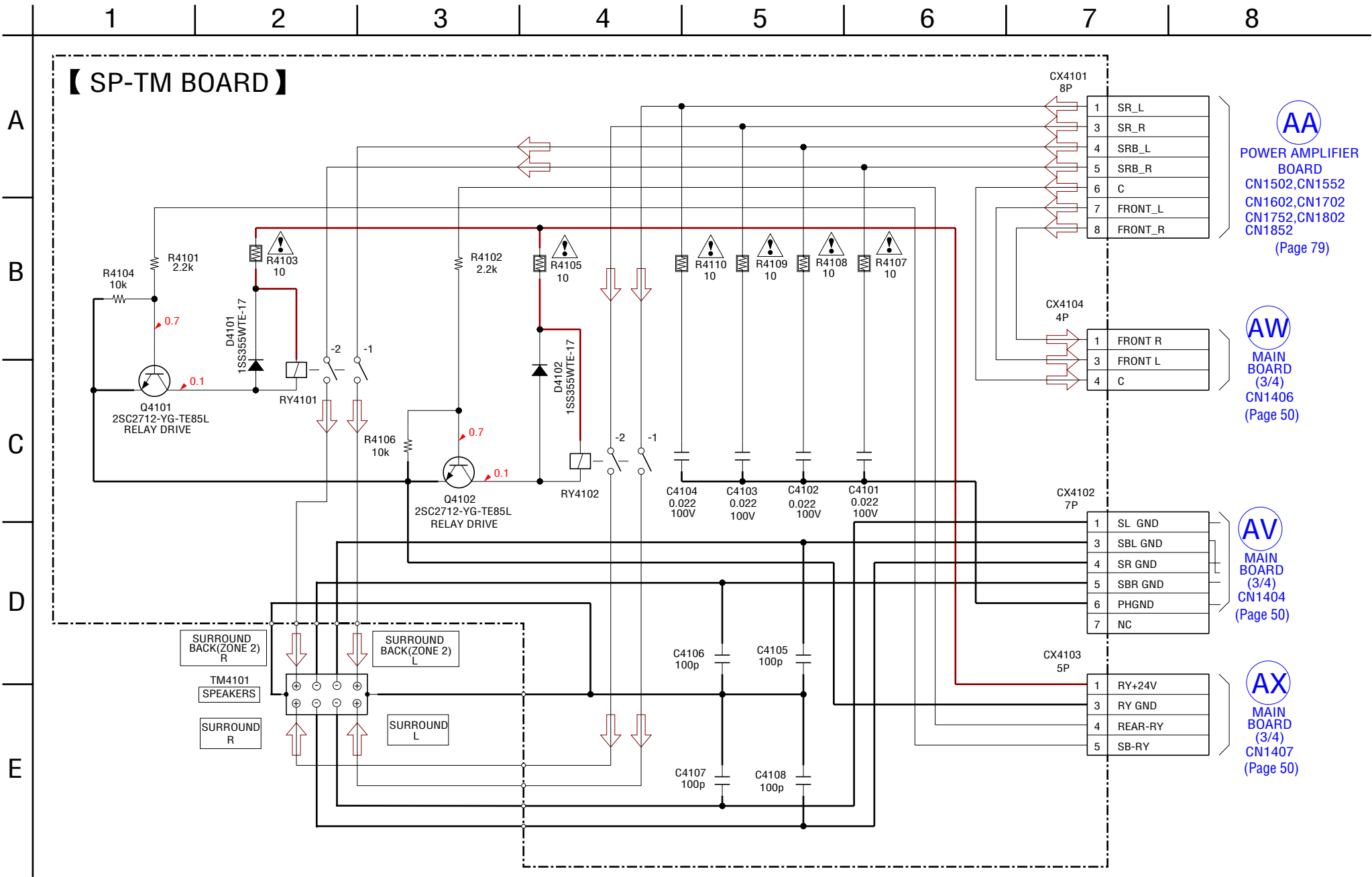
6-55. SCHEMATIC DIAGRAM – SP-TM Board –
