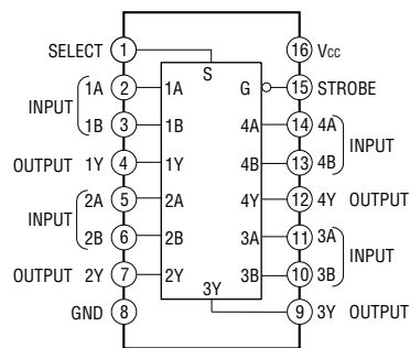
IC2212 – 2214 TC74VHC157FT (EKJ)
