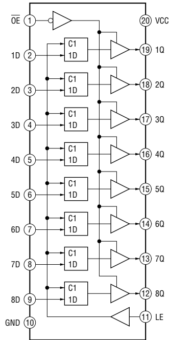
IC5009, 5010, 5209, 5210 SN74LVC573APWR
