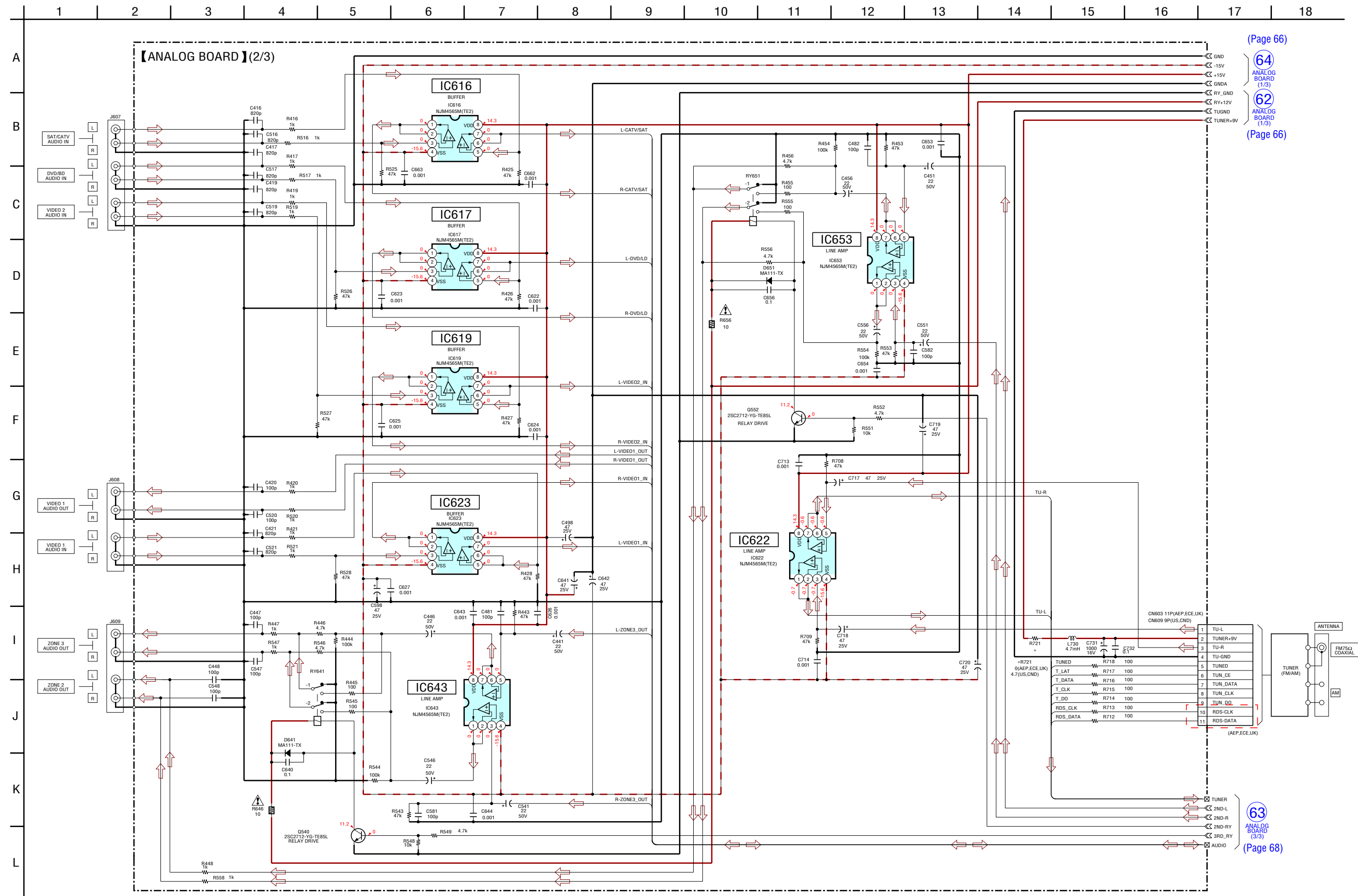
6-34. SCHEMATIC DIAGRAM – ANALOG Board (2/3) –
