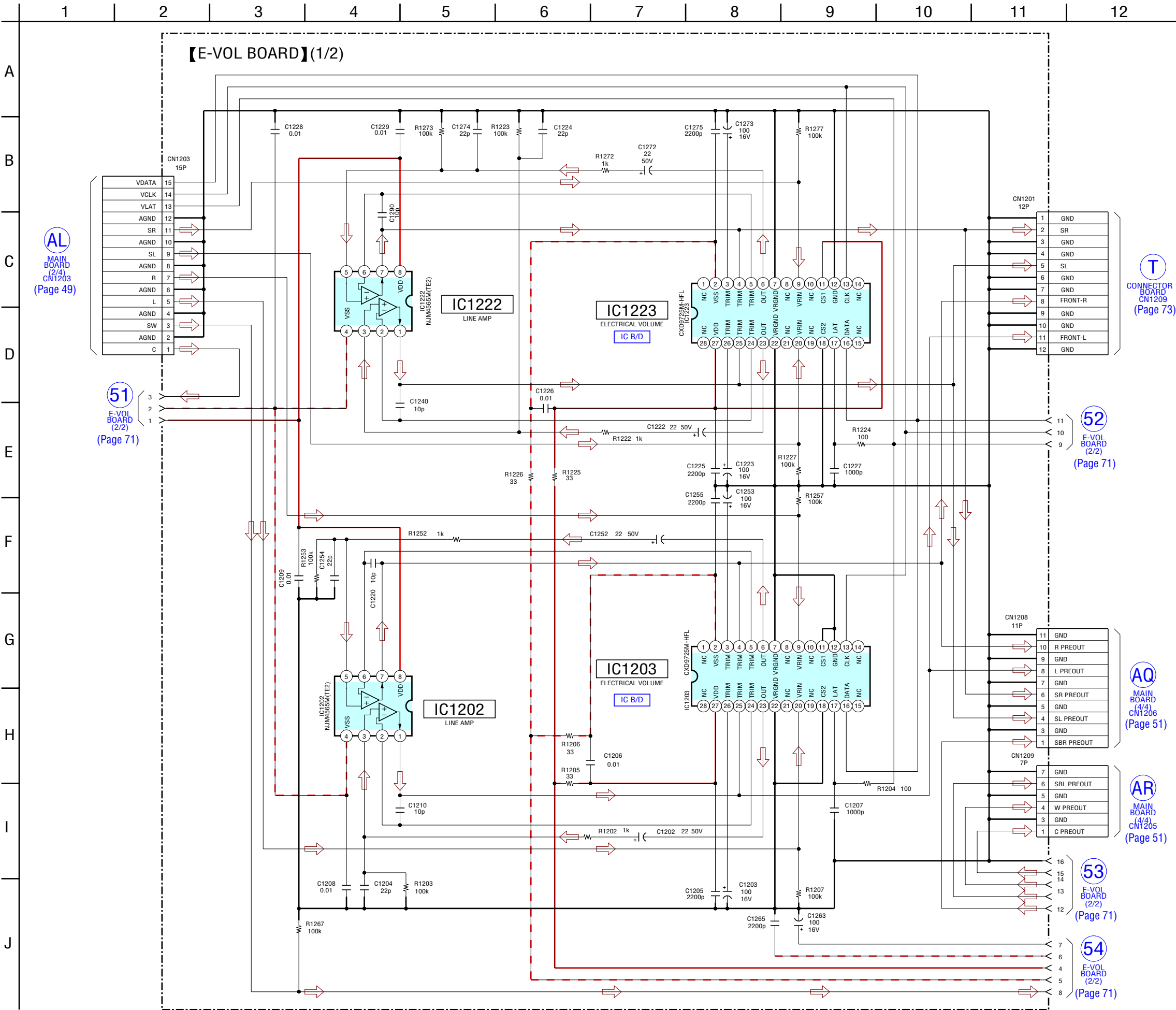
6-37. SCHEMATIC DIAGRAM – E-VOL Board (1/2) – • See page 127 for IC Block Diagrams.
