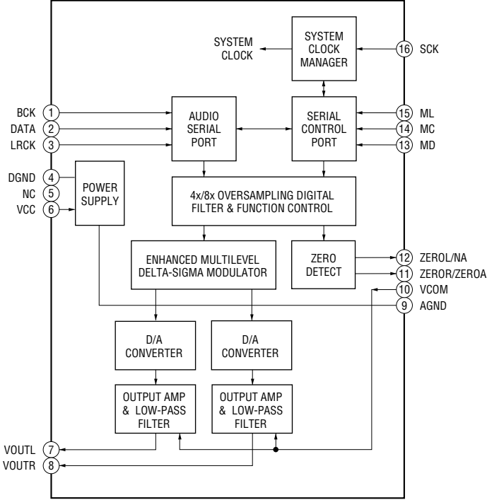
IC3904 PCM1753DBQR
