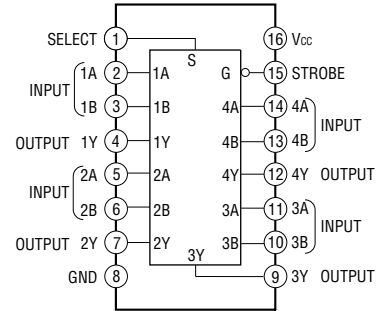
IC5013 TC74VHC157FT (EKJ)
