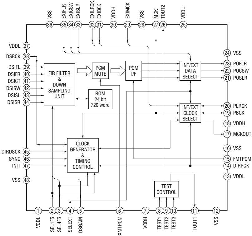
IC3519 CXD9850Q
