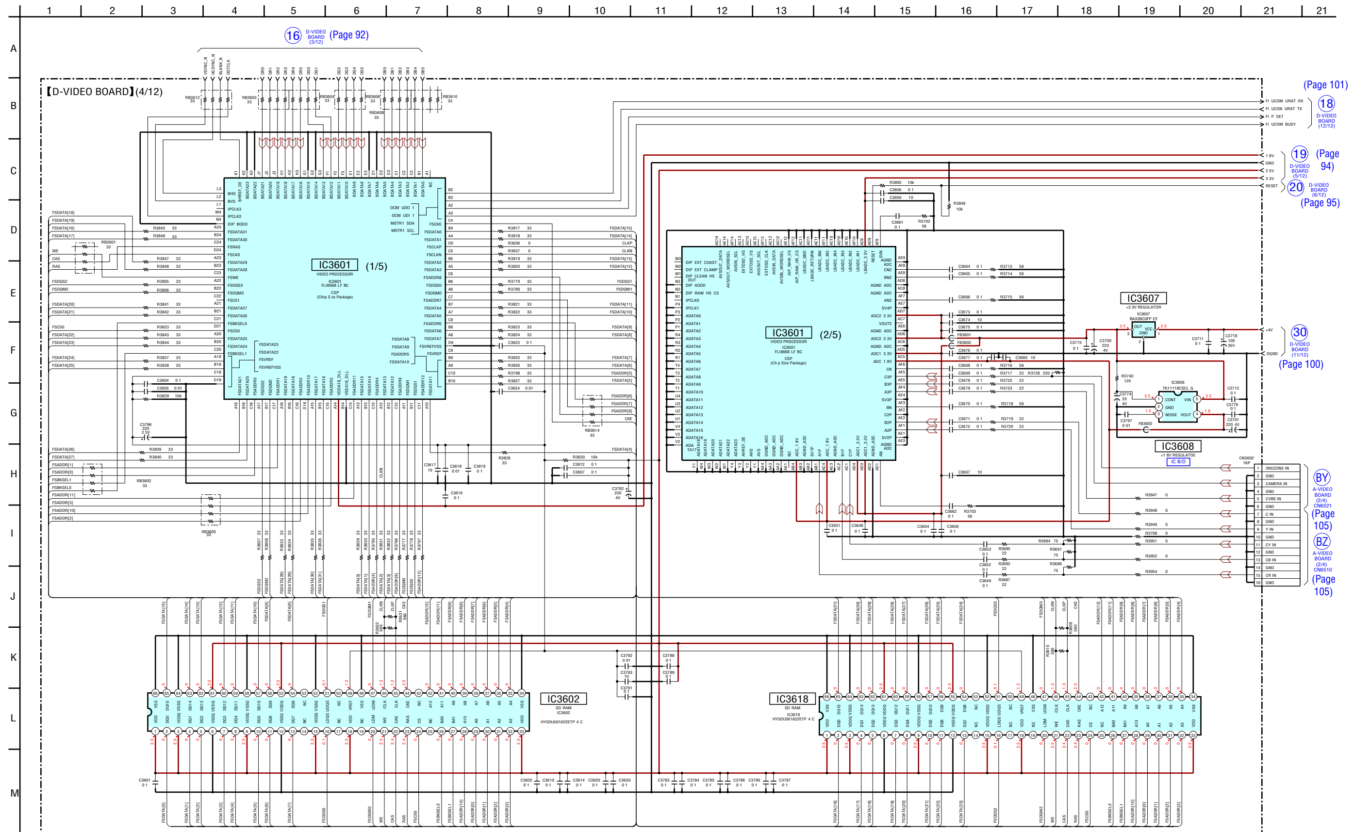
6-61. SCHEMATIC DIAGRAM – D-VIDEO Board (4/12) – • See page 127 for IC Block Diagrams. • See page 141 for IC Pin Function Description.
