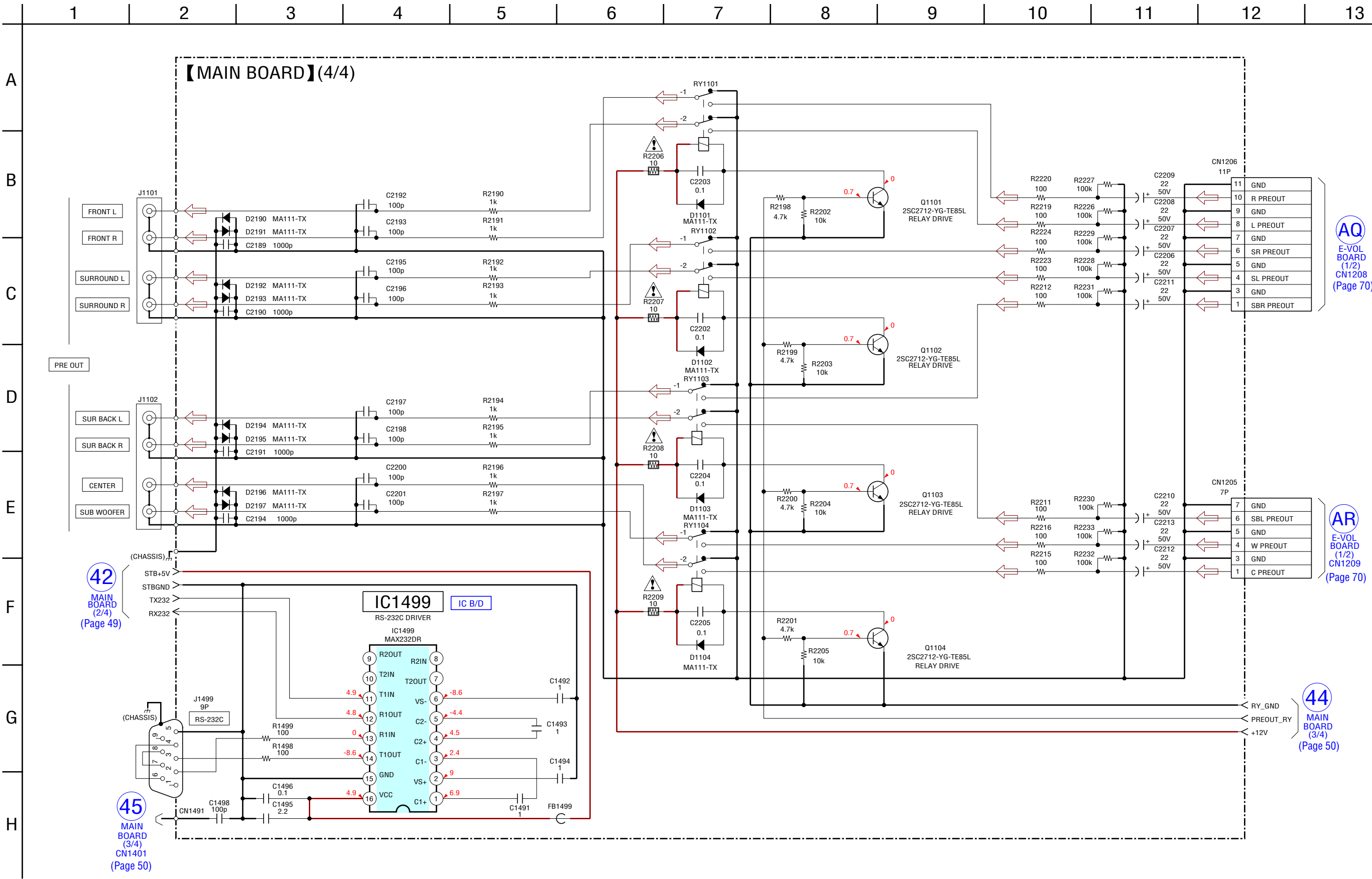
6-18. SCHEMATIC DIAGRAM – MAIN Board (4/4) – • See page 127 for IC Block Diagrams.
