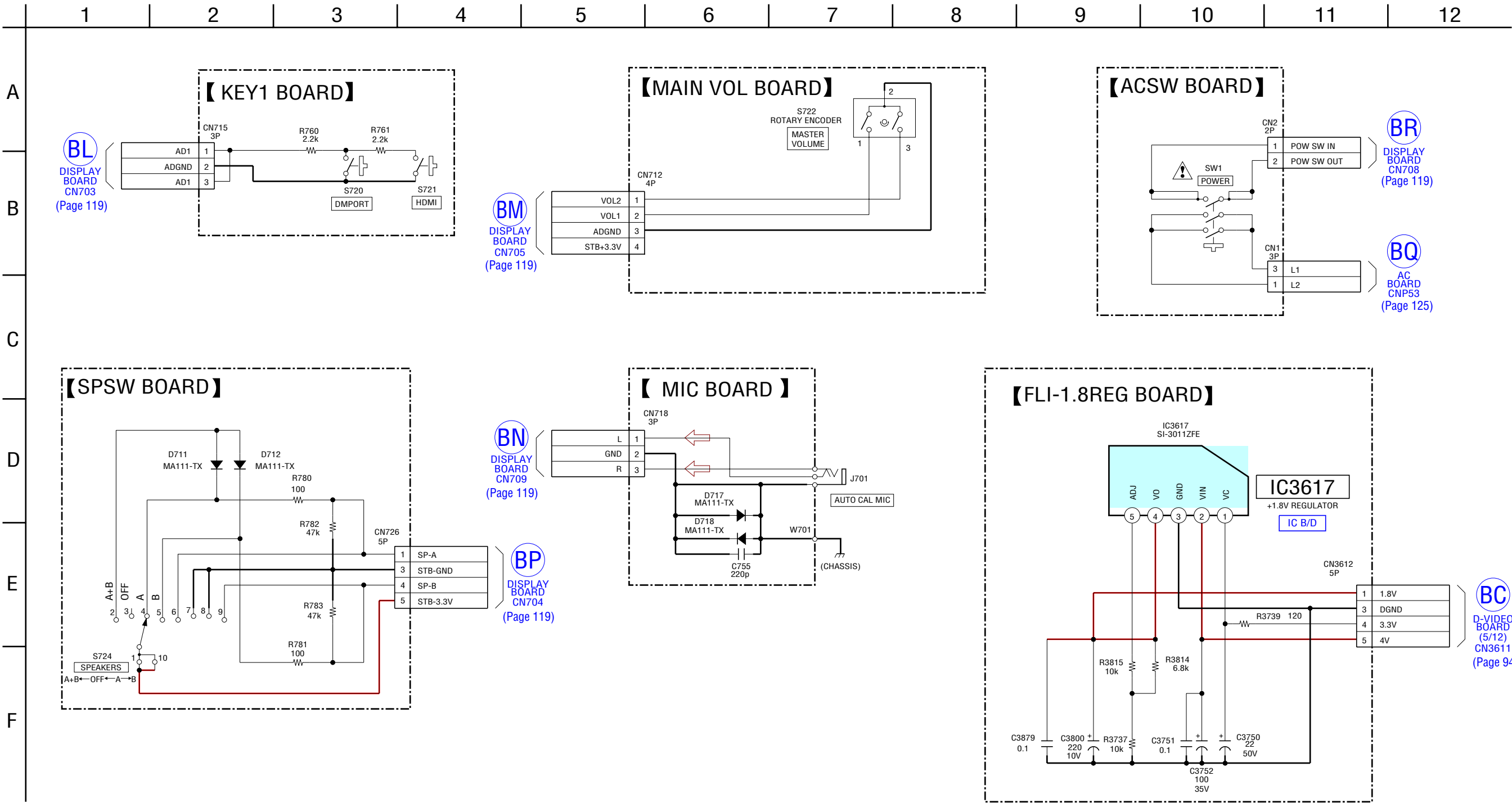
6-89. SCHEMATIC DIAGRAM – PANEL Section – • See page 127 for IC Block Diagrams.
