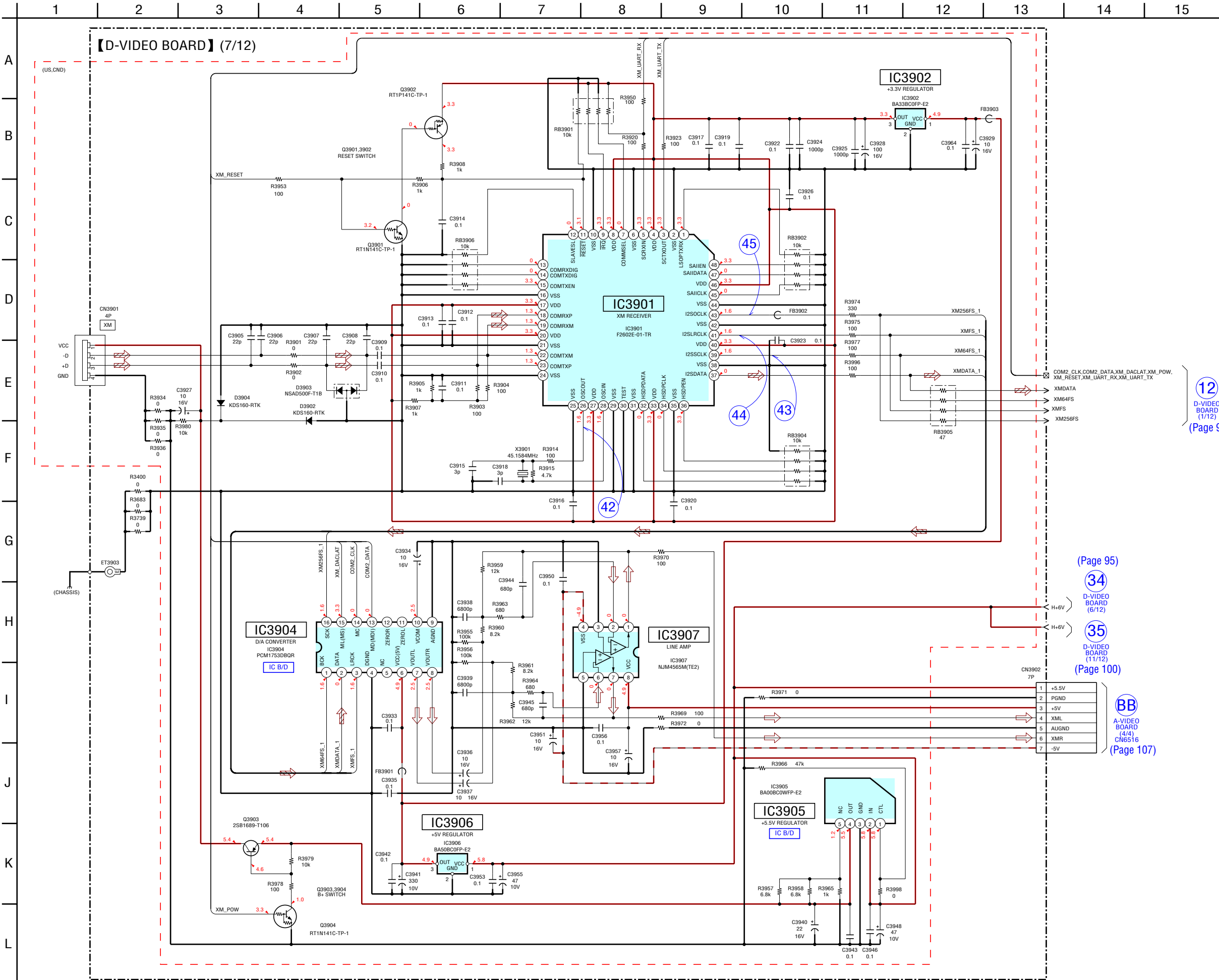
6-64. SCHEMATIC DIAGRAM – D-VIDEO Board (7/12) – • See page 126 for Waveforms. • See page 127 for IC Block Diagrams. • See page 141 for IC Pin Function Description.
