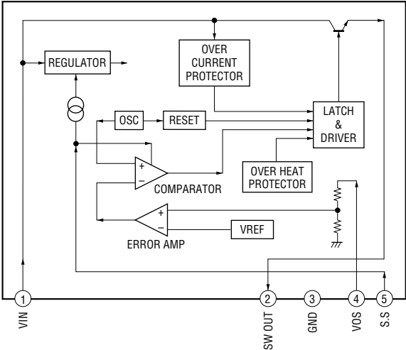
IC1401, 1404 SI-8050S-LF1101
