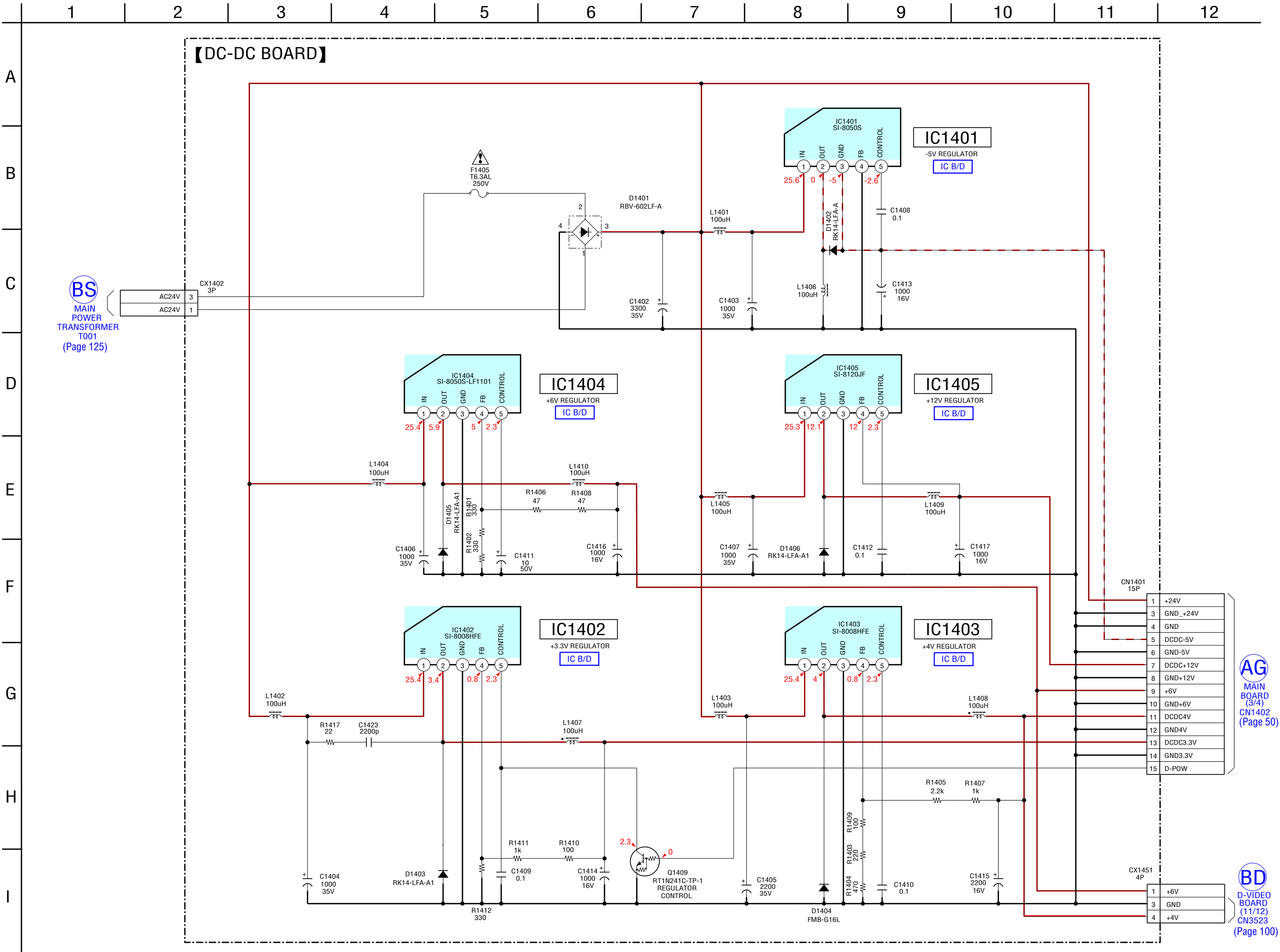
6-91. SCHEMATIC DIAGRAM – DC-DC Board – • See page 127 for IC Block Diagrams.
