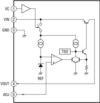
IC3853 SI-3010KM-TL
