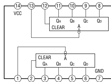
IC2211, 2216 TC74VHC393FT (EL)
