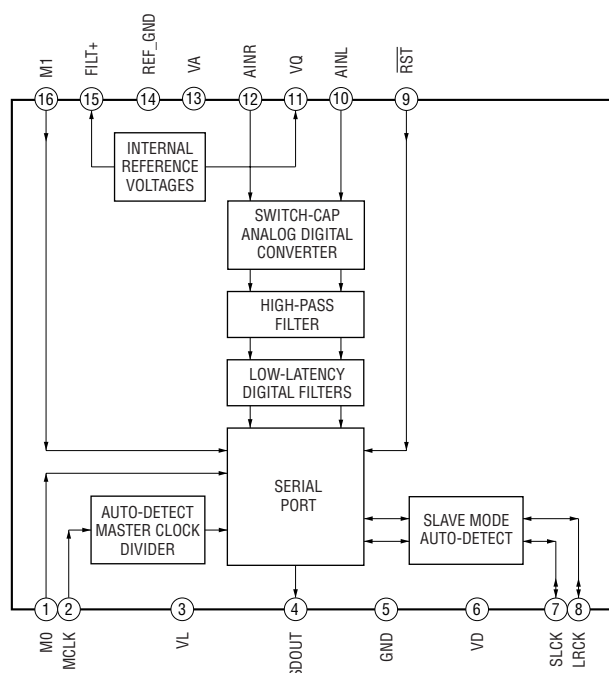
IC2217 CS5340-CZZR
