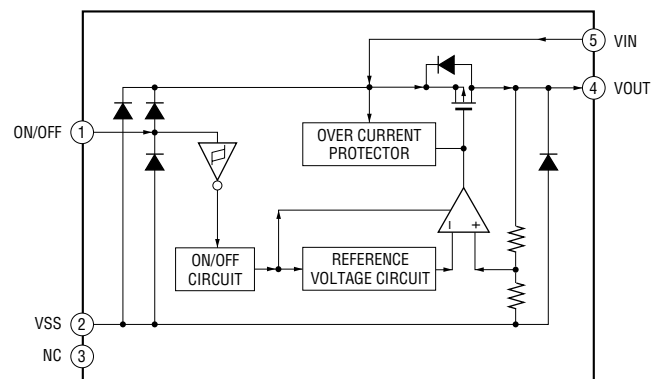
IC2215 S-T111B33MC-OGSTFG
