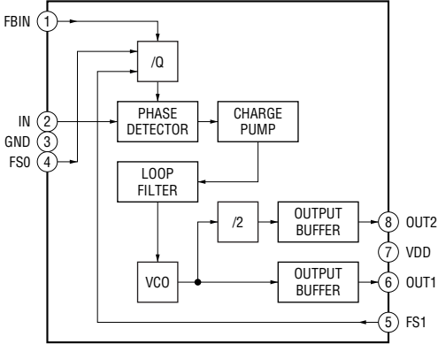
IC3854 CY2302-SXC-1T
