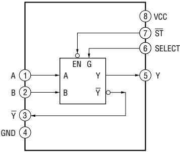
IC3518 TC7WH157FU (TE12R)
