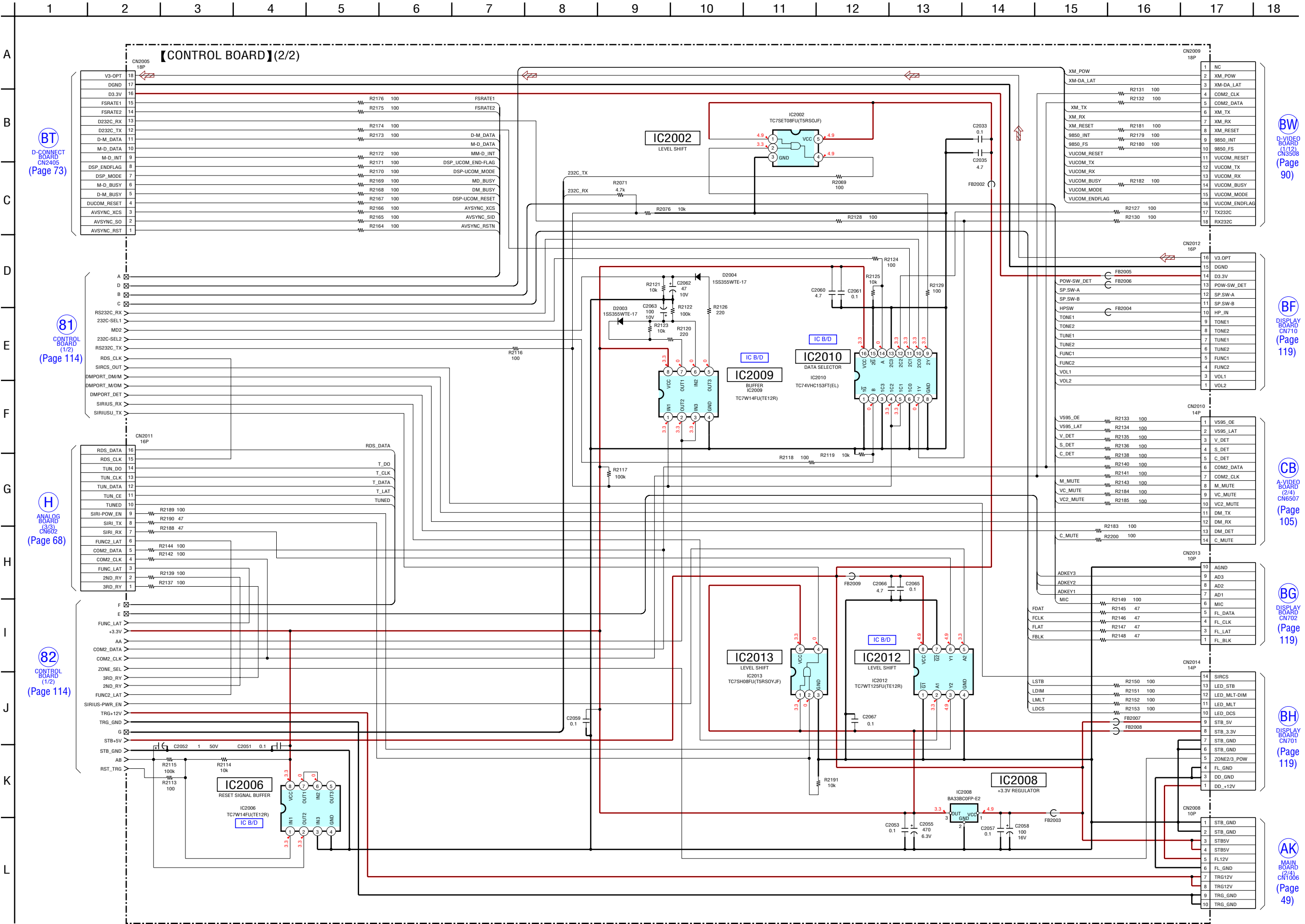
6-83. SCHEMATIC DIAGRAM – CONTROL Board (2/2) – • See page 127 for IC Block Diagrams.
