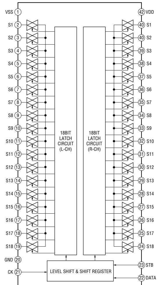
IC401, 501 TC9274CNG-015
