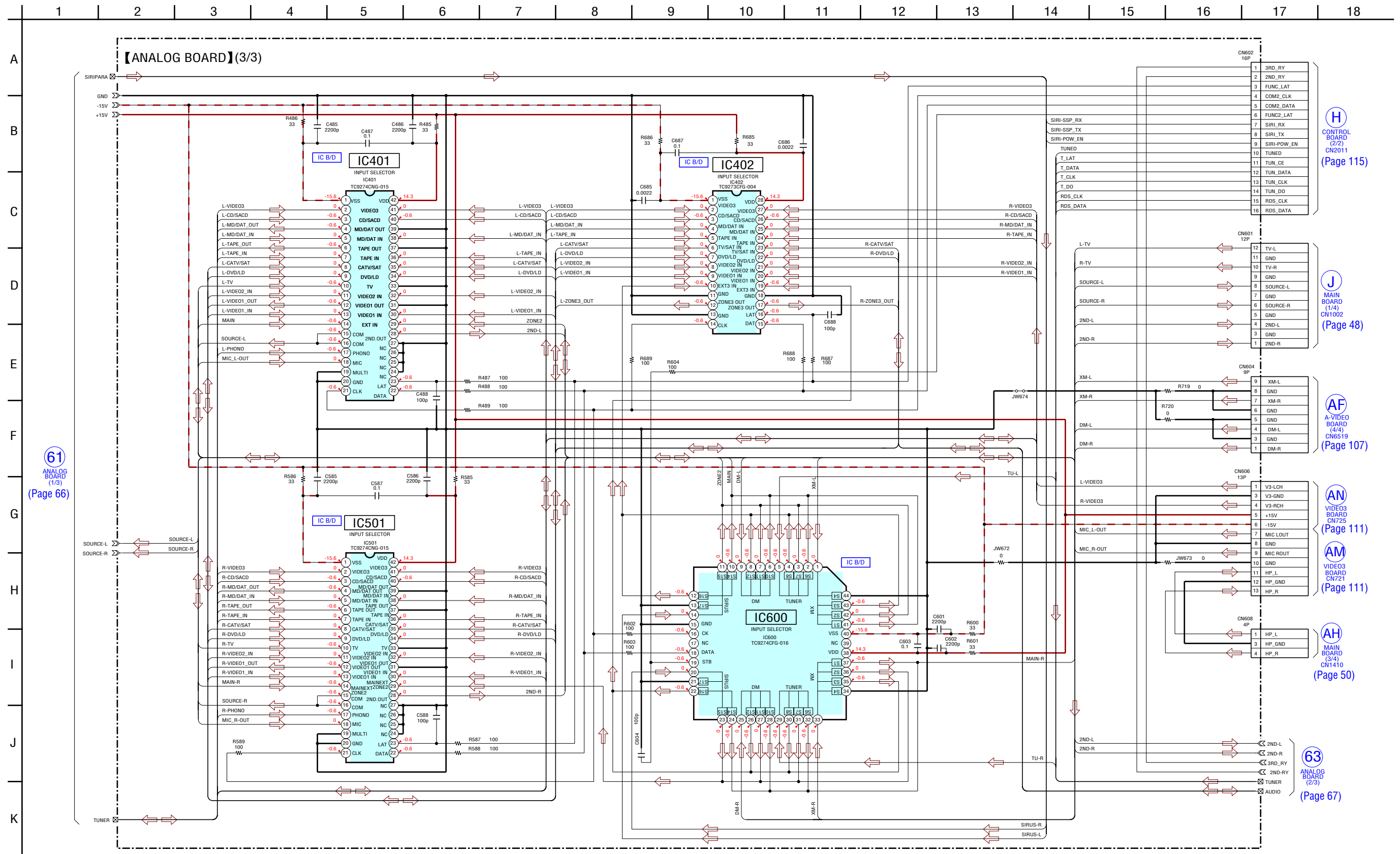
6-35. SCHEMATIC DIAGRAM – ANALOG Board (3/3) – • See page 127 for IC Block Diagrams.
