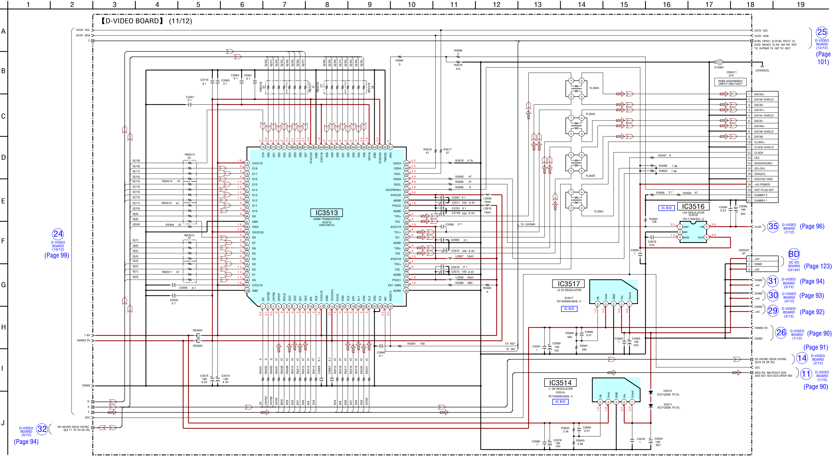
6-68. SCHEMATIC DIAGRAM – D-VIDEO Board (11/12) – • See page 127 for IC Block Diagrams. • See page 141 for IC Pin Function Description.
