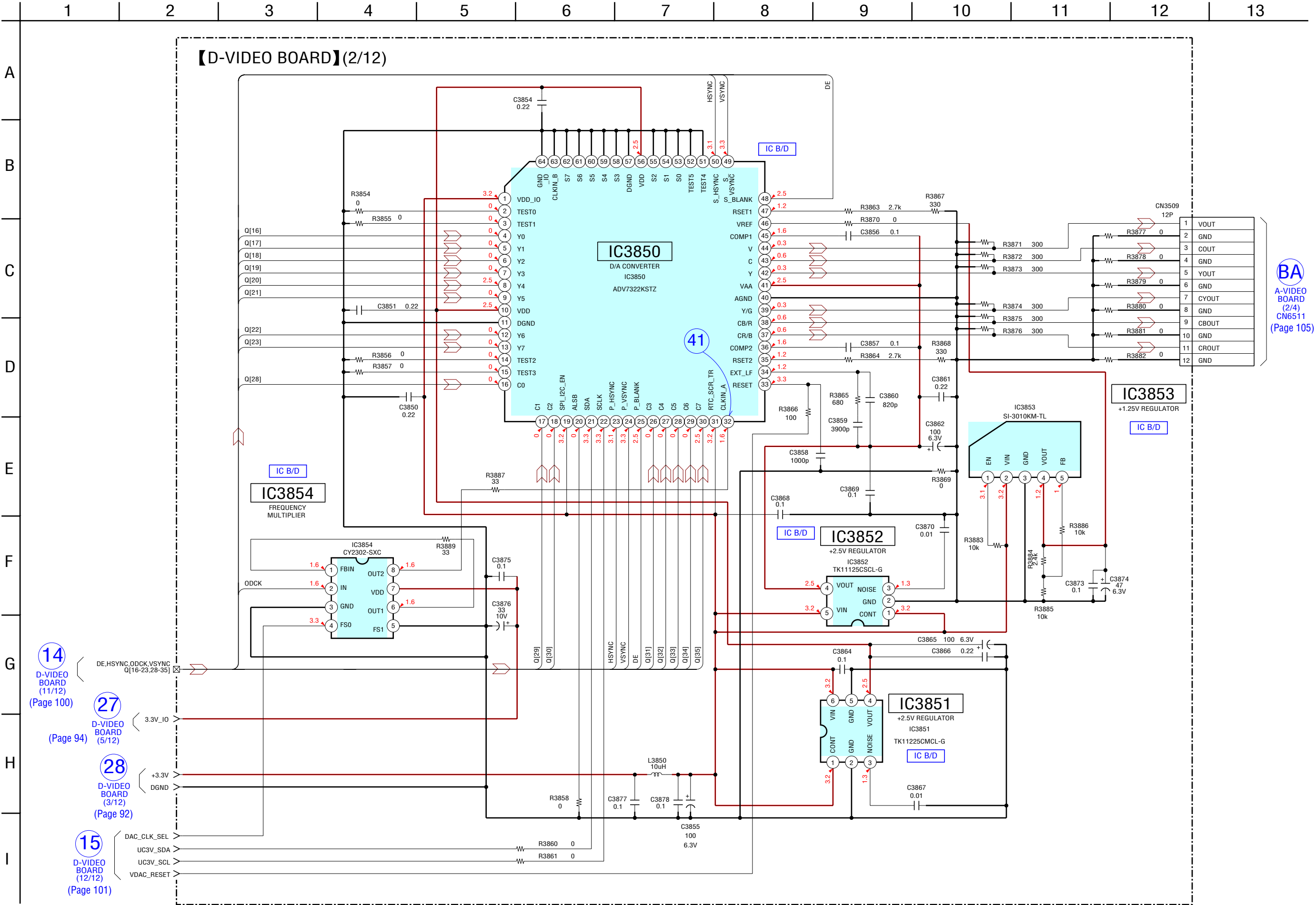
6-59. SCHEMATIC DIAGRAM – D-VIDEO Board (2/12) – • See page 126 for Waveforms. • See page 127 for IC Block Diagrams.
