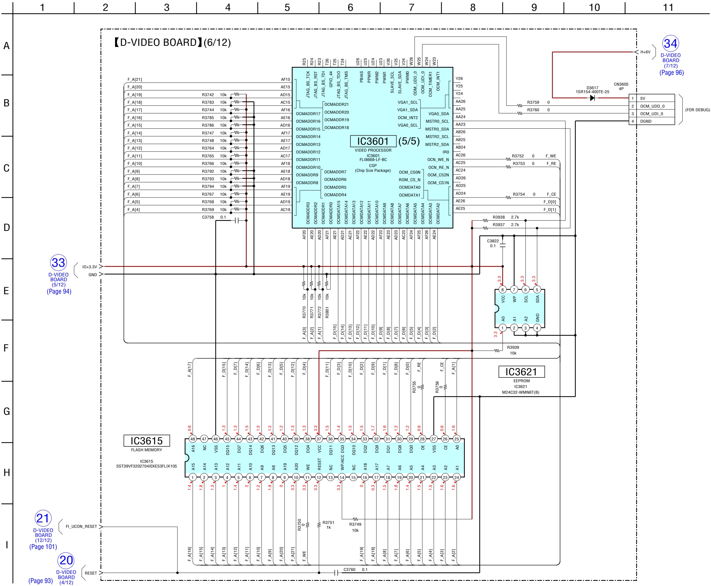
6-63. SCHEMATIC DIAGRAM – D-VIDEO Board (6/12) – • See page 141 for IC Pin Function Description.
