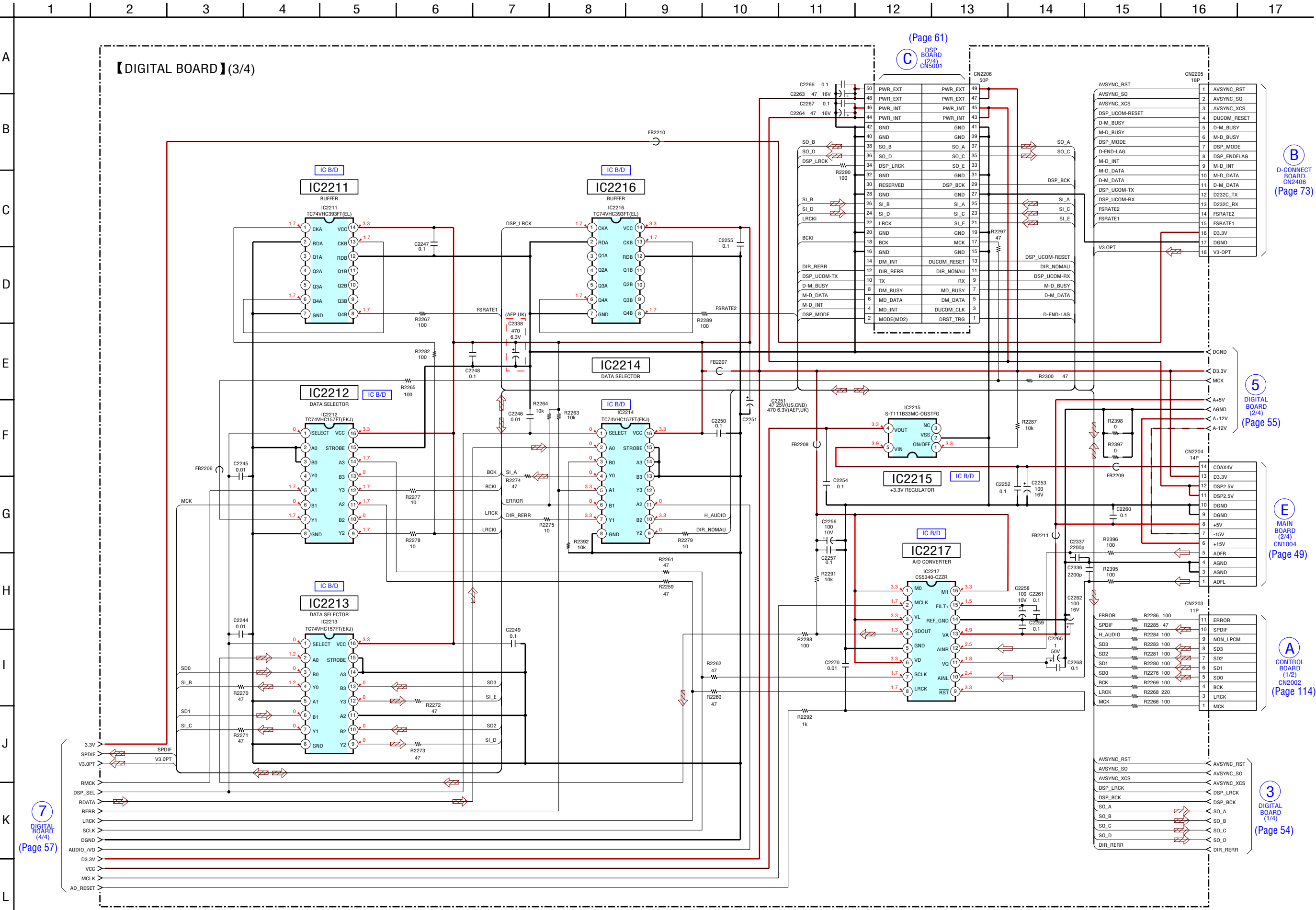
6-23. SCHEMATIC DIAGRAM – DIGITAL Board (3/4) – • See page 127 for IC Block Diagrams.
