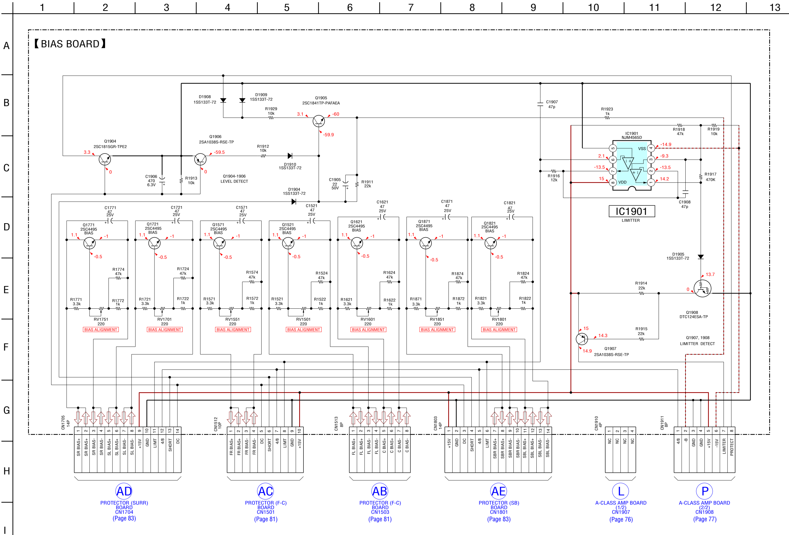
6-53. SCHEMATIC DIAGRAM – BIAS Board –
