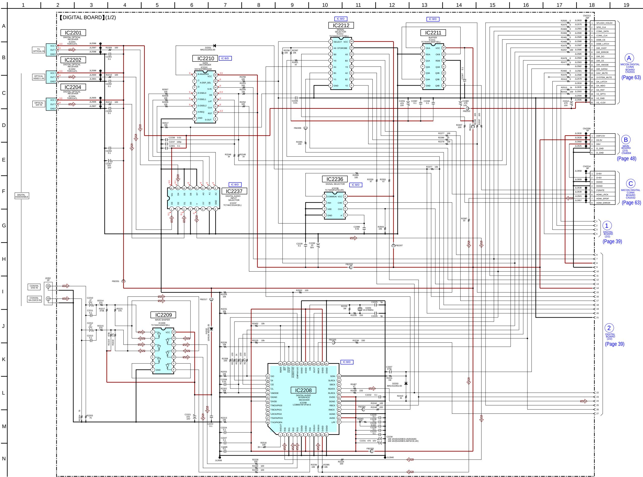
6-11. SCHEMATIC DIAGRAM - DIGITAL Board (1/2) - • See Page 76 for IC Block Diagrams.
