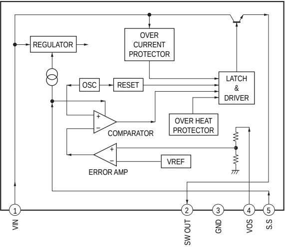
- DCDC CON Board - IC1401 SI-8050S-LF1101
