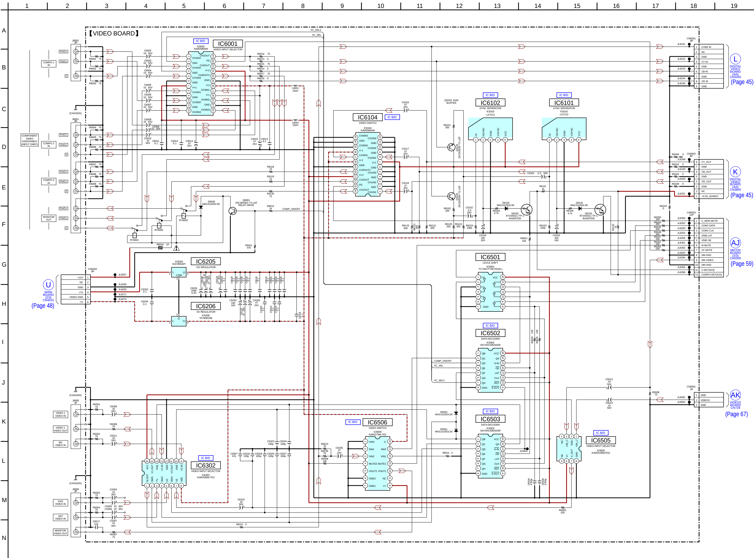
6-26. SCHEMATIC DIAGRAM - VIDEO Board - • See Page 76 for IC Block Diagrams.
