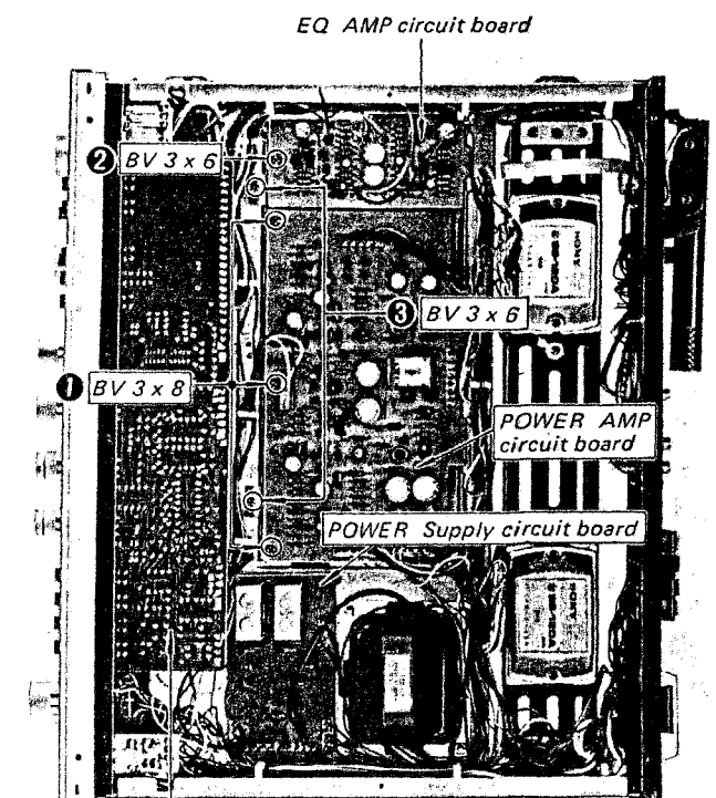
TONE CONTROL circuit board
