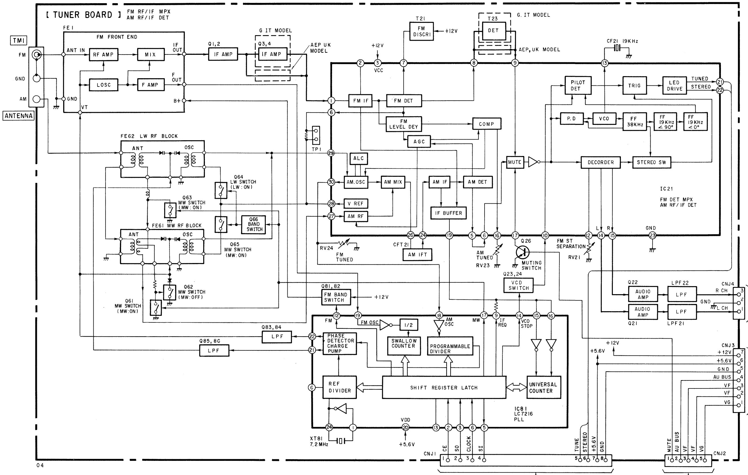
4-1. BLOCK DIAGRAM
