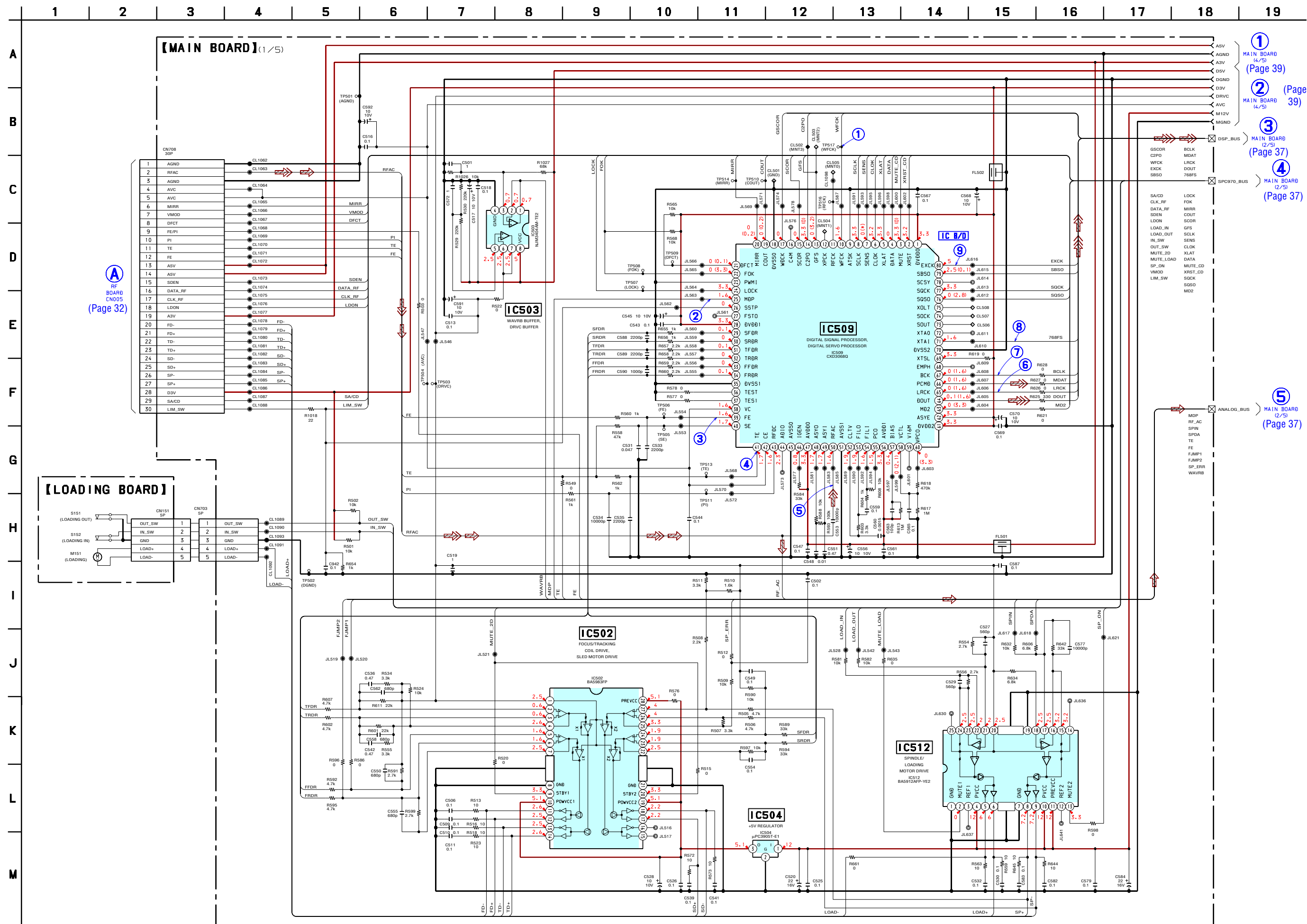
5-11. SCHEMATIC DIAGRAM – MAIN (1/5)/LOADING Boards – • See page 48 for Waveforms. • See page 51 for IC Block Diagram.
