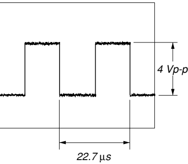
⑤ IC301 – 303 ⑤ (PLRCK) (CD Play mode)
