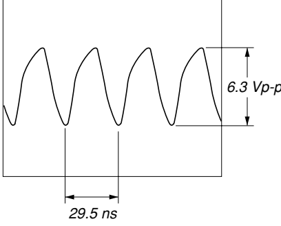
⑭ IC801 ⑩① (MCKI)
