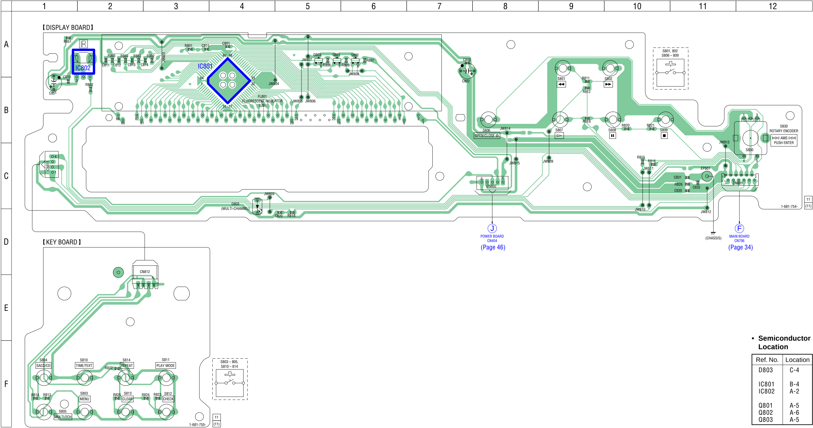
5-19. PRINTED WIRING BOARDS – DISPLAY/KEY Boards – • See page 31 for Circuit Boards Location.
