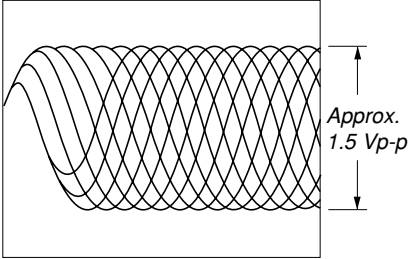
③ IC001 ⑥⑦ (RFAC) (CD Play mode)
