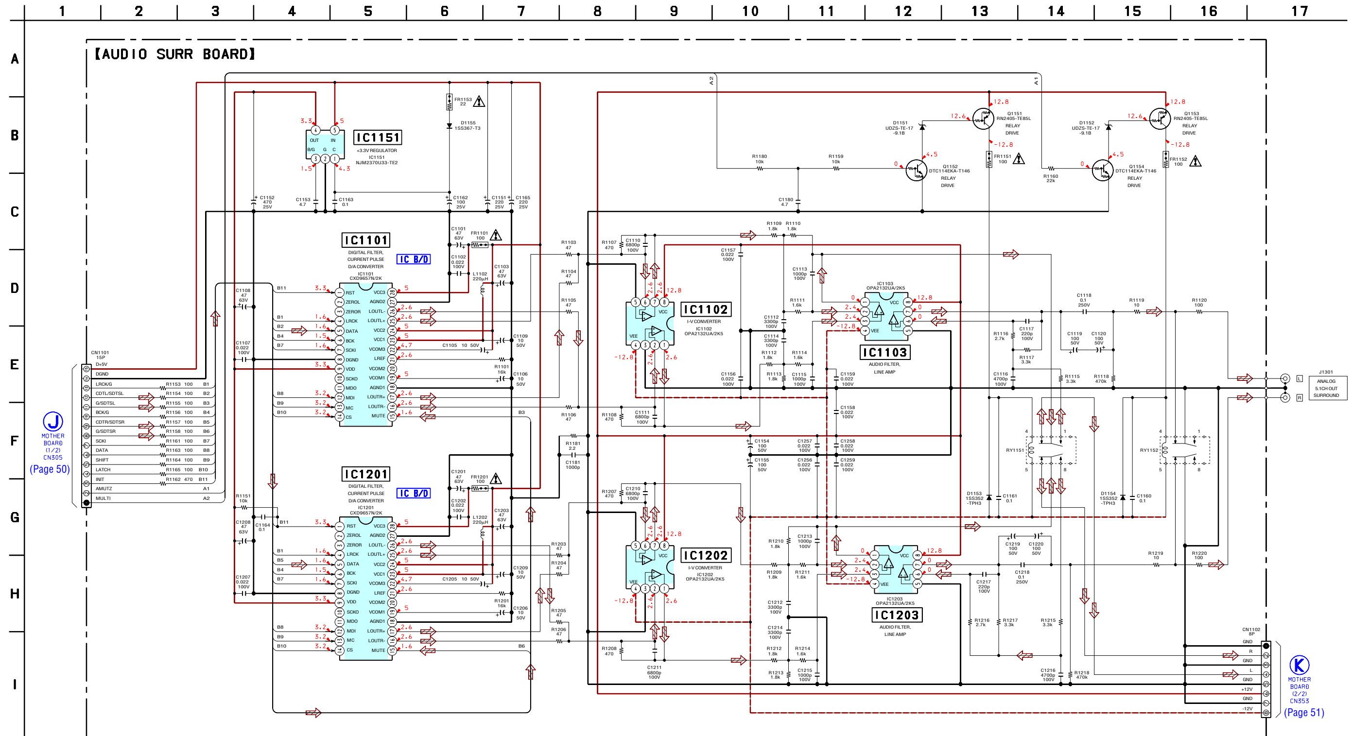
5-26. SCHEMATIC DIAGRAM – AUDIO SURR Board – • See page 70 for IC Block Diagrams.
