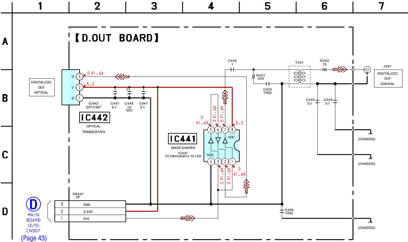
5-18. SCHEMATIC DIAGRAM – D.OUT Board –
