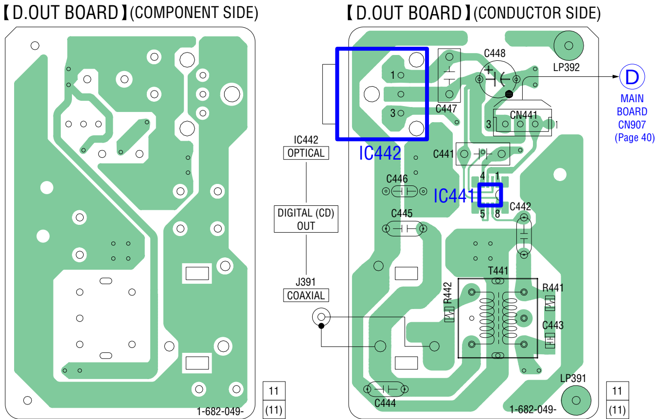
5-17. PRINTED WIRING BOARD – D.OUT Board – • See page 37 for Circuit Boards Location.
