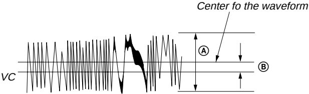
Traverse waveform
