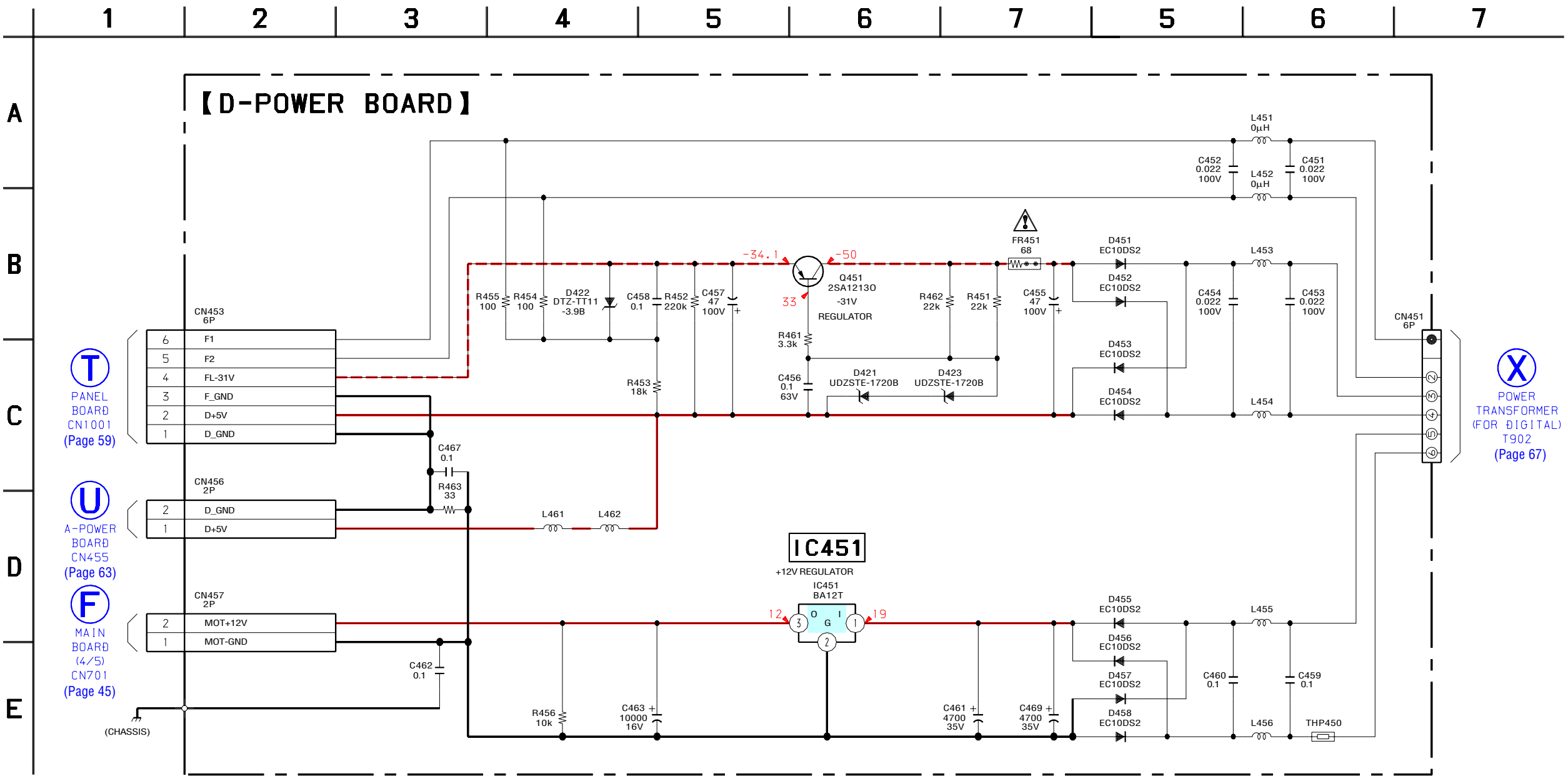
5-36. SCHEMATIC DIAGRAM – D-POWER Board –
