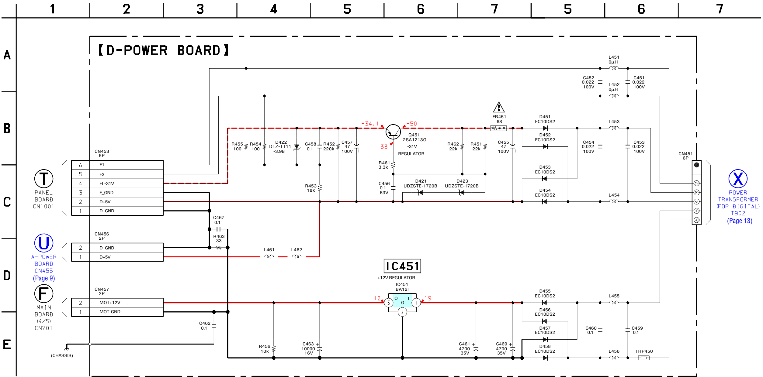
2-11. SCHEMATIC DIAGRAM – D-POWER Board –
