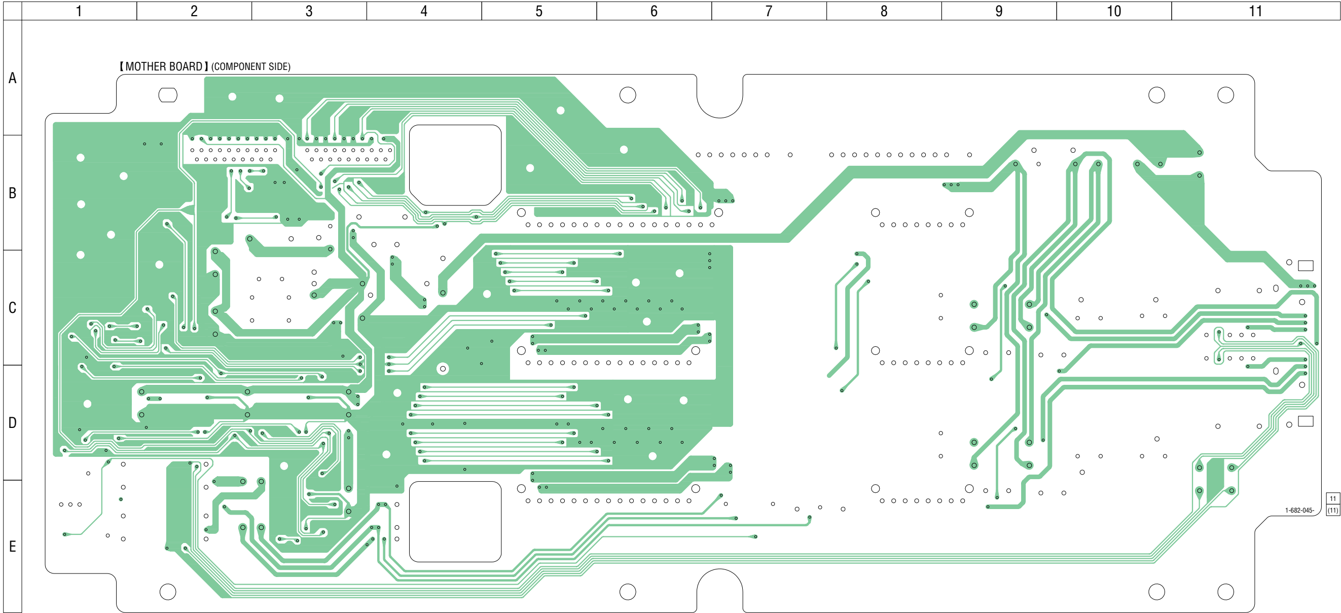
5-19. PRINTED WIRING BOARD – MOTHER Board (Component Side) – • See page 37 for Circuit Boards Location.
