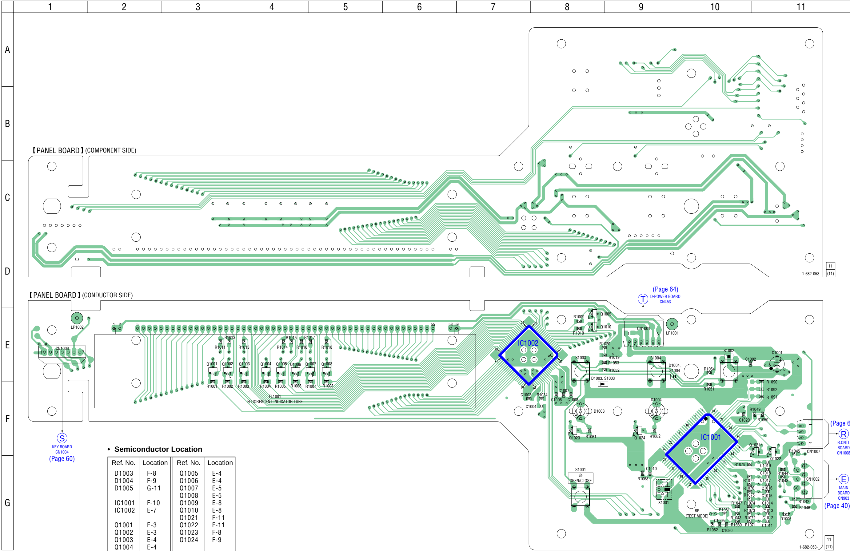
5-29. PRINTED WIRING BOARD – PANEL Board – • See page 37 for Circuit Boards Location.
