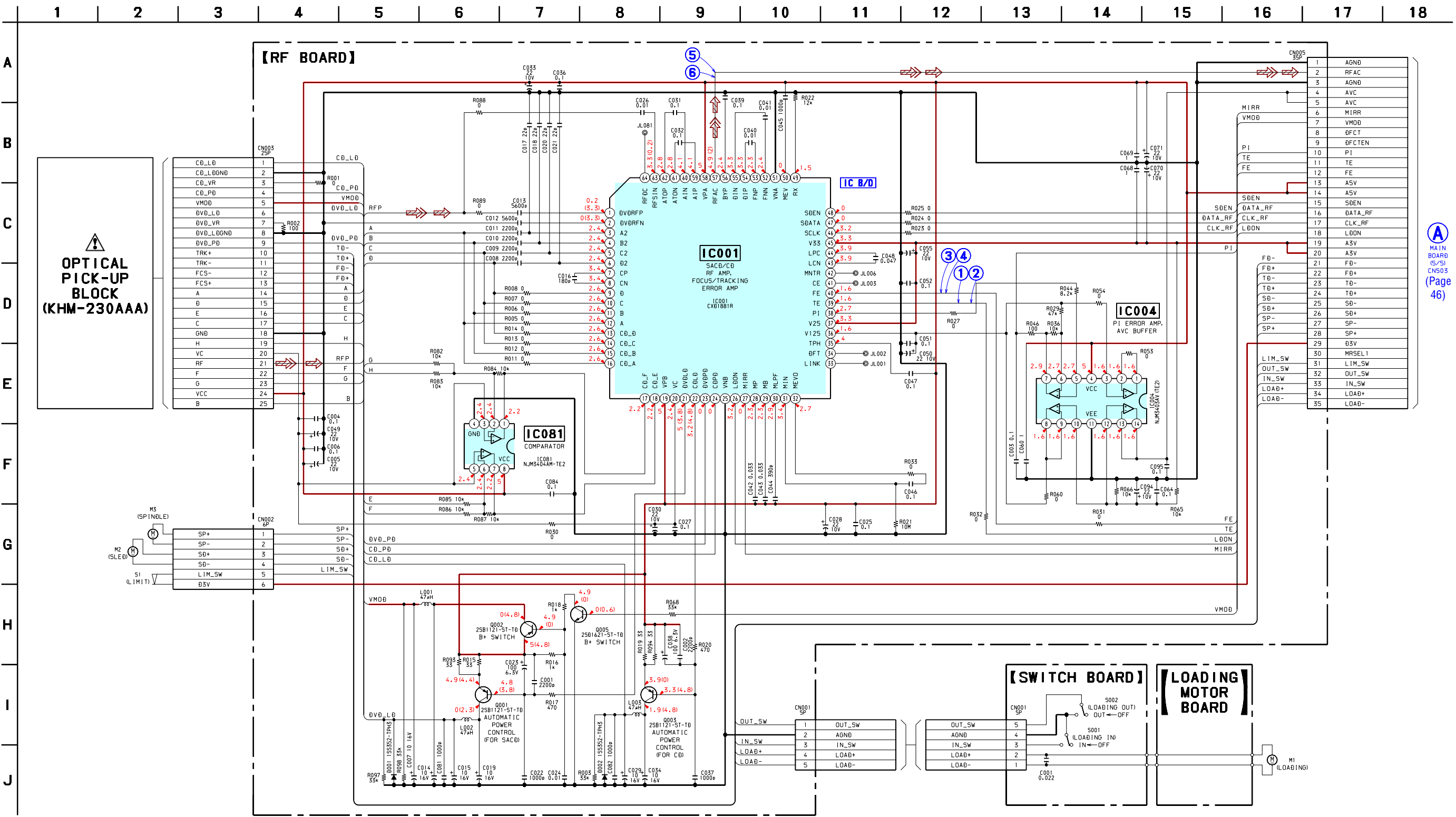
5-9. SCHEMATIC DIAGRAM – LOADING MOTOR/RF/SWITCH Boards – • See page 68 for Waveforms. • See page 70 for IC Block Diagram.
