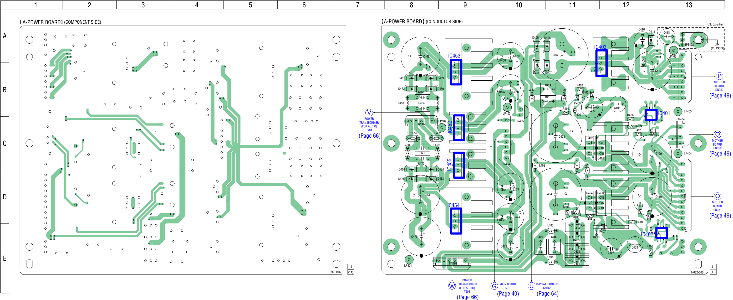
5-33. PRINTED WIRING BOARD – A-POWER Board – • See page 37 for Circuit Boards Location.
