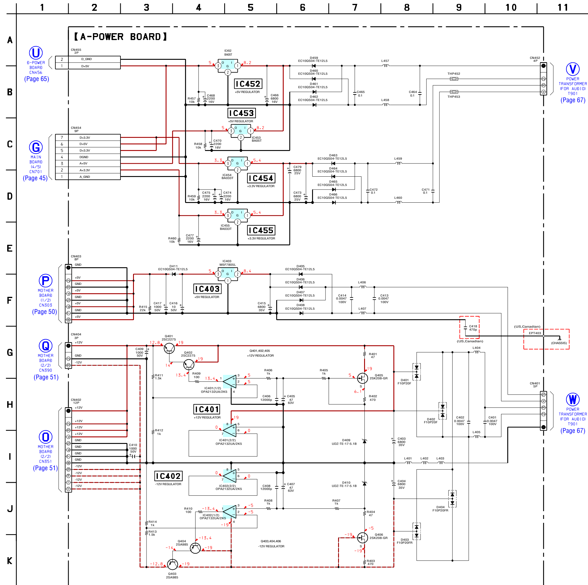
5-34. SCHEMATIC DIAGRAM – A-POWER Board –
