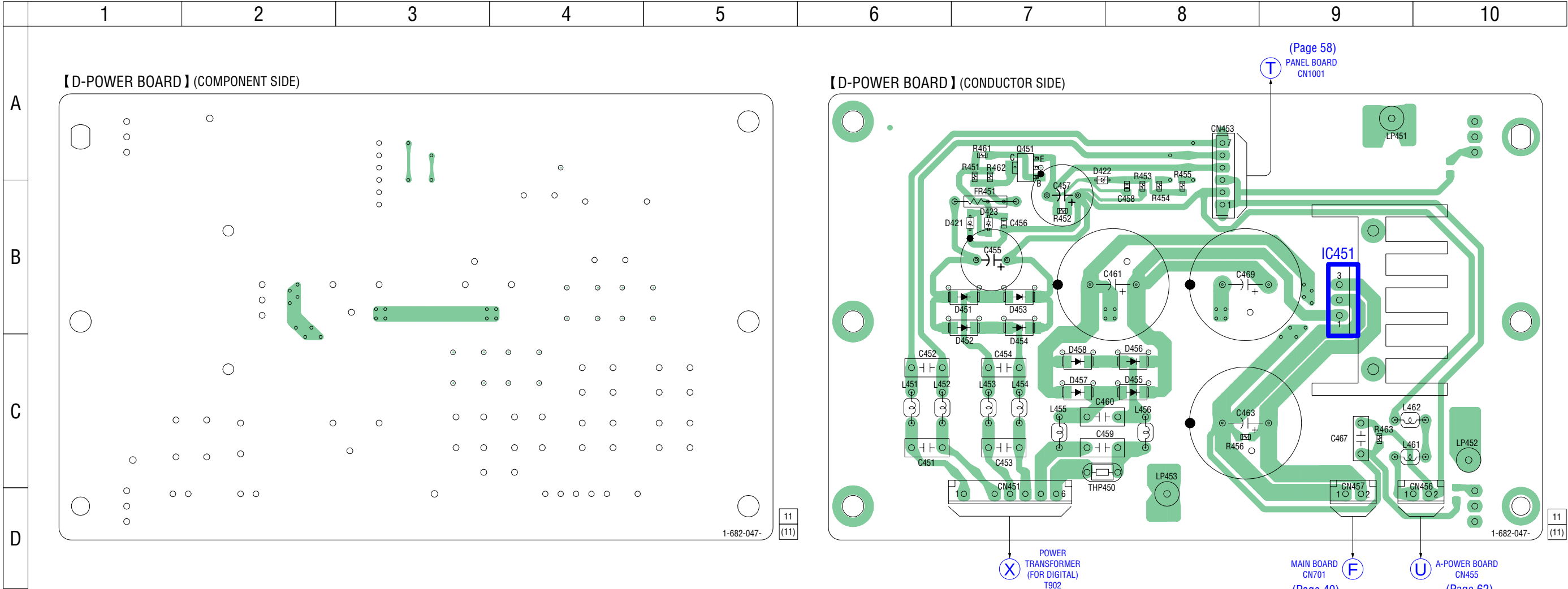
5-35. PRINTED WIRING BOARD – D-POWER Board – • See page 37 for Circuit Boards Location.
