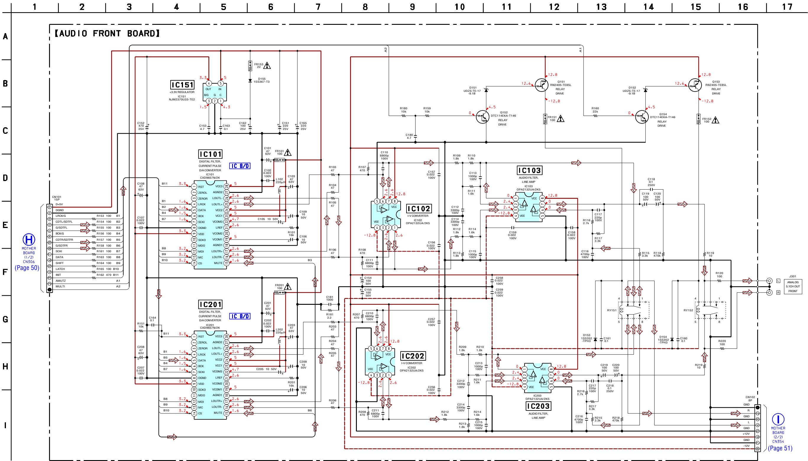
5-24. SCHEMATIC DIAGRAM – AUDIO FRONT Board – • See page 70 for IC Block Diagrams.
