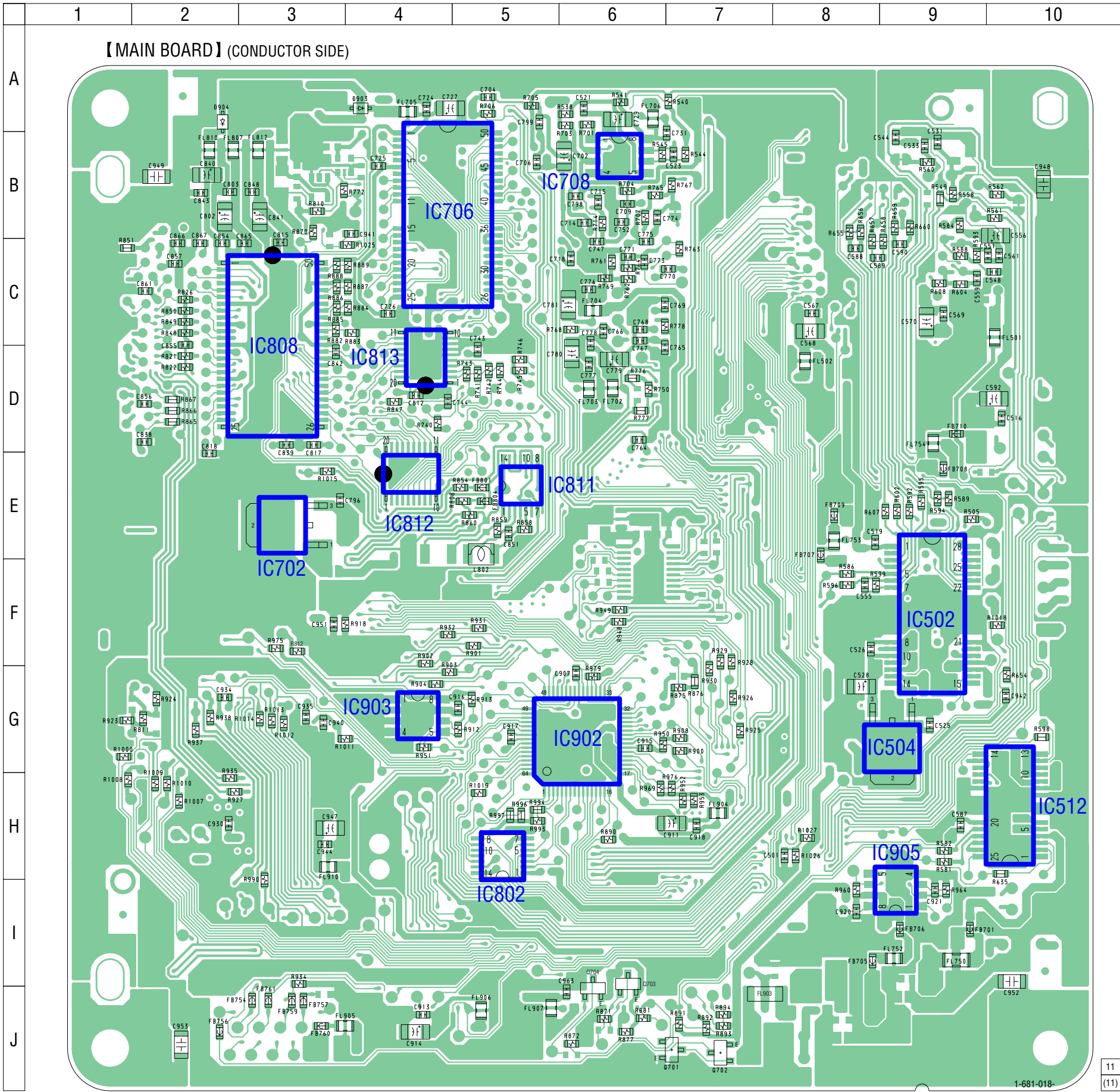
6-12. PRINTED WIRING BOARD – MAIN Board (Conductor Side) – • See page 35 for Circuit Boards Location.
