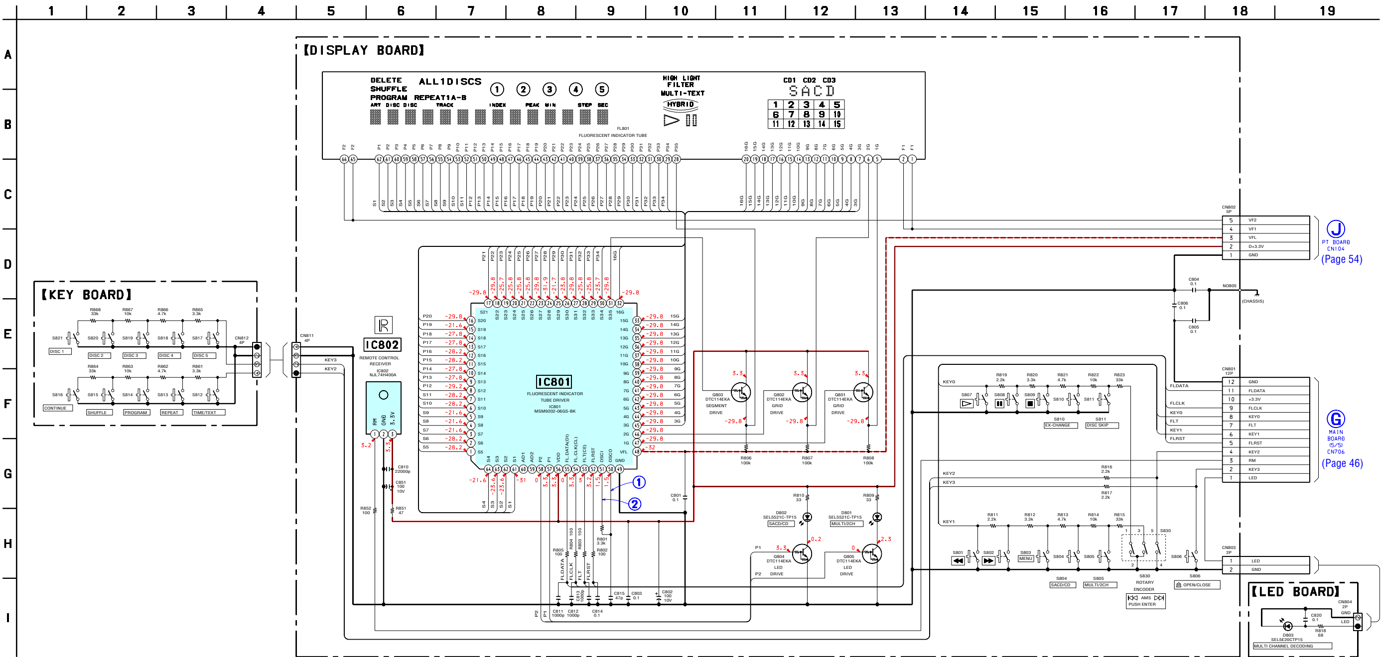
6-22. SCHEMATIC DIAGRAM – DISPLAY/KEY/LED Boards – • See page 55 for Waveforms.
