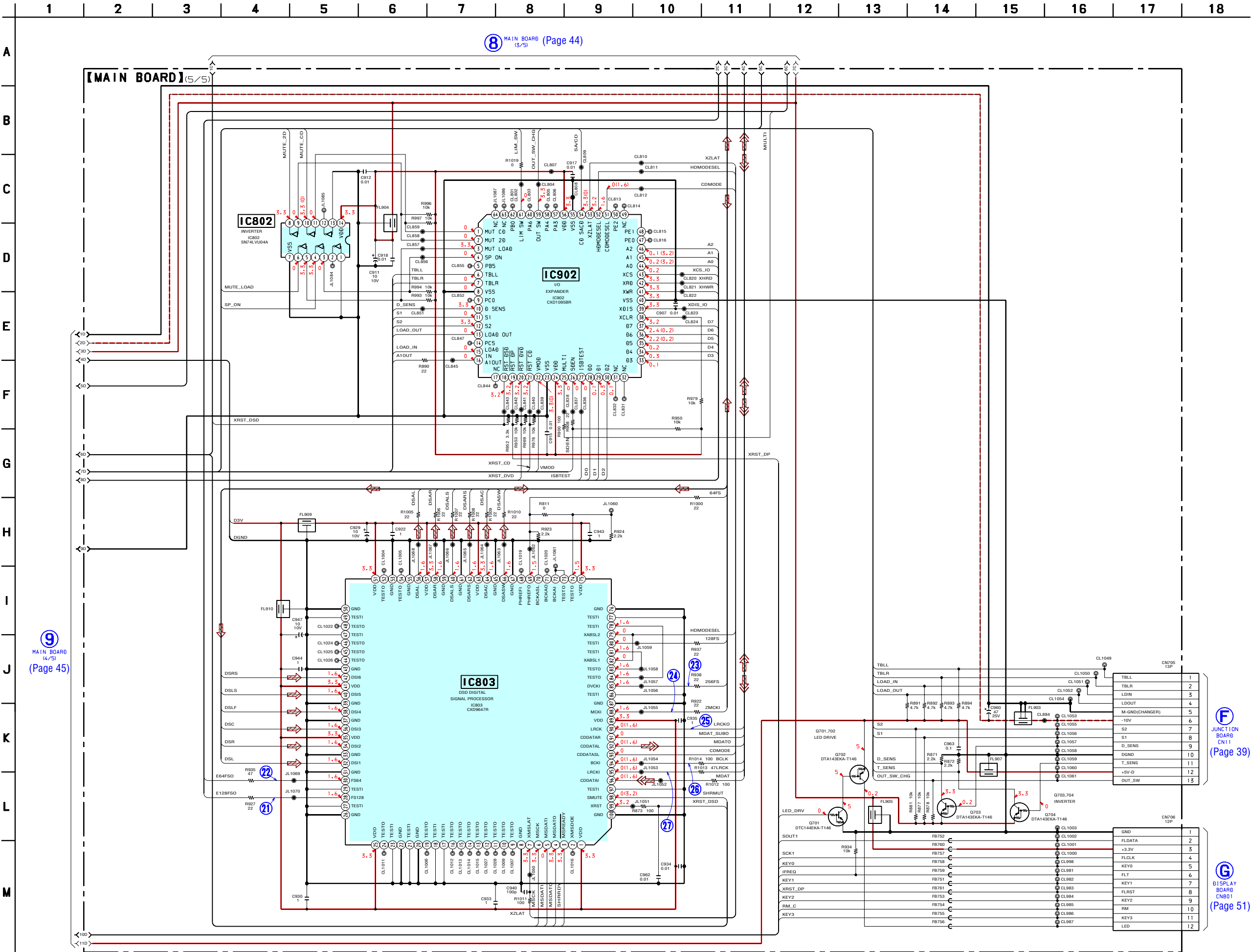
6-17. SCHEMATIC DIAGRAM – MAIN Board (5/5) – • See page 55 for Waveforms.
