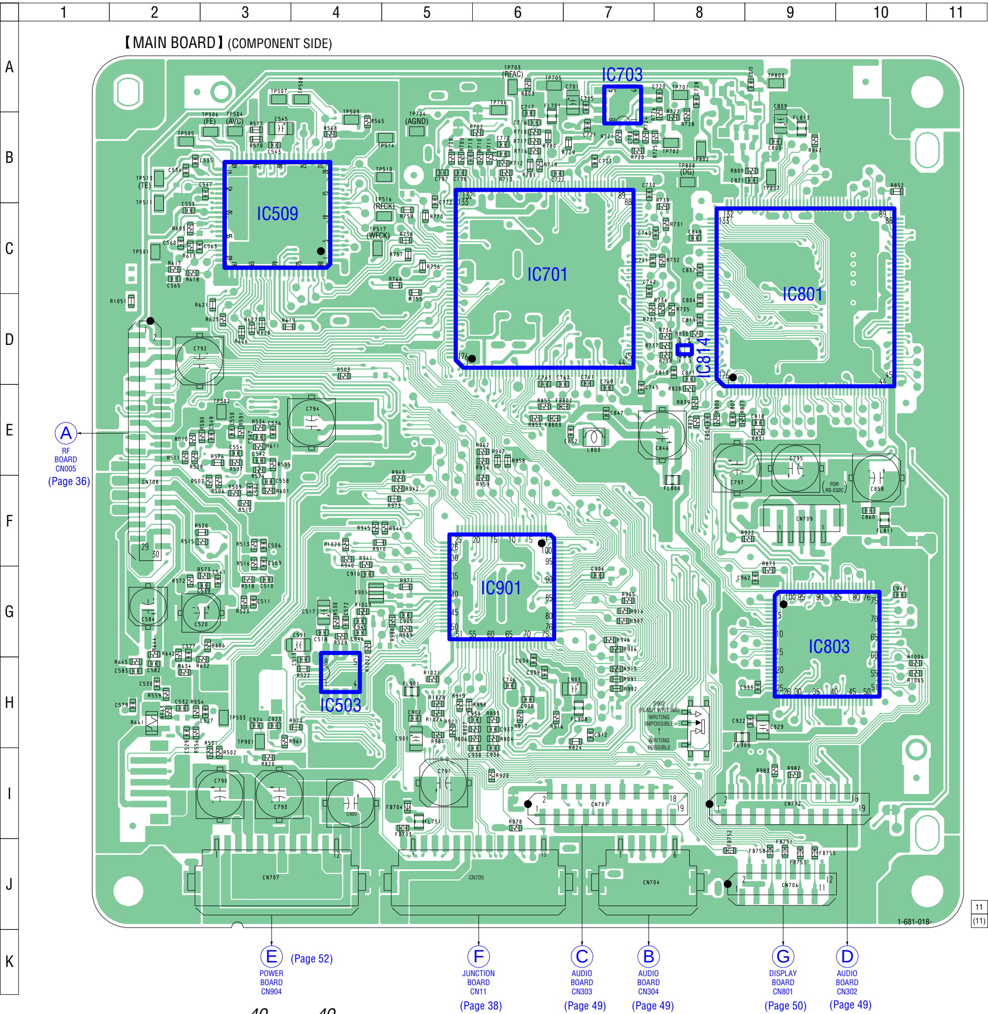
6-11. PRINTED WIRING BOARD – MAIN Board (Component Side) – • See page 35 for Circuit Boards Location.
