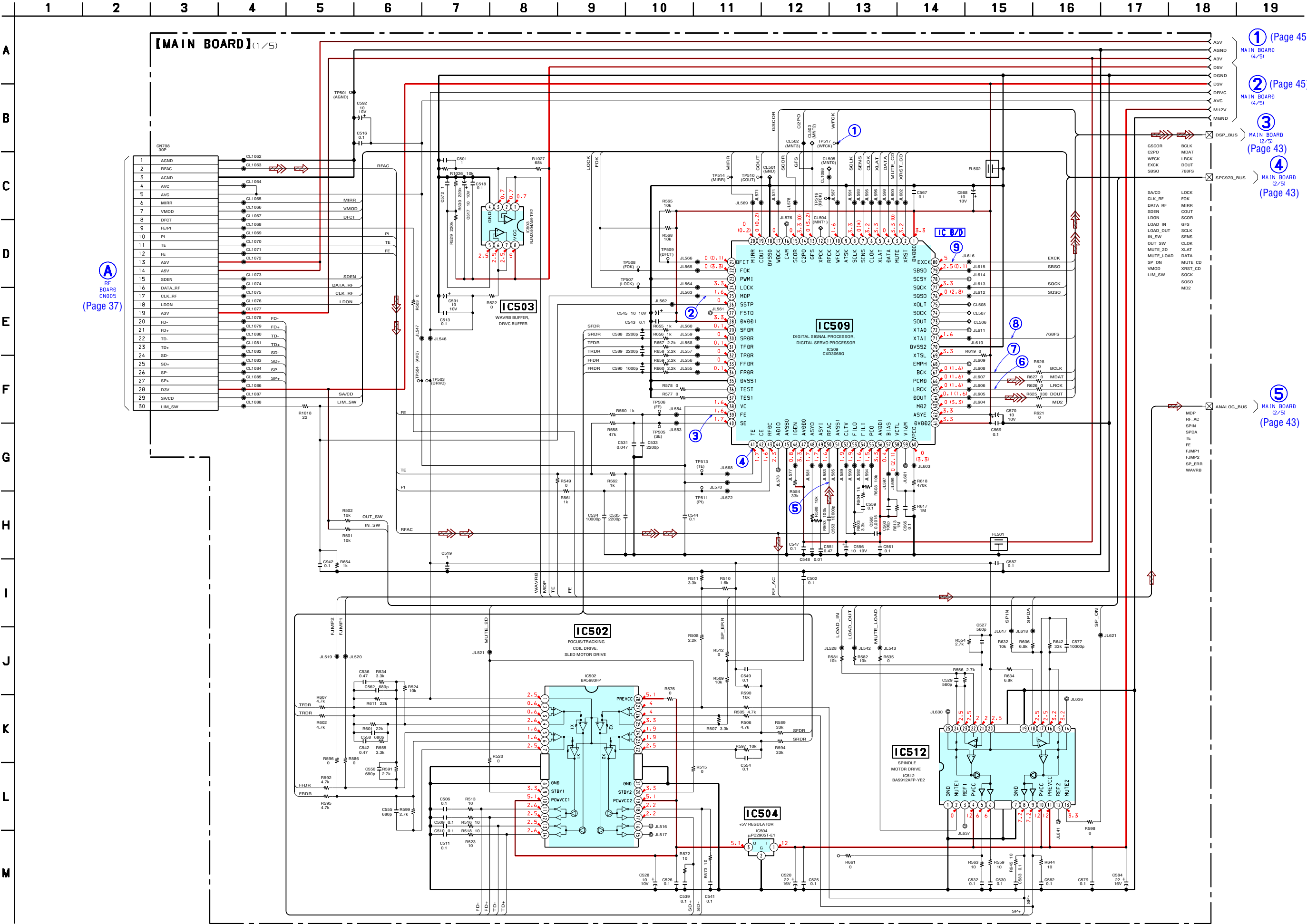
6-13. SCHEMATIC DIAGRAM – MAIN Board (1/5) – • See page 55 for Waveforms. • See page 59 for IC Block Diagram.
