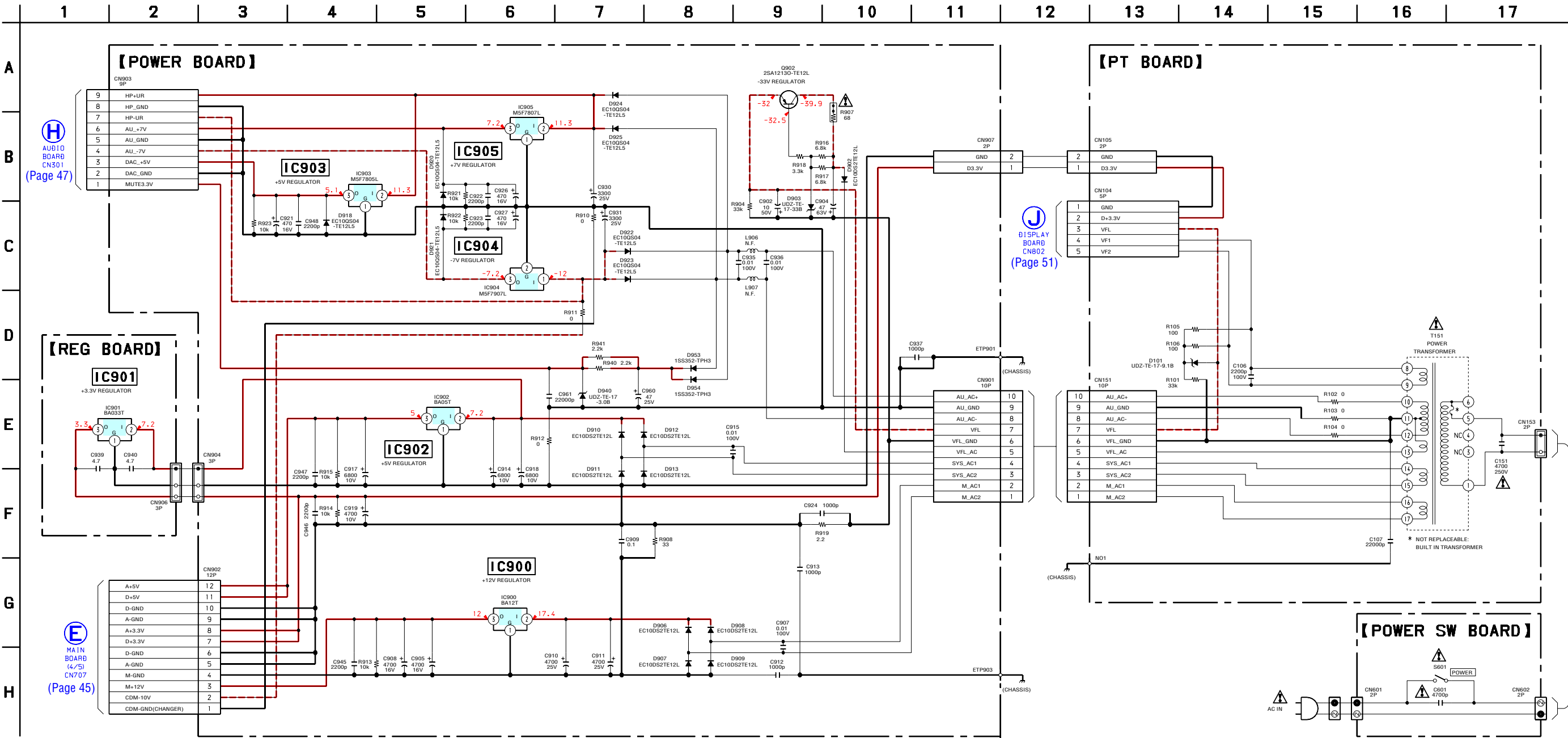
6-25. SCHEMATIC DIAGRAM – POWER/POWER SW/PT/REG Boards –
