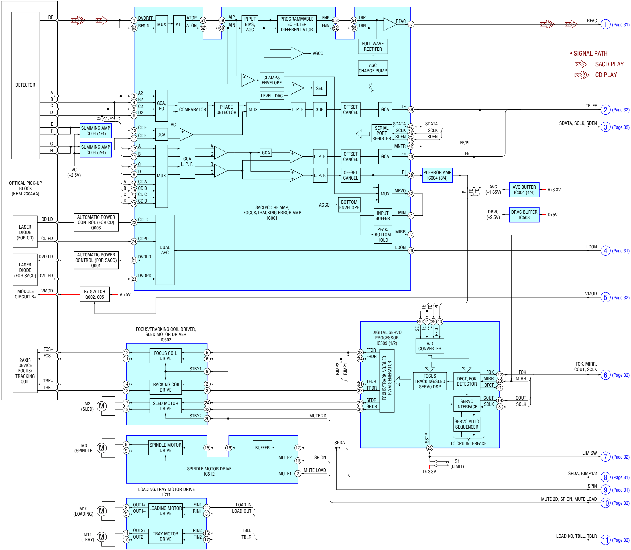
6-1. BLOCK DIAGRAM – RF/SERVO Section –
