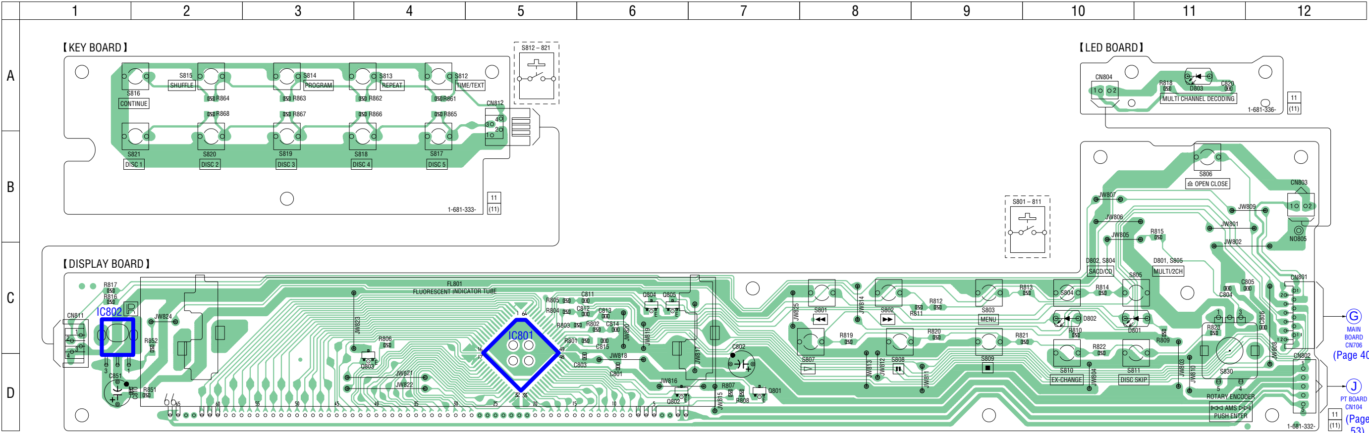
6-21. PRINTED WIRING BOARDS – DISPLAY/KEY/LED Boards – • See page 35 for Circuit Boards Location.
