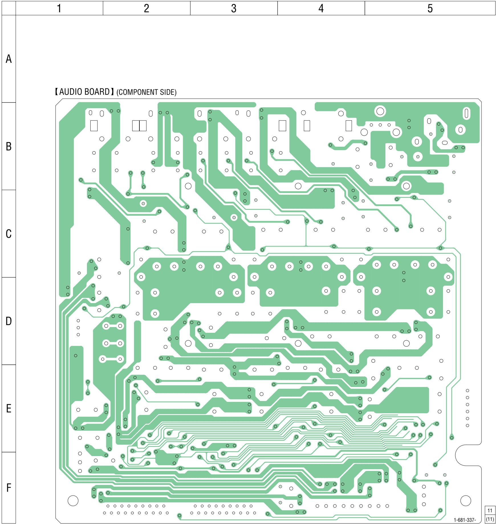
6-19. PRINTED WIRING BOARD – AUDIO Board (Component Side) – • See page 35 for Circuit Boards Location.
