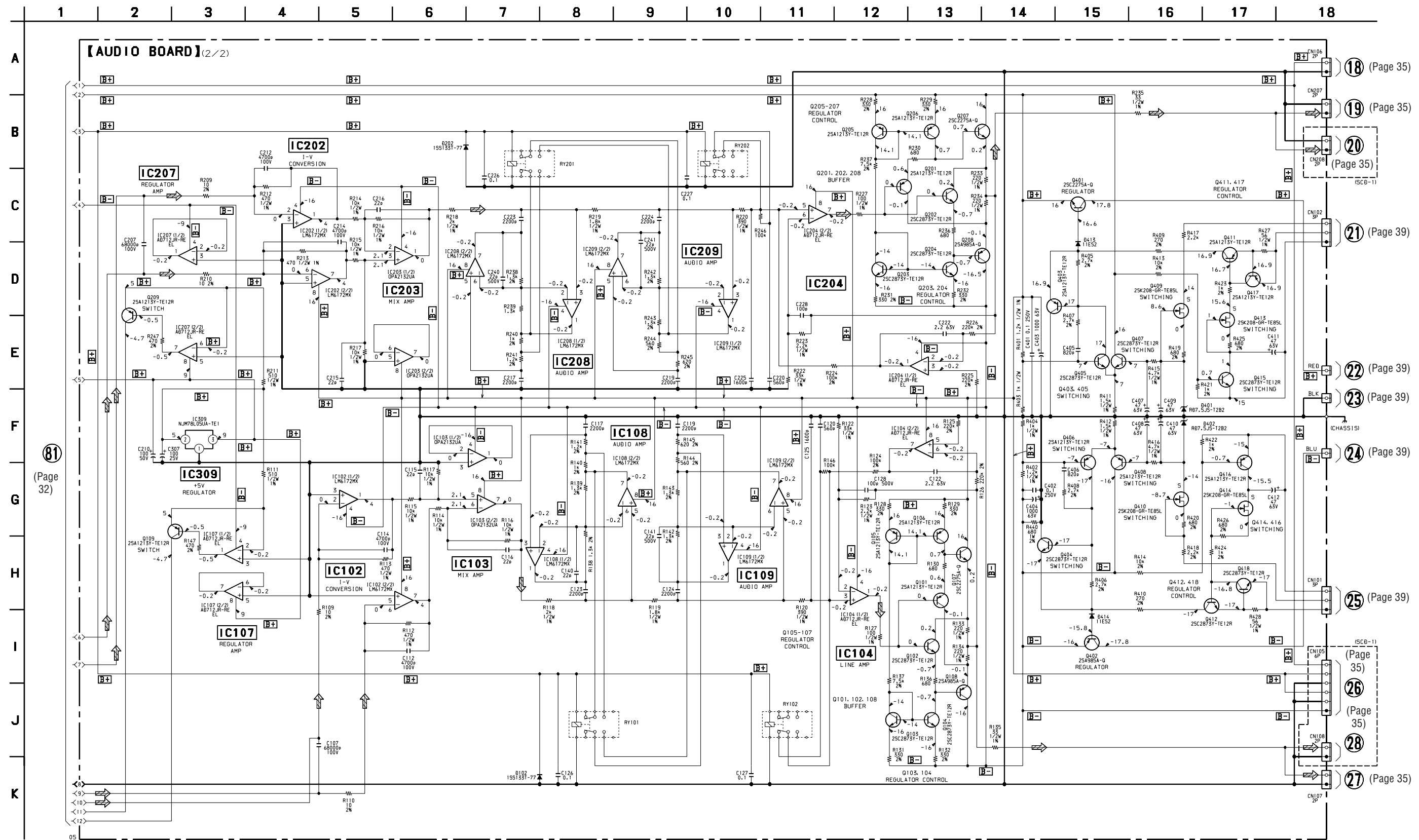
7-17. SCHEMATIC DIAGRAM – AUDIO Board (2/2) – • See page 40 for Waveforms.
