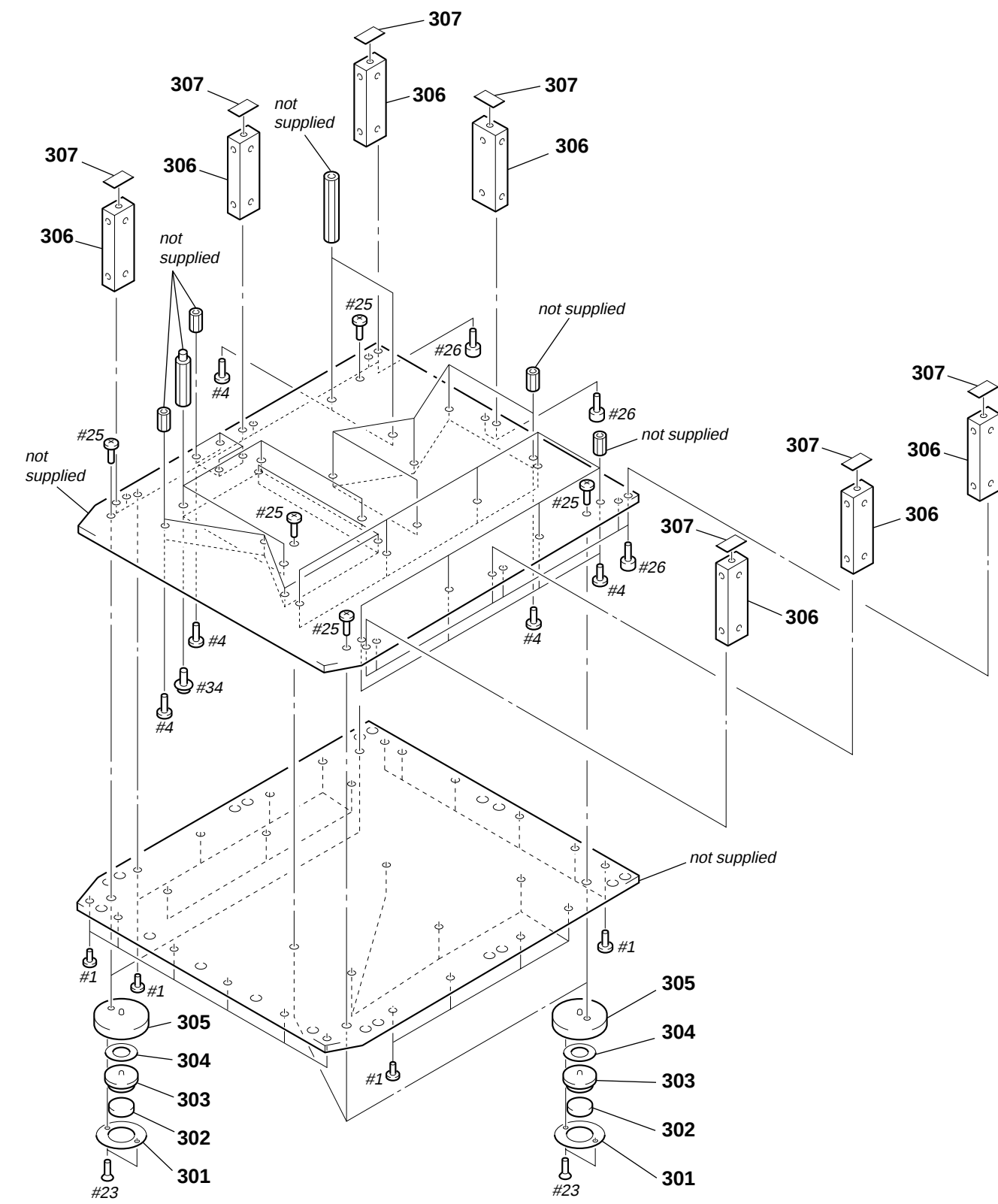
(7) CHASSIS SECTION (SCD-1)
