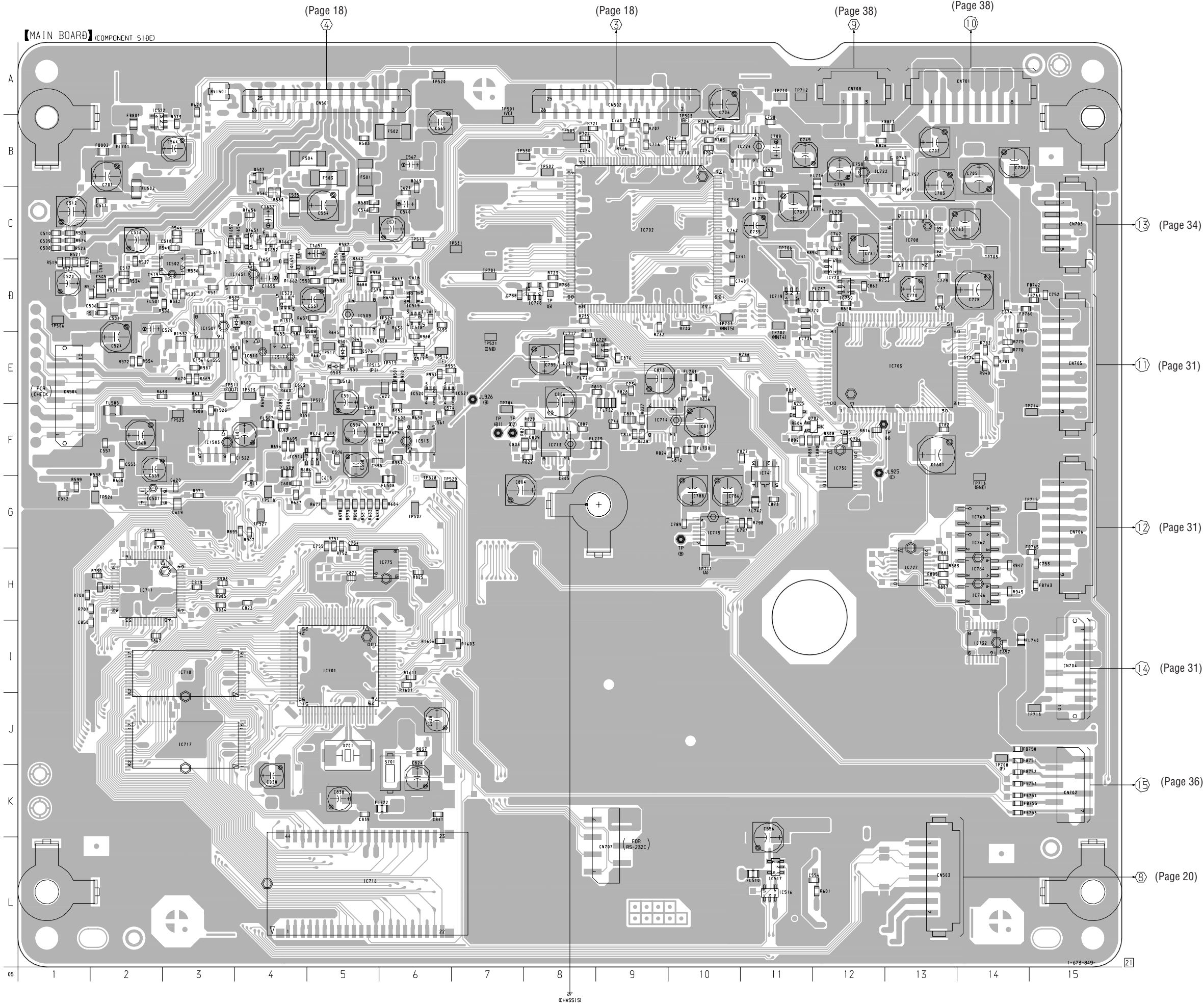
7-6. PRINTED WIRING BOARD – MAIN Board (component side) – • See page 17 for Circuit Boards Location.
