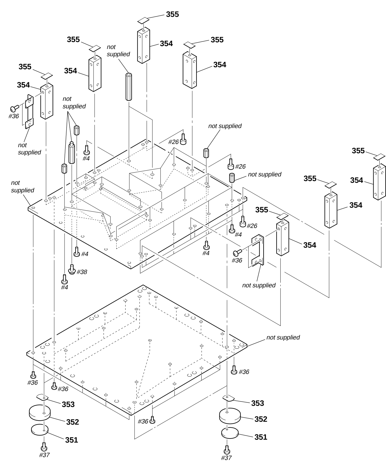
(8) CHASSIS SECTION (SCD-777ES)
