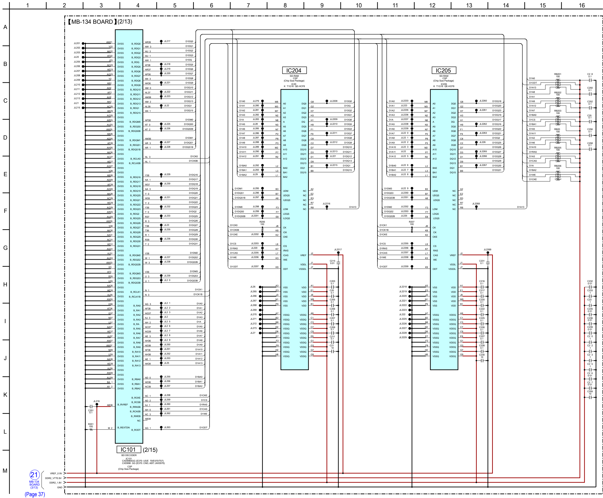
5-8. SCHEMATIC DIAGRAM - MB-134 Board (2/13) - • See page 77 for IC Pin Function Description.
