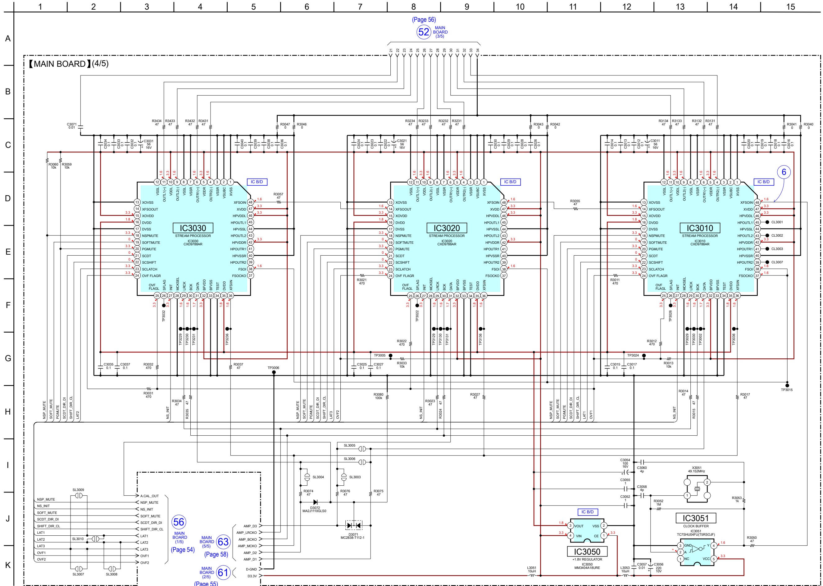
5-29. SCHEMATIC DIAGRAM - MAIN Board (4/5) - • See page 60 for waveforms. • See page 67 for IC Block Diagrams.
