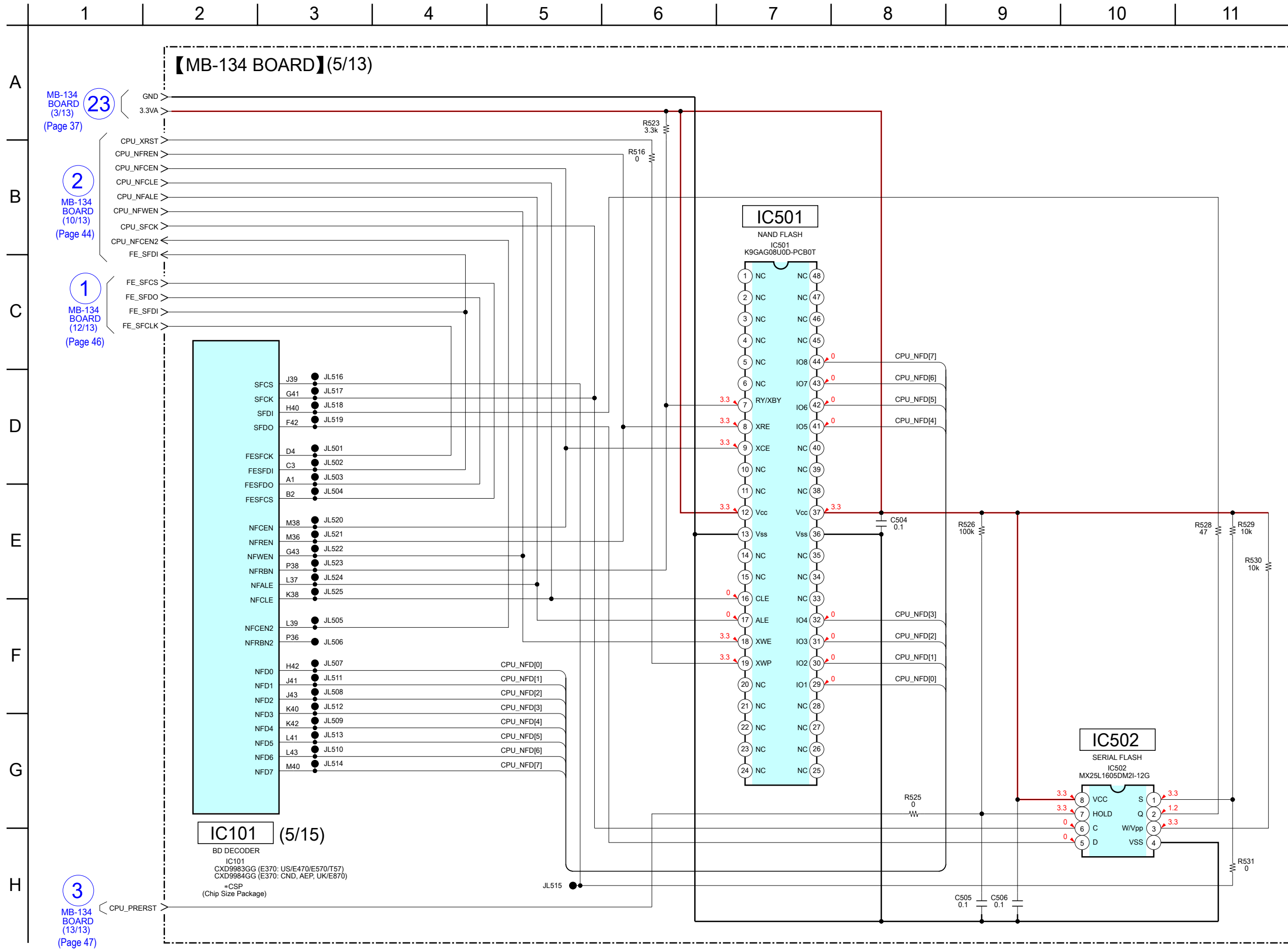
5-11. SCHEMATIC DIAGRAM - MB-134 Board (5/13) - • See page 77 for IC Pin Function Description.
