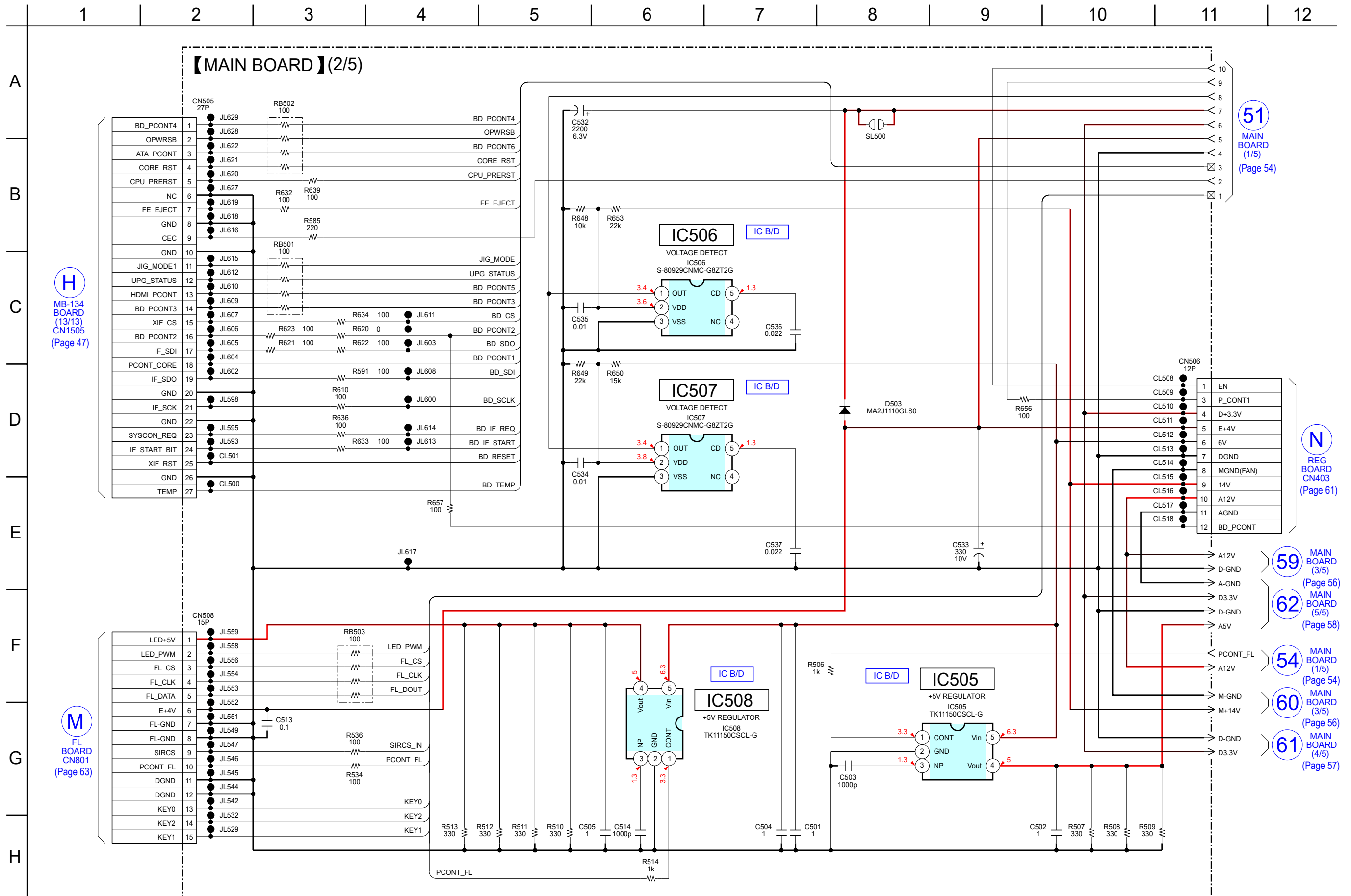
5-27. SCHEMATIC DIAGRAM - MAIN Board (2/5) - • See page 67 for IC Block Diagrams.
