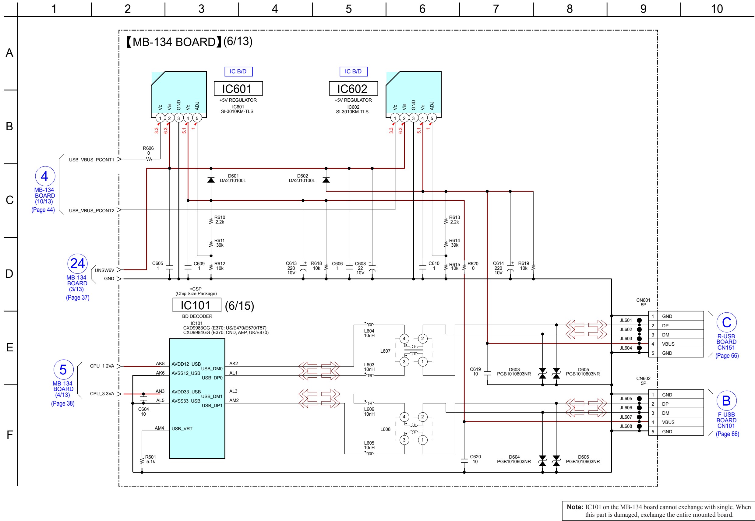
5-12. SCHEMATIC DIAGRAM - MB-134 Board (6/13) - • See page 67 for IC Block Diagrams. • See page 77 for IC Pin Function Description.
