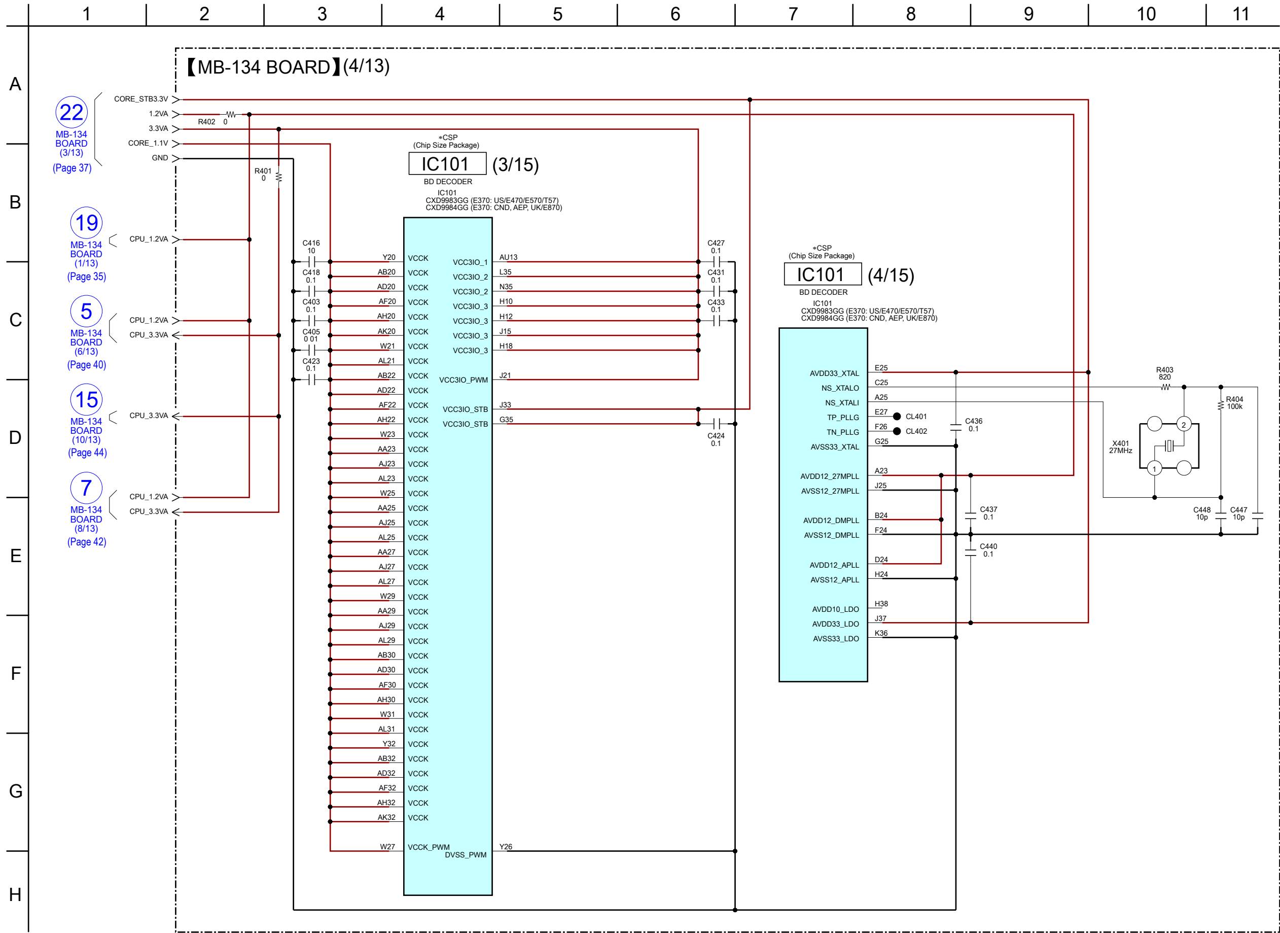
5-10. SCHEMATIC DIAGRAM - MB-134 Board (4/13) - • See page 77 for IC Pin Function Description.
