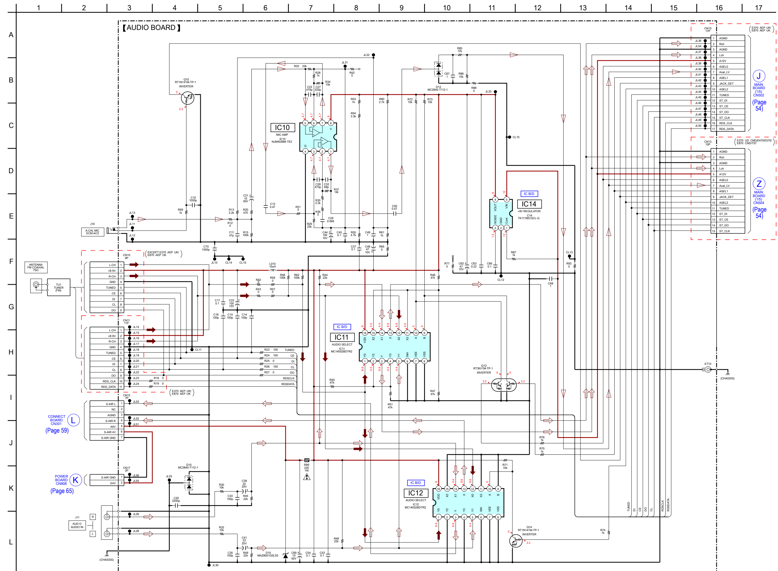
5-23. SCHEMATIC DIAGRAM - AUDIO Board - • See page 67 for IC Block Diagrams.
