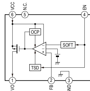
IC1451 BD35630HFV-TR
