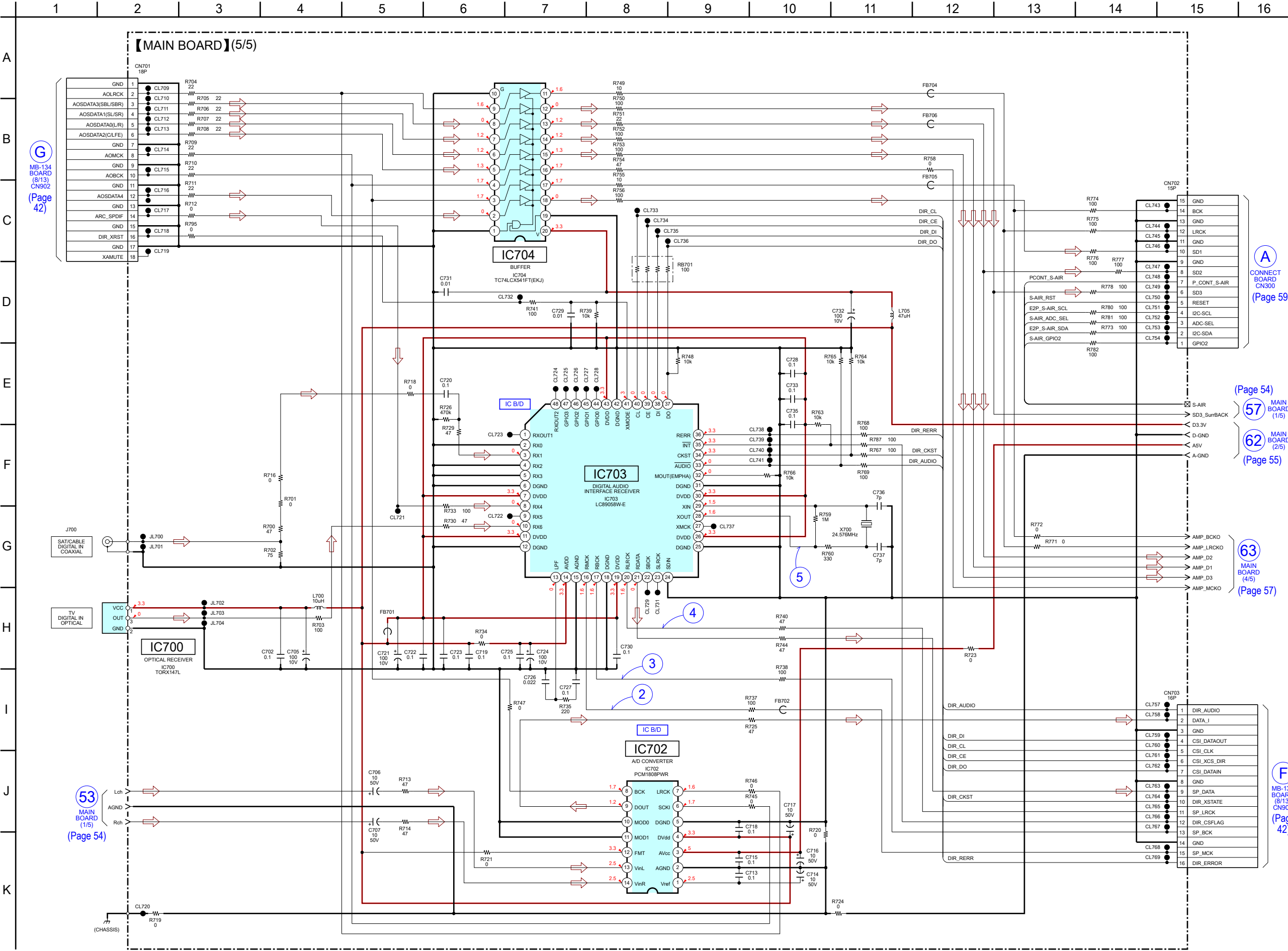
5-30. SCHEMATIC DIAGRAM - MAIN Board (5/5) - • See page 60 for waveforms. • See page 67 for IC Block Diagrams.
