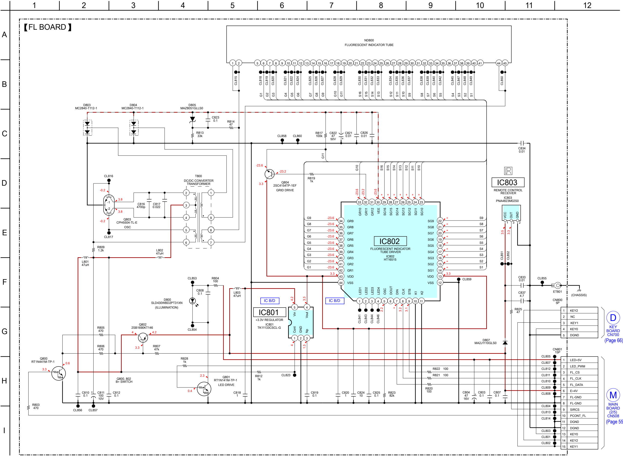
5-36. SCHEMATIC DIAGRAM - FL Board - • See page 67 for IC Block Diagrams.
