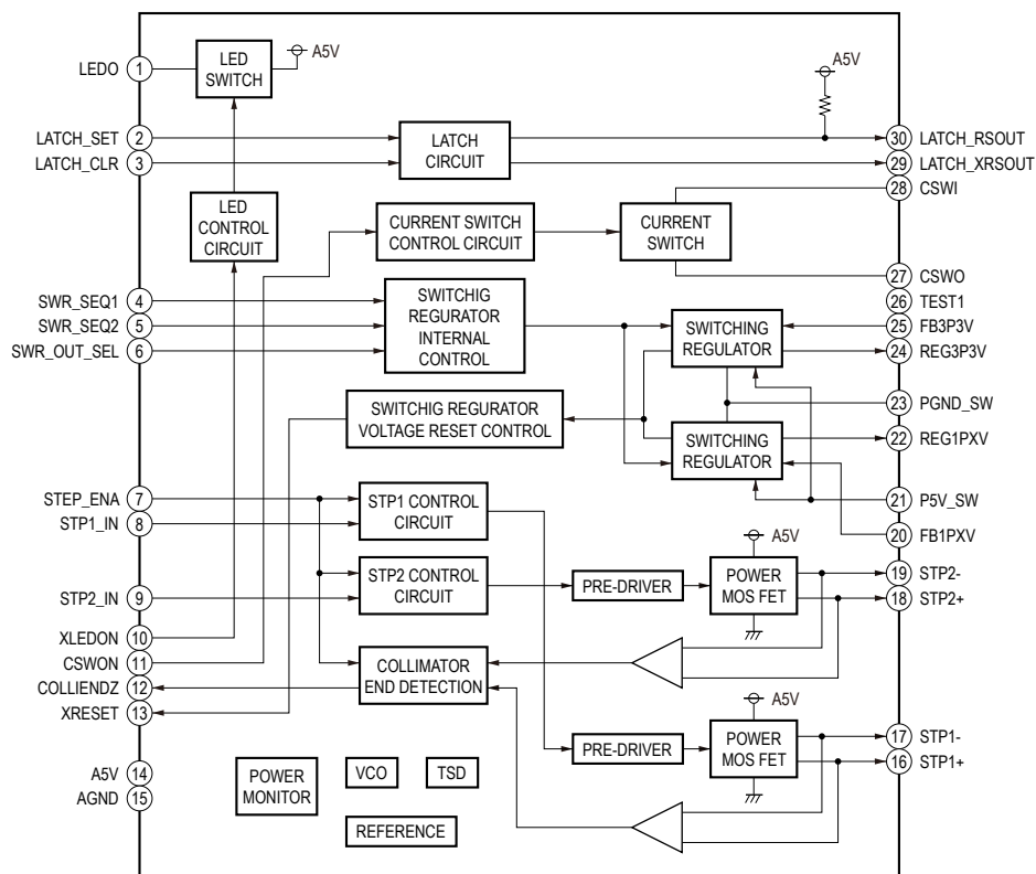
IC2301 TPIC1391DBTRG4
