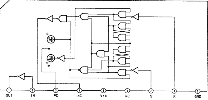
IC505 TC5081AP
