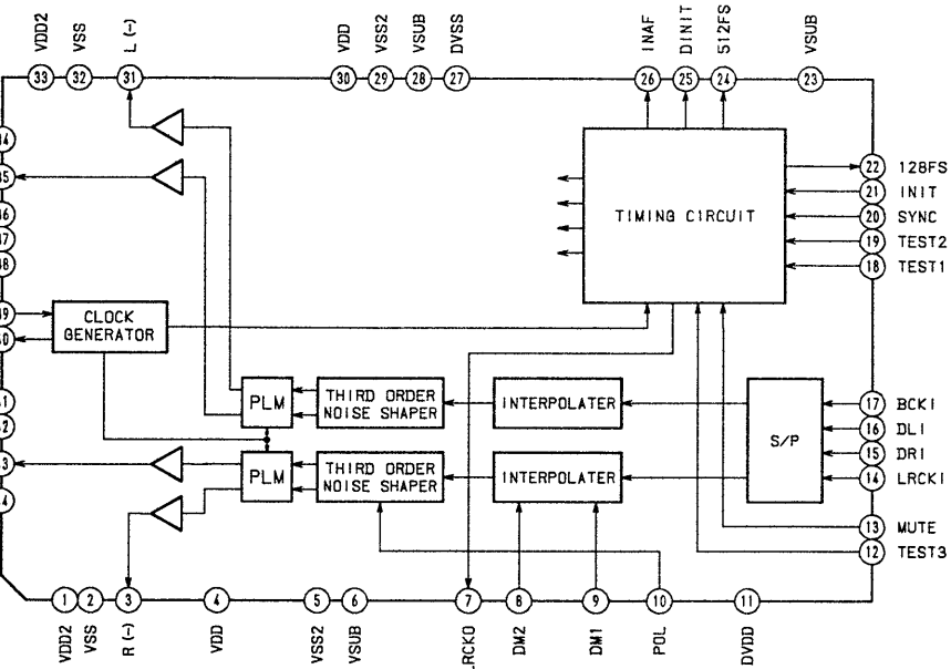
IC504 CXD2552
