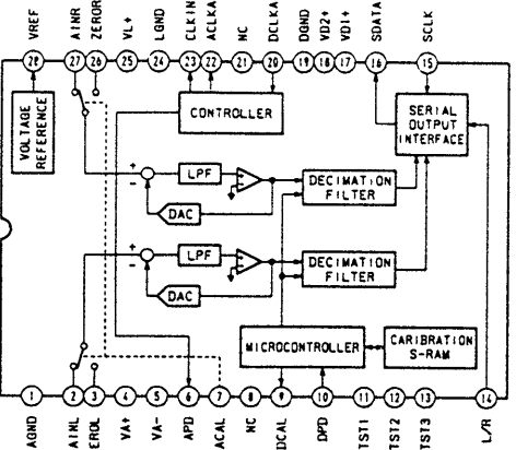
IC522 CS5326-KP
