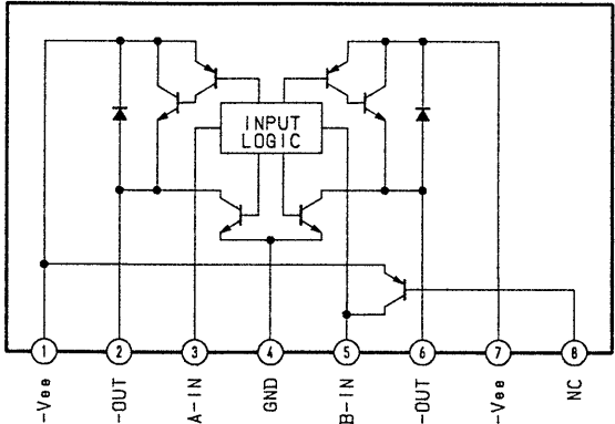
IC319 MB3763PS
