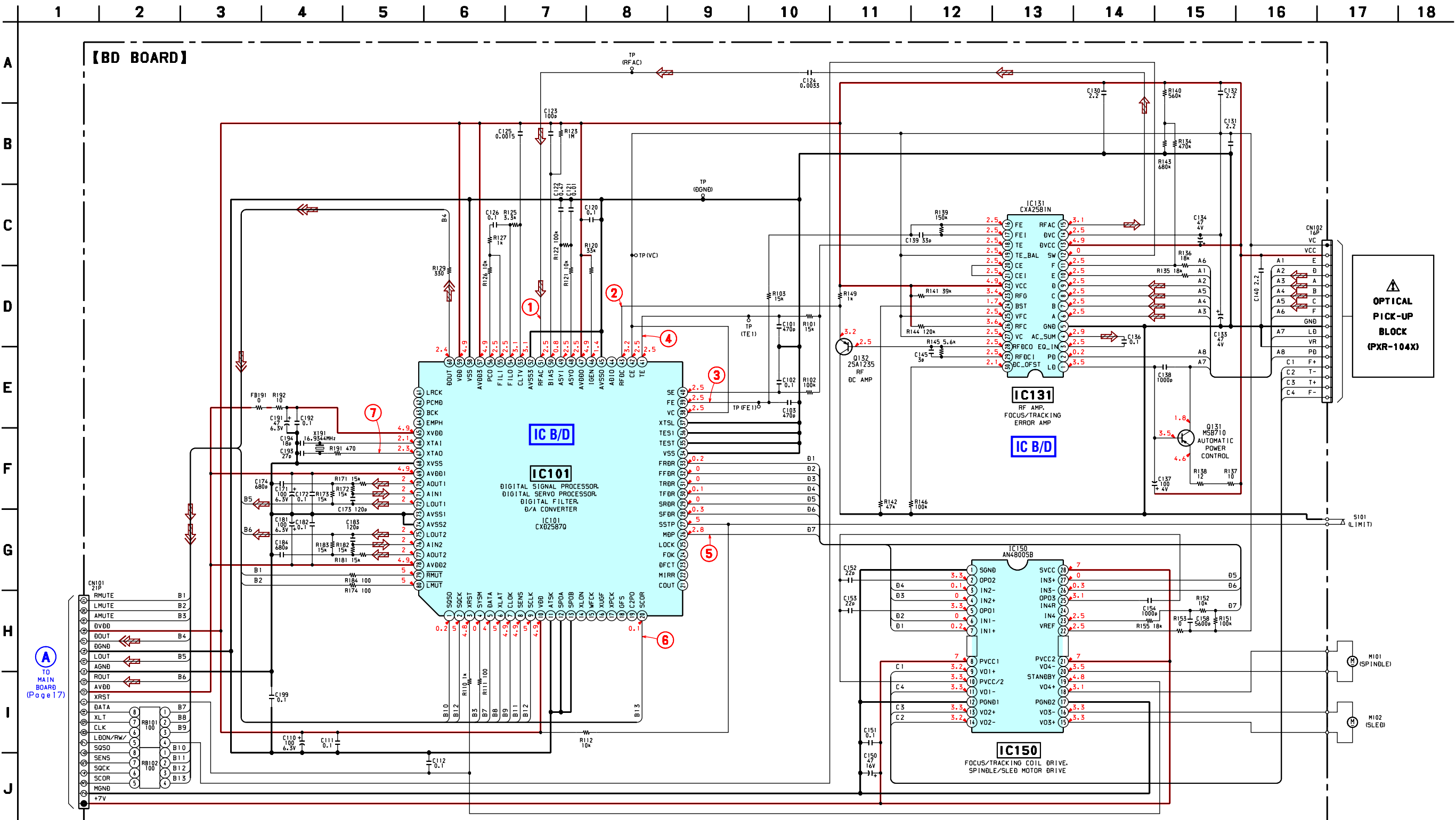
6-5. SCHEMATIC DIAGRAM BD SECTION • See page 21,22 for IC Block Diagrams. • See page 13 for waveforms.
