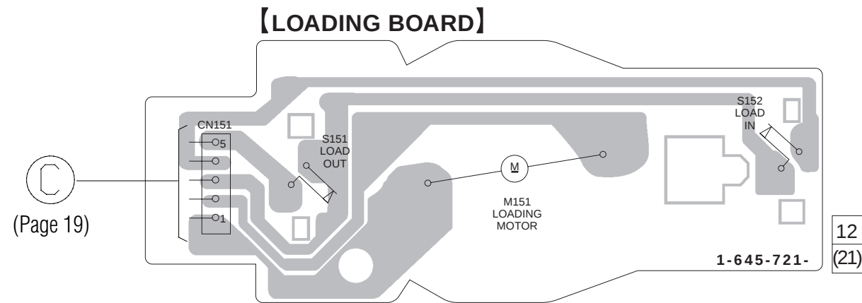
6-9. PRINTED WIRING BOARD – LOADING MOTOR SECTION – • See page 13 for Circuit Boards Location.
