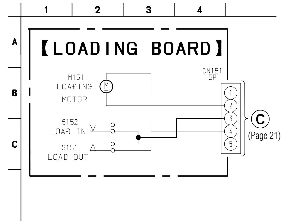
6-8. SCHEMATIC DIAGRAM – LOADING MOTOR SECTION –
