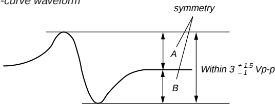
S-curve waveform
