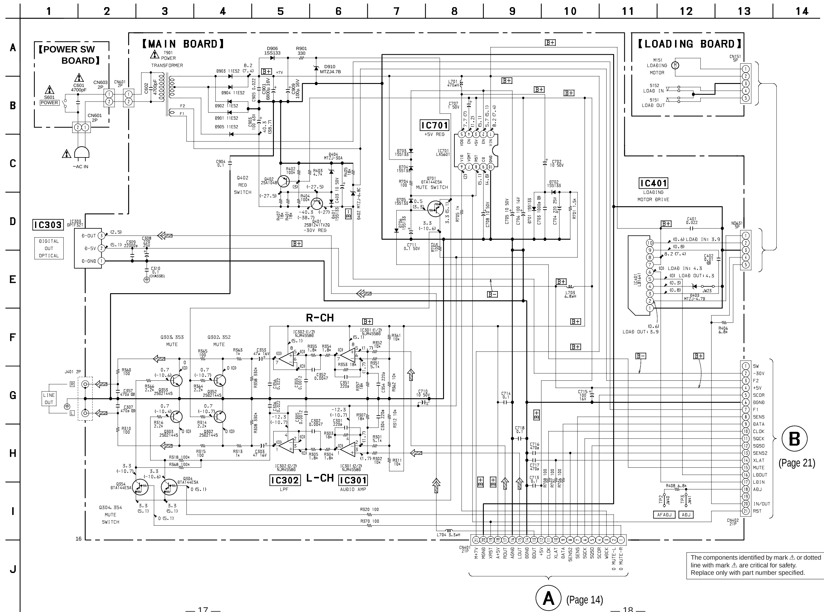
6-5. SCHEMATIC DIAGRAM — MAIN SECTION — • Refer to page 31 for IC Block Diagrams.
