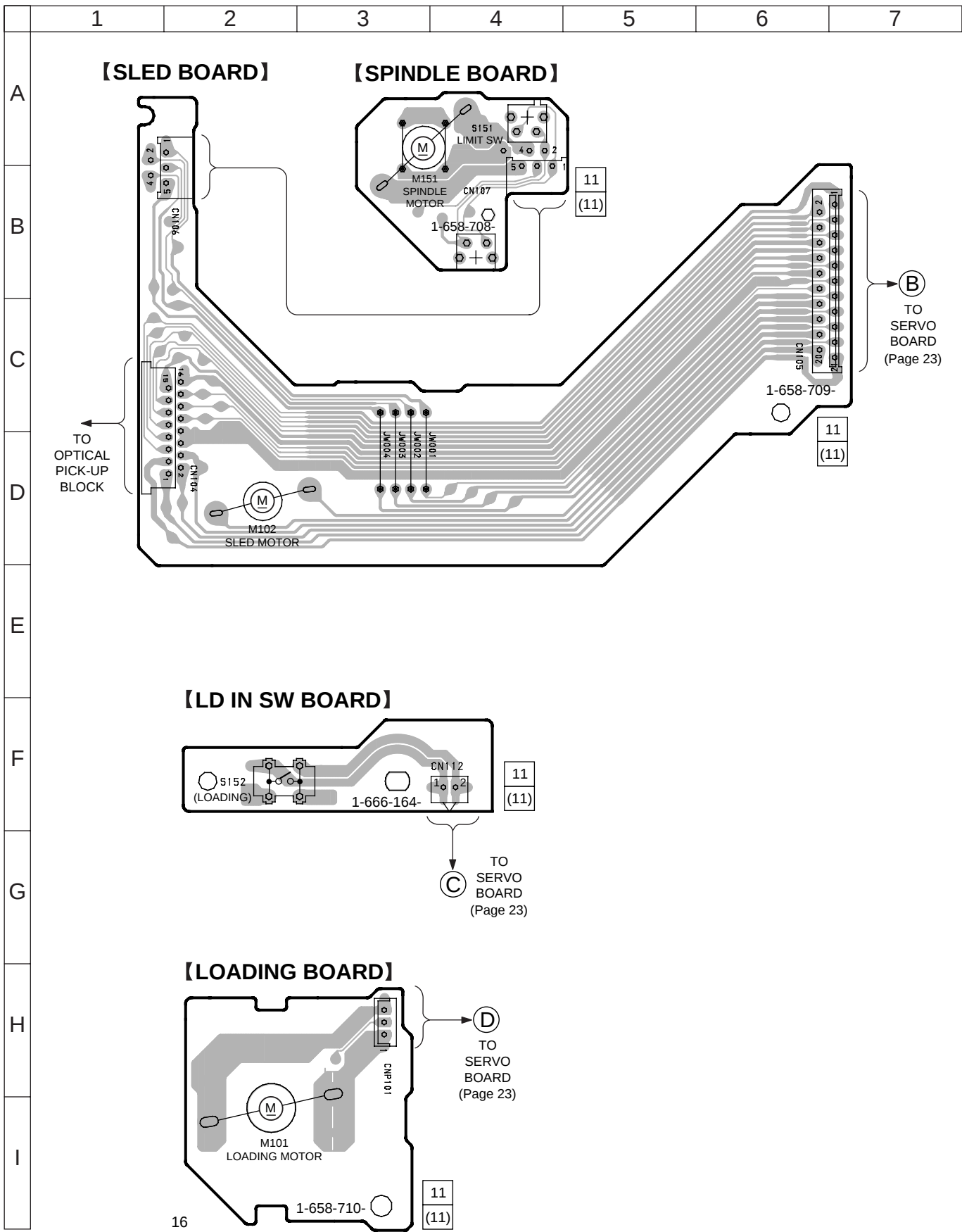
6-13. PRINTED WIRING BOARDS MOTOR SECTION • Refer to page 13 for Circuit Boards Location.
