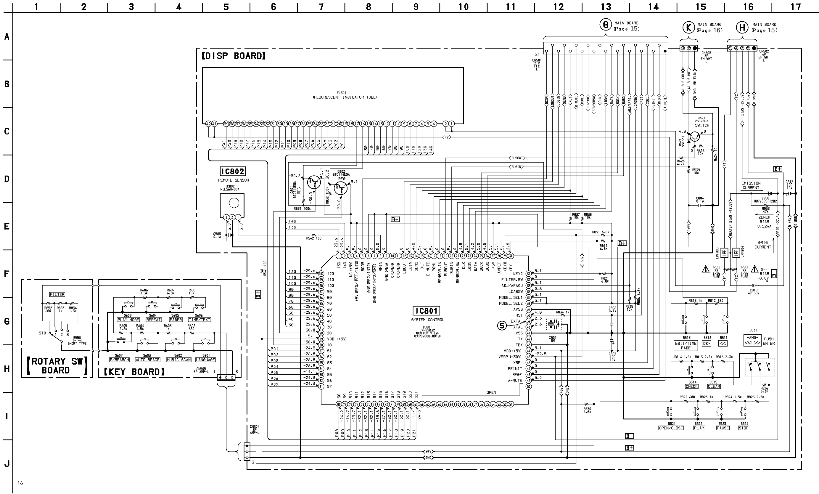
6-6. SCHEMATIC DIAGRAM DISPLAY SECTION • Refer to page 13 for Waveforms. • Refer to page 27 for IC Pin Function Description.
