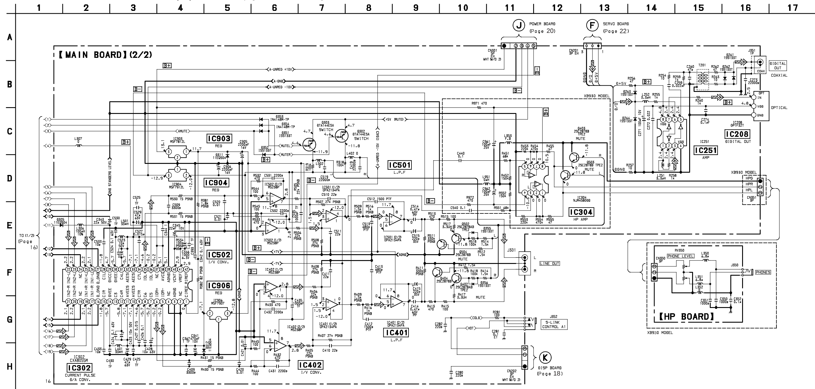
6-4. SCHEMATIC DIAGRAM MAIN SECTION (2/2) • Refer to page 25 for IC Block Diagram.
