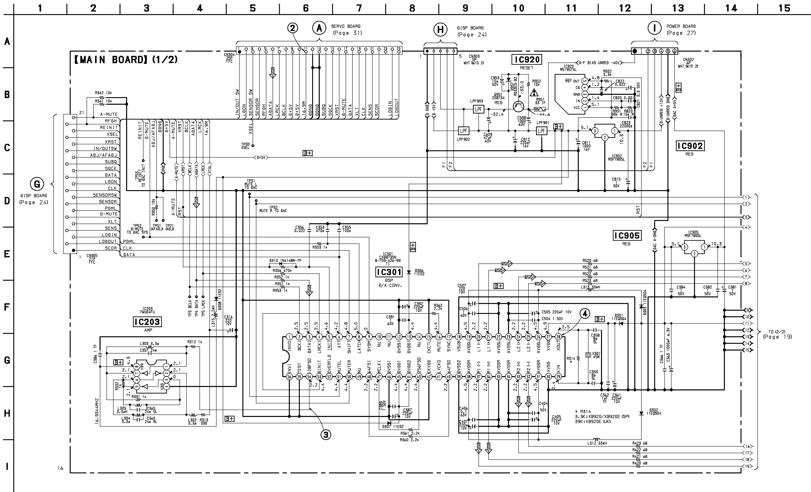
6-3. SCHEMATIC DIAGRAM – MAIN SECTION (1/2) – • See page 37 for IC Block Diagram.
